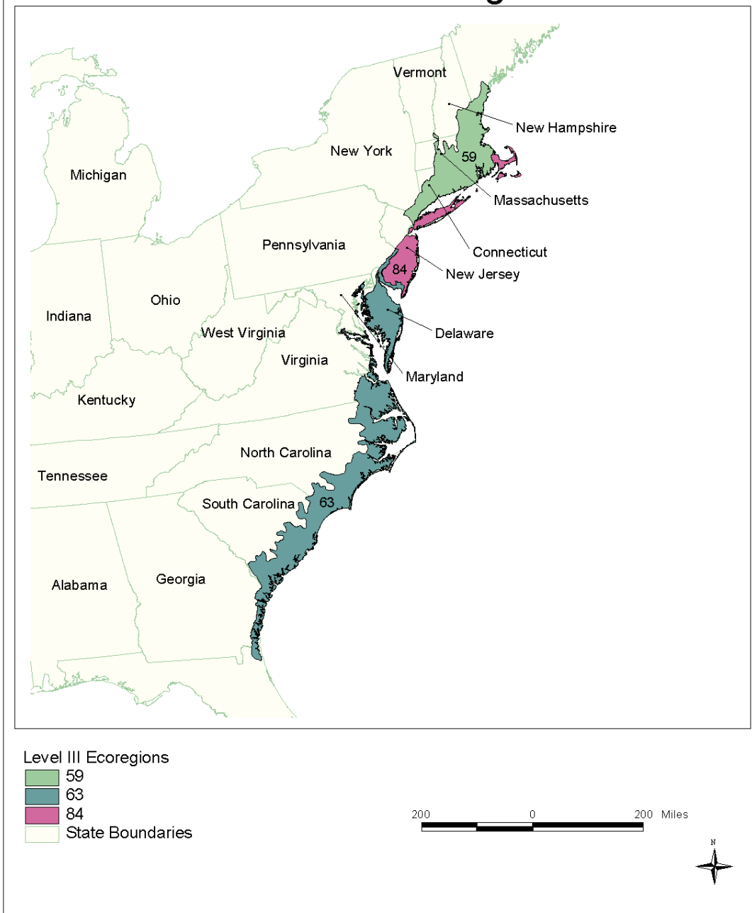
Figure 3. Aggregate Ecoregion XIV with level III Ecoregions shown.
