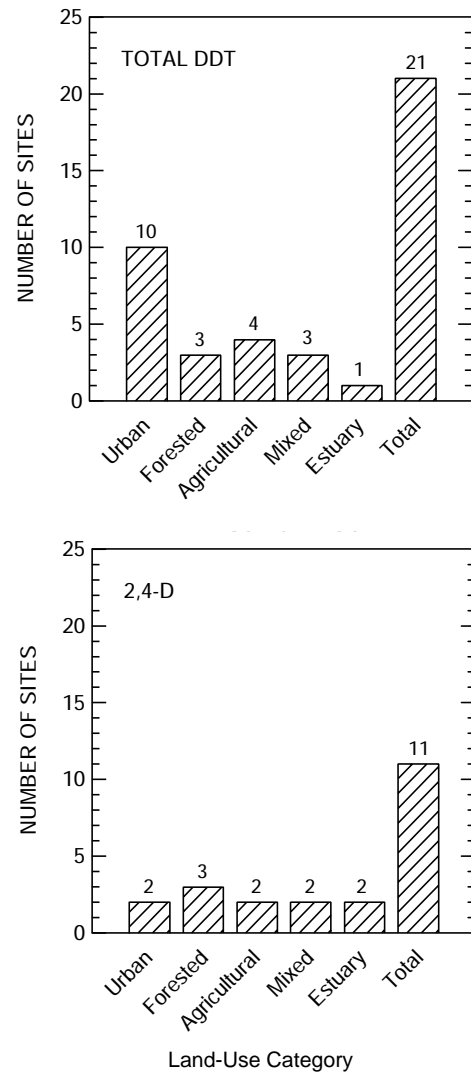
Figure 14. Number of sites in Hudson River basin, N.Y., with concentration data for total DDT or 2,4-D, by land-use category, 1970-90.
