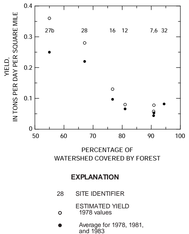
Figure 33. Relation of suspended-sediment yield, 1970-90, to percentage of watershed in the Hudson River basin that is forested. (Site locations are shown in fig. 12.)
