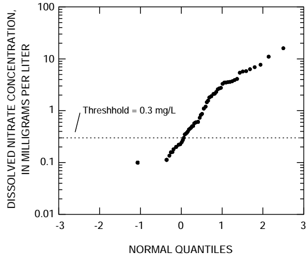
Figure 15. Dissolved nitrate concentrations in water from wells completed in bedrock and unconsolidated aquifers in the Hudson River basin in eastern New York and adjacent States, as a function of normal distribution, 1970-90.
