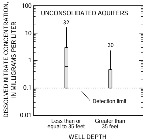
Figure 17. Dissolved nitrate concentrations in relation to well depth in unconsolidated and bedrock aquifers in the Hudson River basin in eastern New York and adjacent States, 1970-90. A. Concentration as a function of well depth. B. Concentration range in shallow and deep wells
