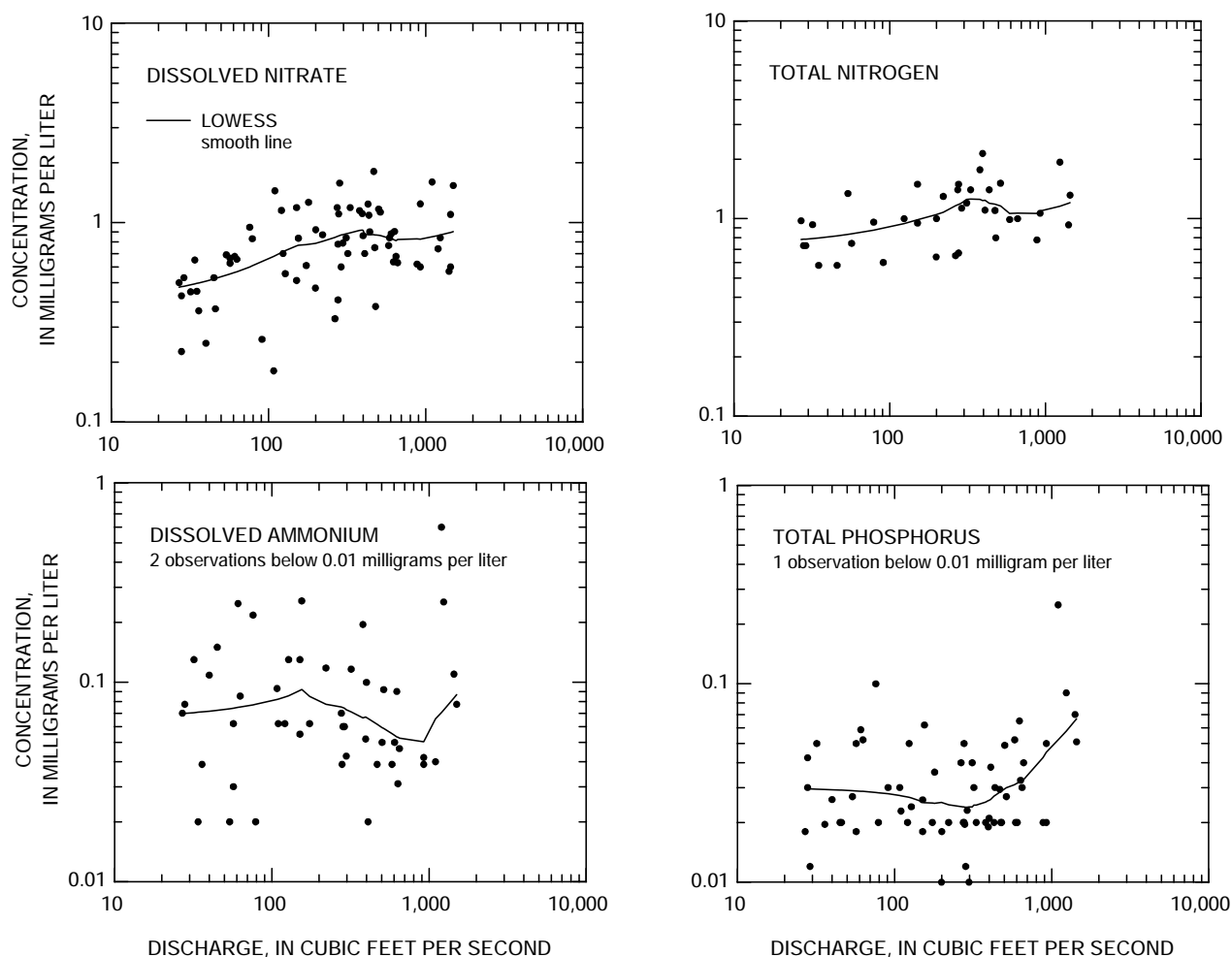
Figure 19A. Nutrient concentrations as a function of discharge in a small agricultural watershed (181 mi 2 , Wappinger Creek near Wappingers Falls, N.Y.), 1970-90.
