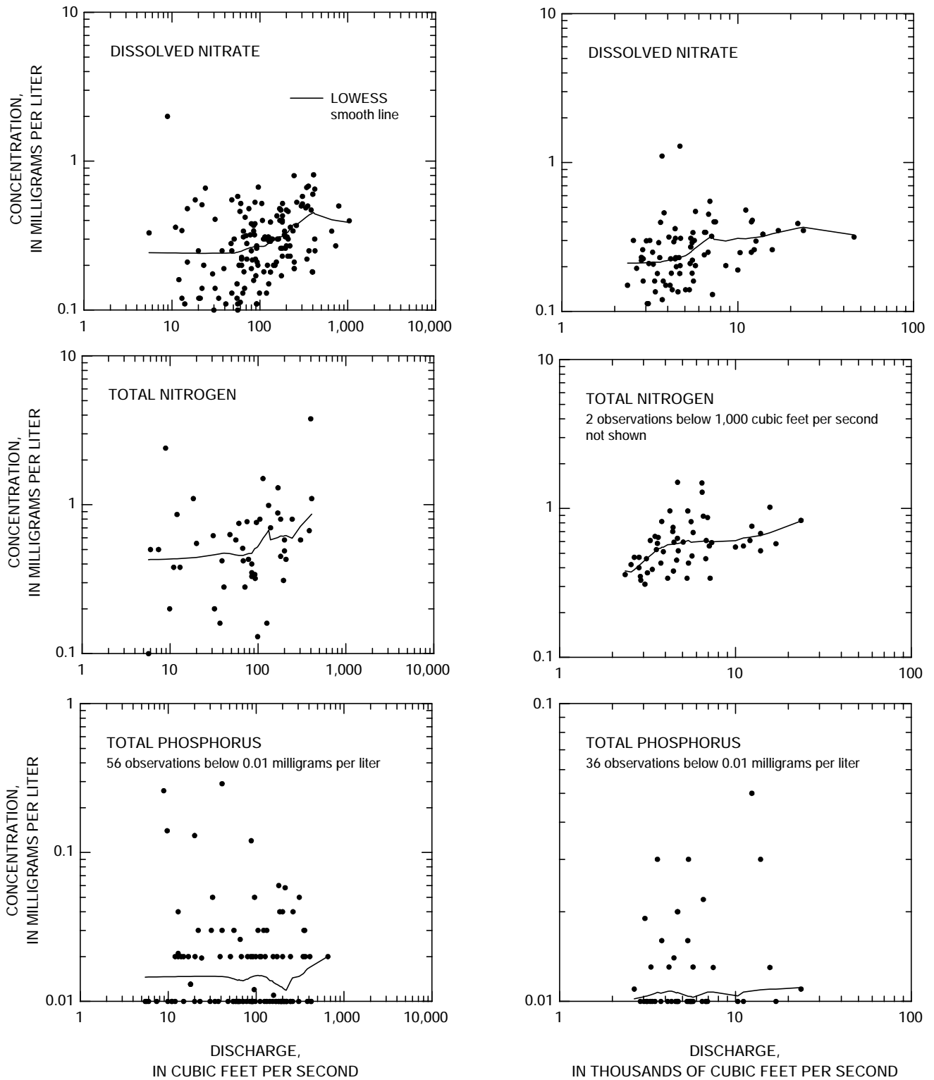
Figure 22. Concentration of dissolved nitrate, total nitrogen, and total phosphorus as a function of discharge at two forested watersheds, 1970-90: A. Esopus Creek at Shandaken, N.Y. (59.5 mi 2 ). B. Hudson River at Corinth, N.Y. (2,755 mi 2 )
