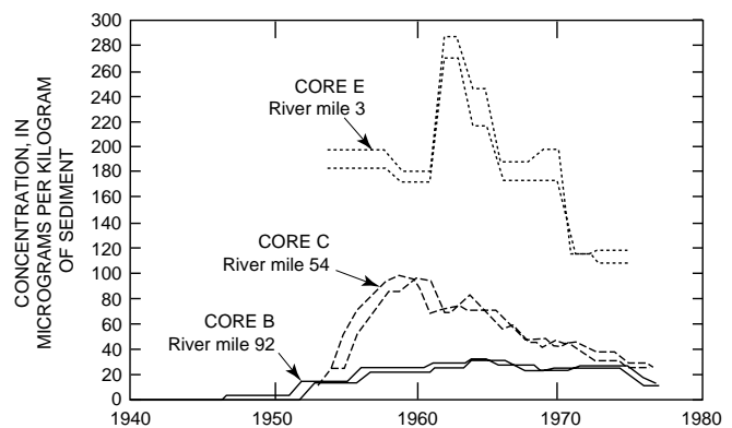
Figure 35. pp'-DDD concentration in Hudson River sediment cores collected by Bopp and others (1982). River miles measured from the southern tip of Manhattan Island. Double lines reflect uncertainty in data. (Modified from Rod, 1989, fig. 8-8).
