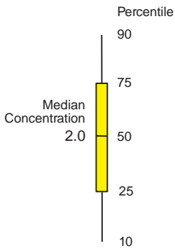
Figure 24. Median and range of dissolved nitrate, total nitrogen, dissolved ammonia, and total phosphorus concentrations at five sites in the Hudson River basin in eastern New York and adjacent States, by land use, 1970-90.
