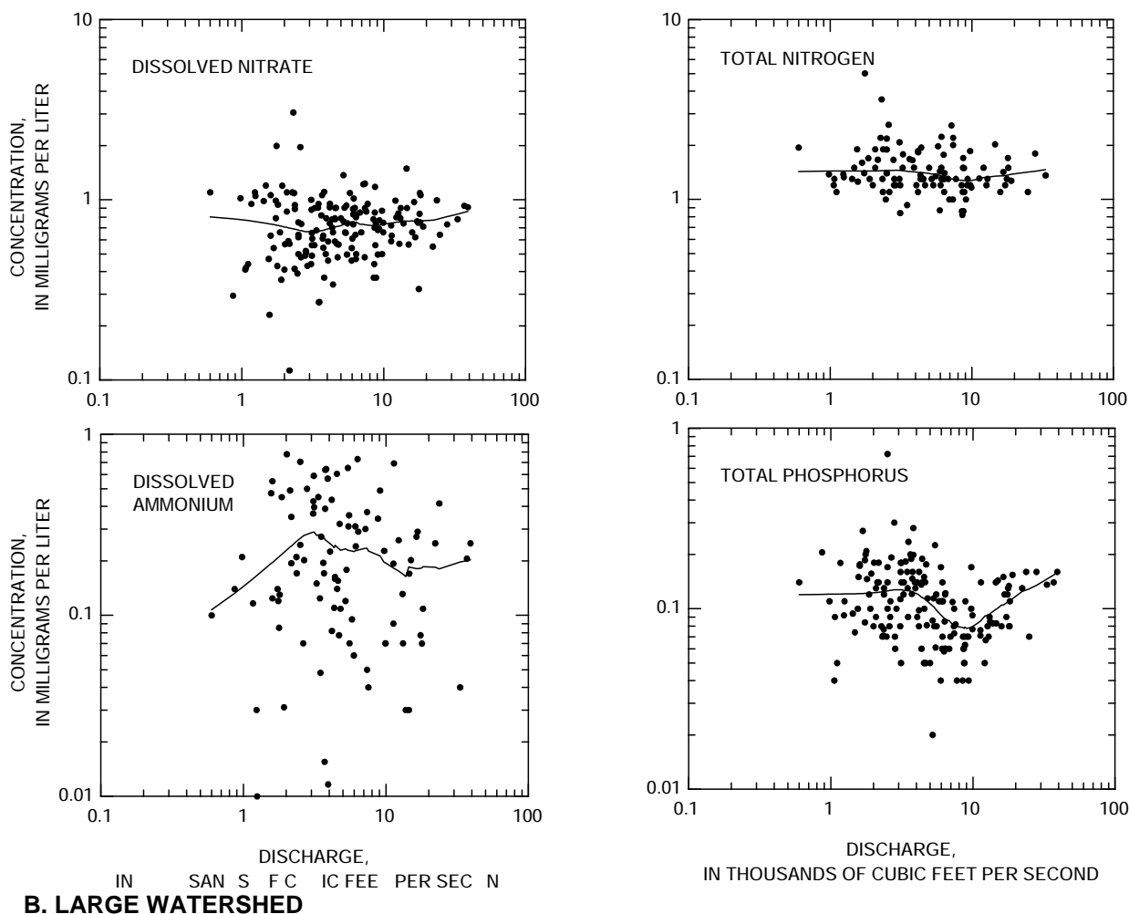
Figure 19B. Nutrient concentrations as a function of discharge in a large agricultural watershed (3,440 mi 2 , Mohawk River at Crescent Dam, N.Y.), 1970-90.
