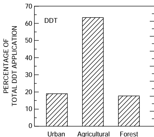
B. DDT, BY LAND USE
