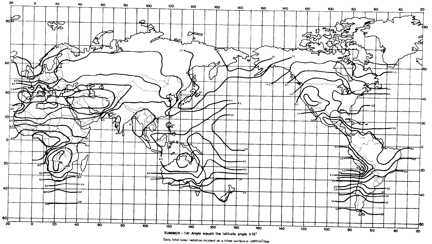
Figure A-3. Insolation Availability (Latitude + 15° Tilt, Summer)
