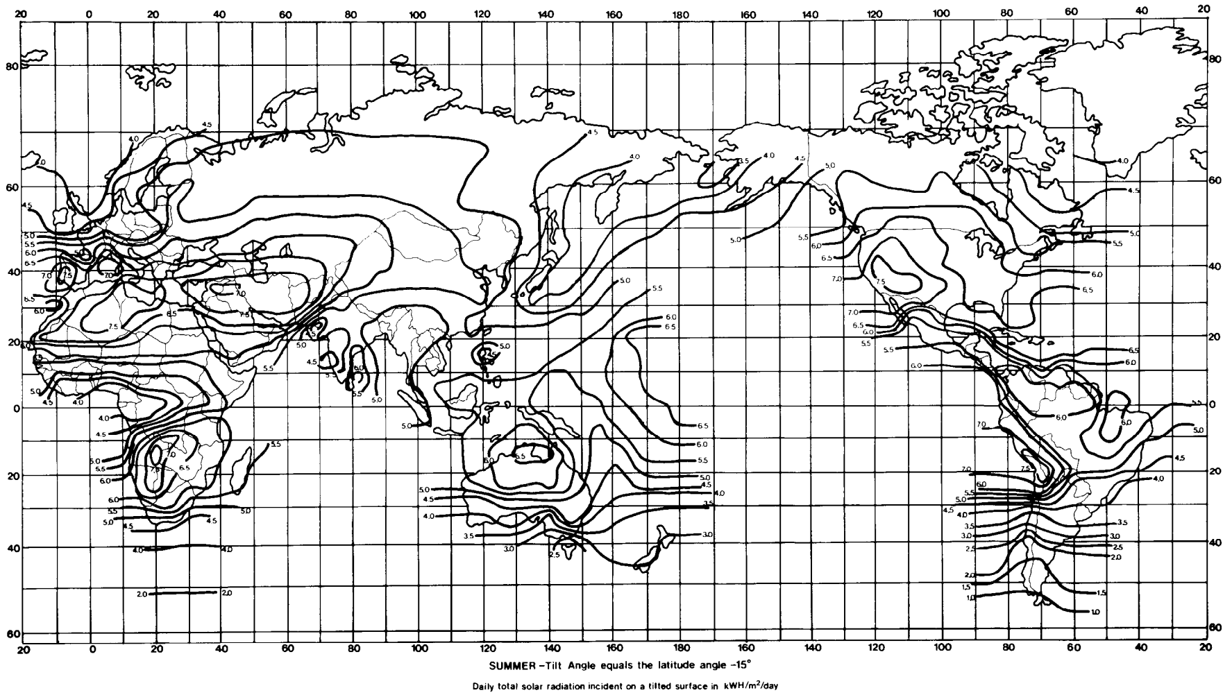
Figure A-11. Insolation Availability (Latitude -15° Tilt, Summer)
