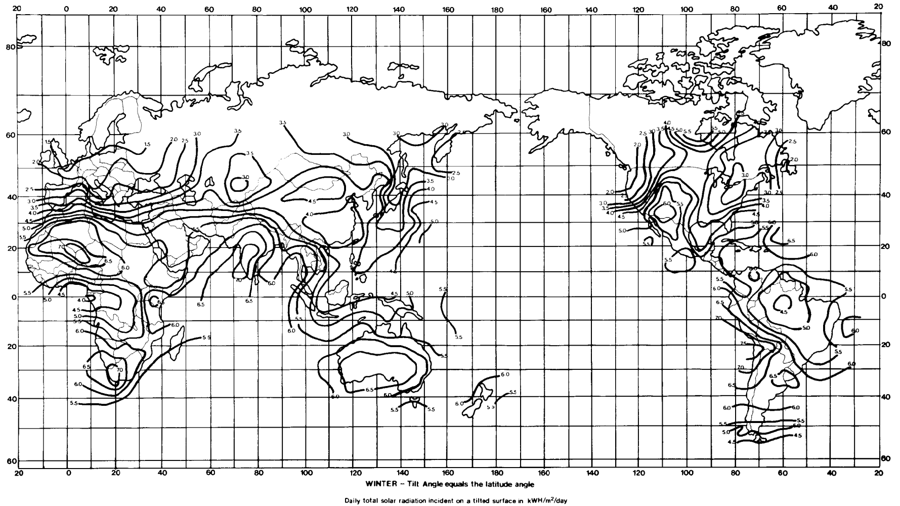
Figure A-5. Insolation Availability (Latitude Tilt, Winter)
