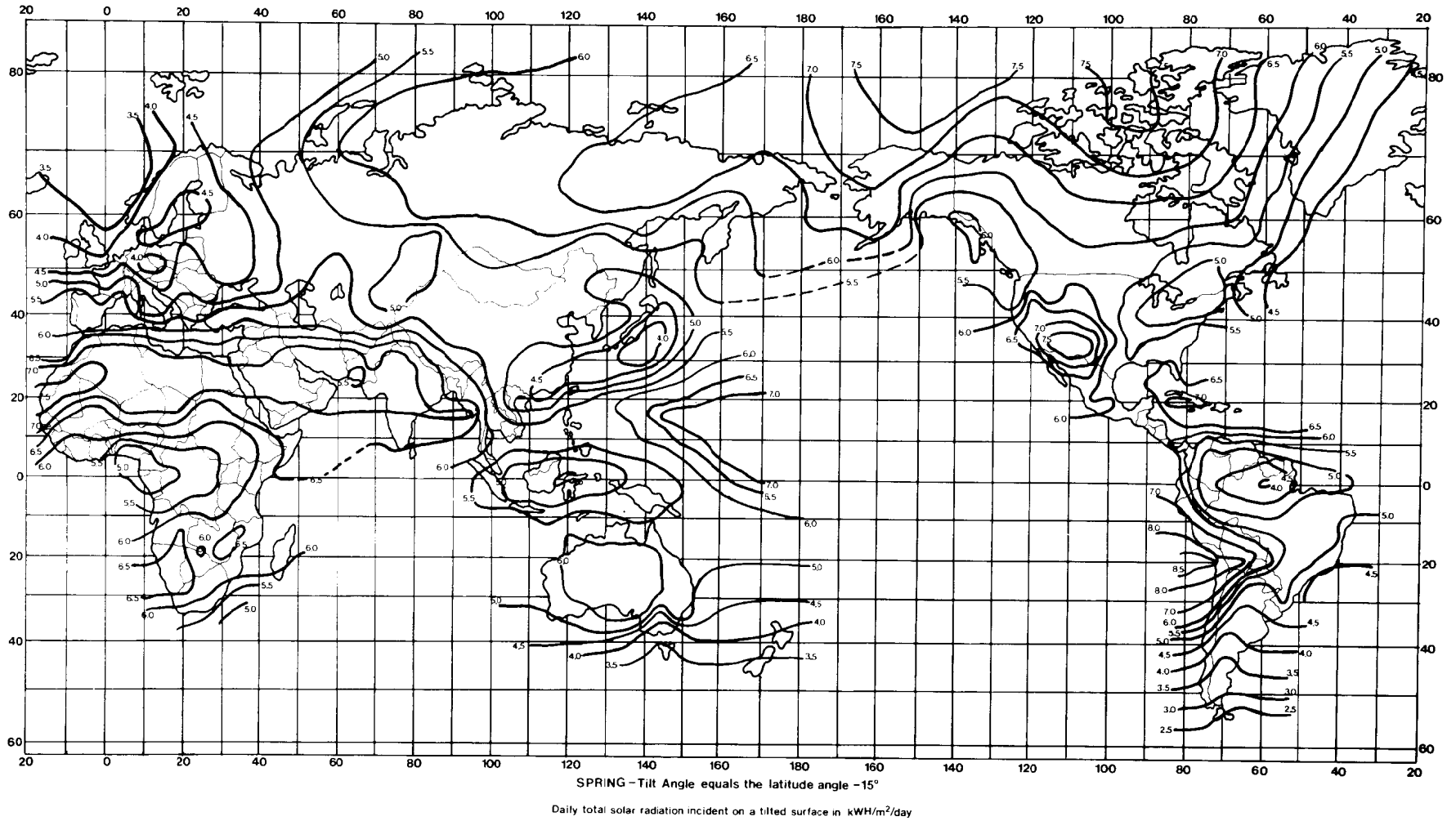
Figure A-10. Insolation Availability (Latitude - 15° Tilt, Spring)
