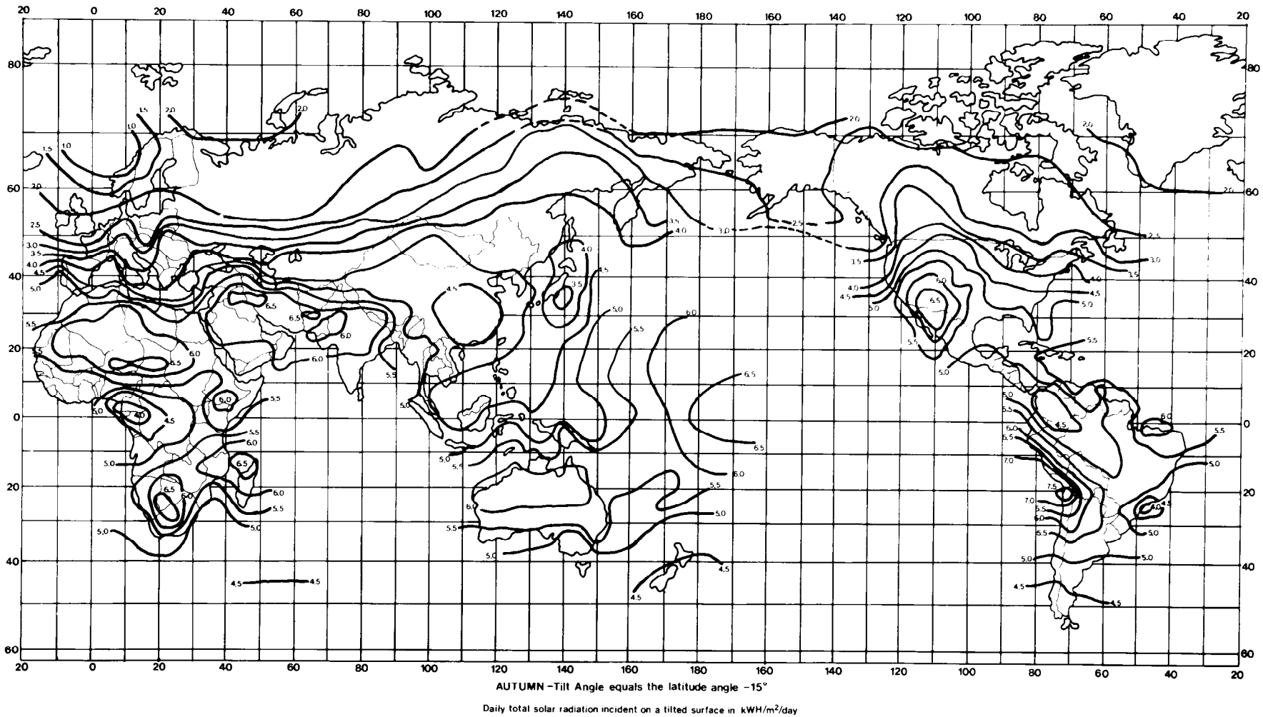
Figure A-12. Insolation Availability (Latitude +15° Tilt, Autumn)
