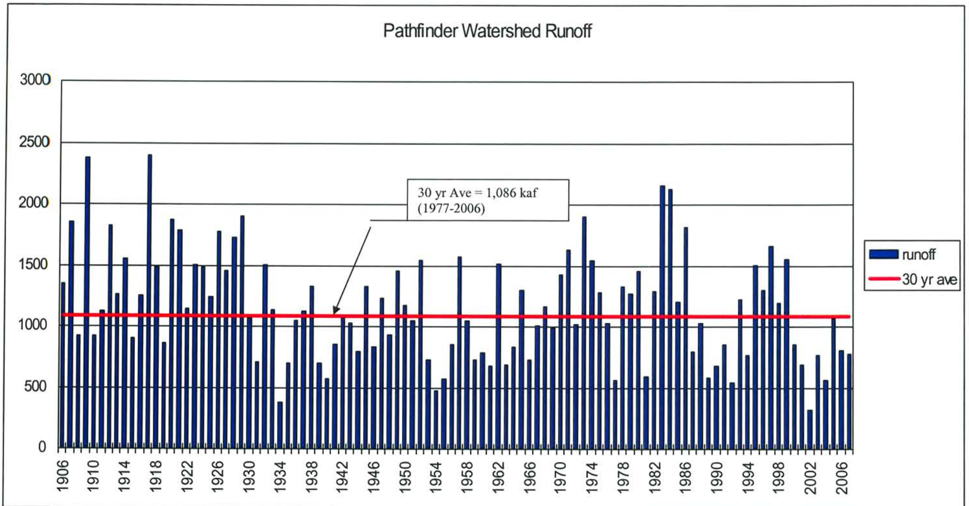
Figure 20 Pathfinder Watershed Runoff 1906-2007
