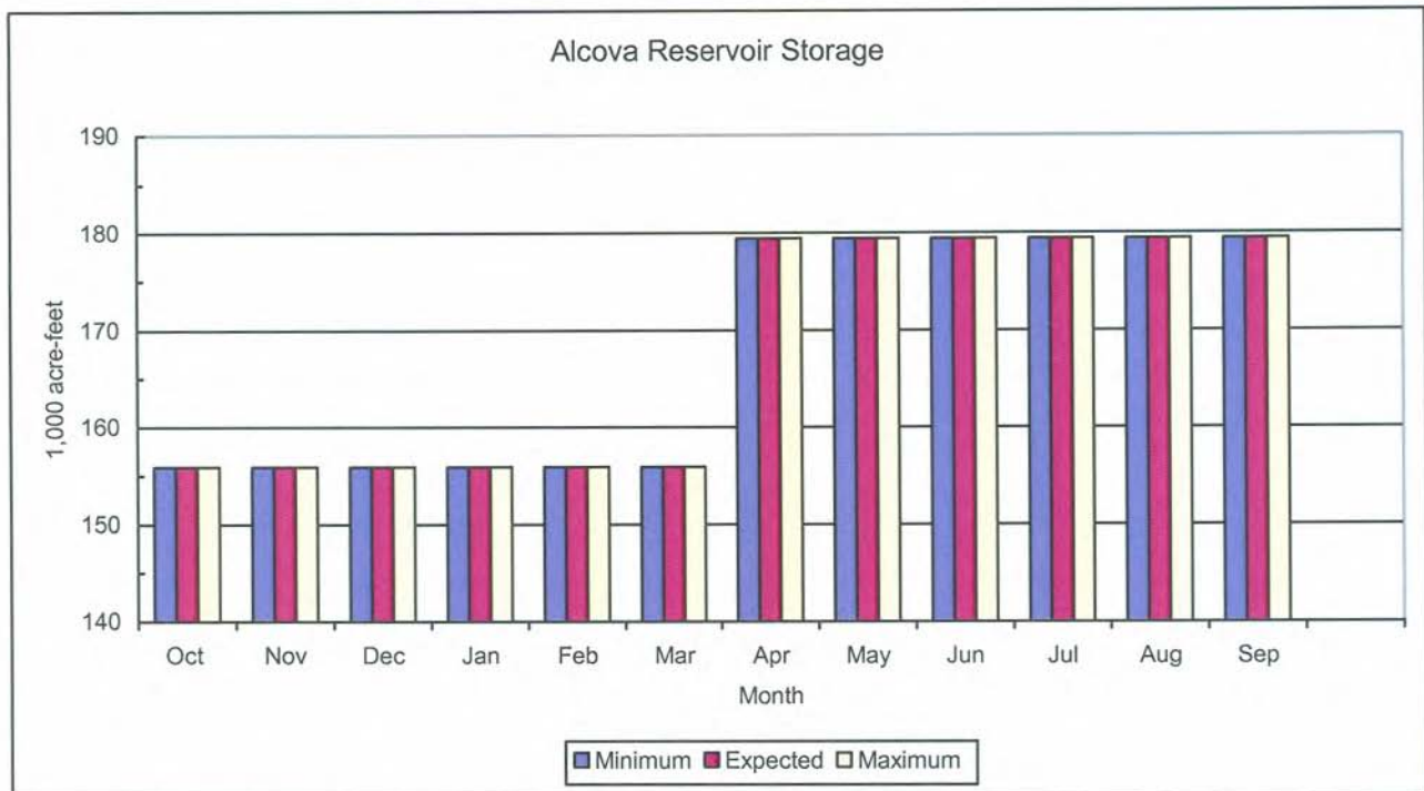
Figure 16 Alcova Reservoir Storage (predicted for water year 2008)
