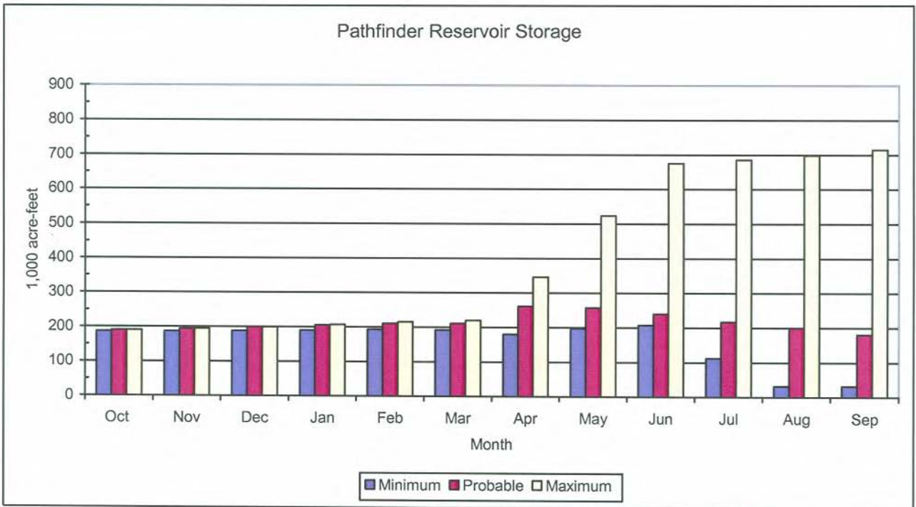
Figure 15 Pathfinder Reservoir Storage (predicted for water year 2008)
