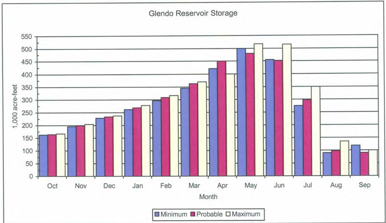
Figure 18 Glendo Reservoir Storage (predicted for water year 2008)
