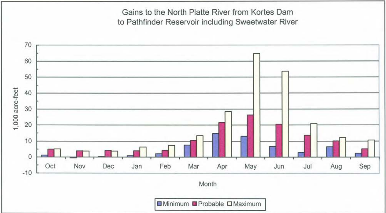
Figure 14 Gains to the North Platte River from Kortes Dam to Pathfinder Reservoir (predicted for water year 2008)
