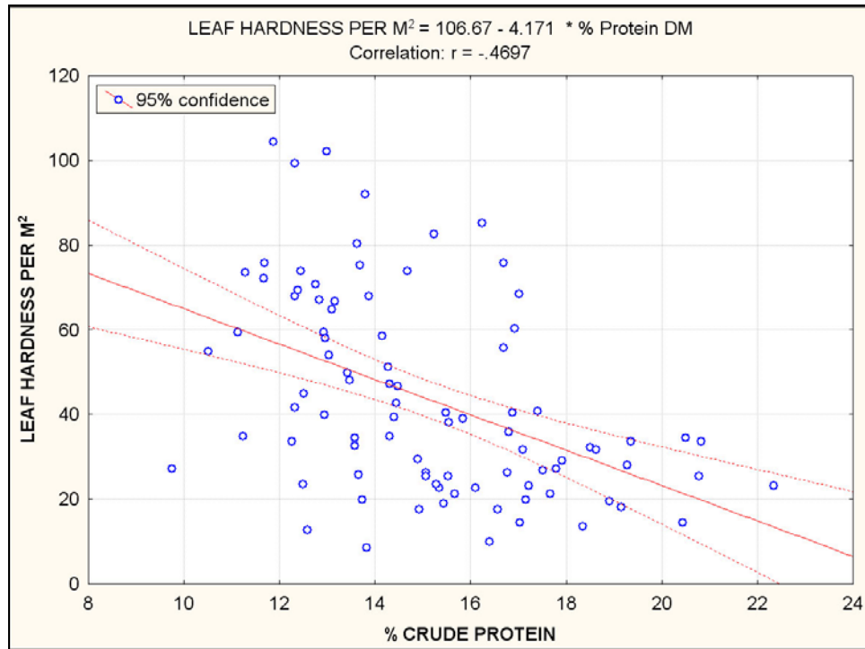
Figure 10. Linear relationship between leaf hardness and % protein (dry matter basis) for sites sampled on Lake Seminole during 2000 ( p < 0.05 , n = 90 , r = -0.4697 )
