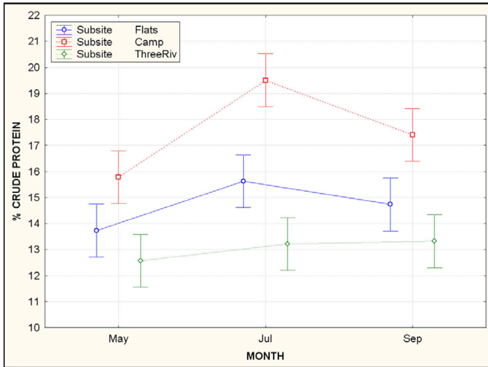
Figure 12. Percentage crude protein for all Lake Seminole sites sampled in 2000. Bars surrounding the means are the 95% confidence interval based on the ANOVA error terms. ANOVA results include: Site – F = 60.33 , df = 2, 81 , p < 0.0000 ; Month – F = 12.50 , df = 2, 81 , p = 0.0000 ; Site by Month interaction – F = 2.44 , df = 4, 81 , p = 0.054
