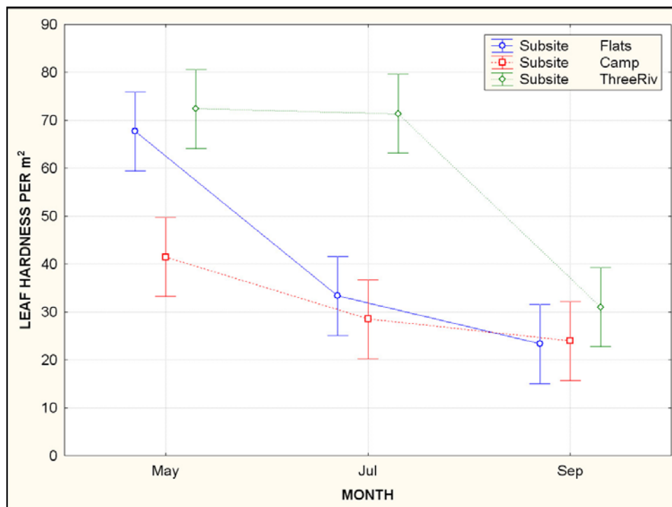
Figure 9. Leaf hardness for Lake Seminole sites sampled in 2000. Bars surrounding means are 95% confidence intervals based on ANOVA error terms. ANOVA results for leaf hardness include: Site – F = 32.22, df = 2, 81, p < 0.0000; Month – F = 51.69, df = 2, 81, p < 0.0000; Site by Month interaction – F = 8.45, df = 4, 81, p < 0.0000
