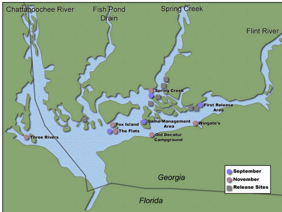
Figure 1. Map of Lake Seminole with areas sampled in September 1999 and November 1999 and original release areas for H. pakistanae
