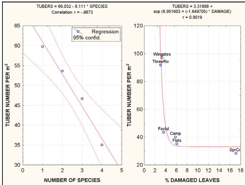
Figure 5. Comparisons between tuber numbers per m 2 and number of plant species and percentage damaged leaves for sites sampled in September 1999
