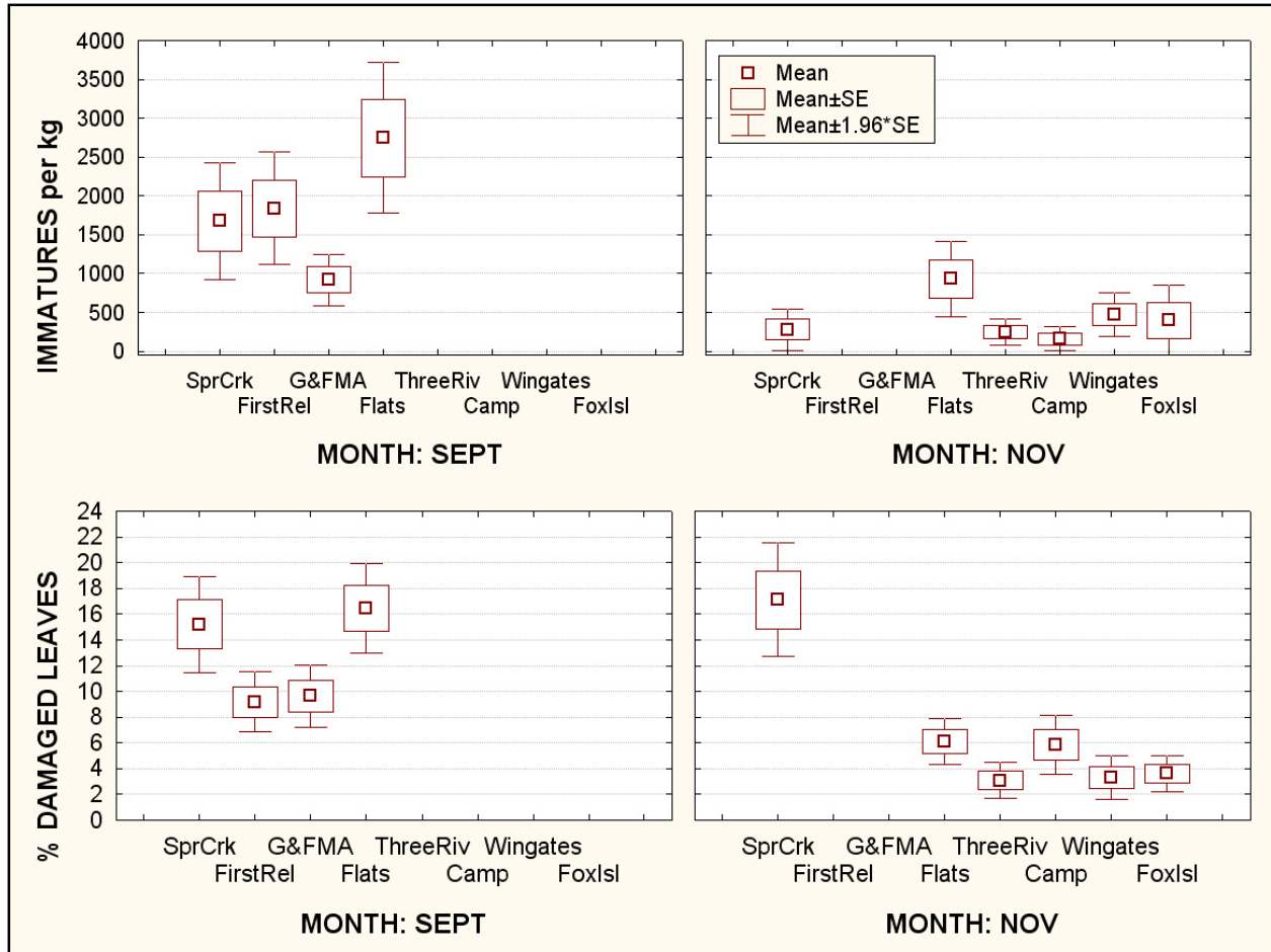
Figure 3. Mean number of immatures per kg of wet plant material and associated percent leaf damage for sites sampled on Lake Seminole during September 1999 and November 1999
