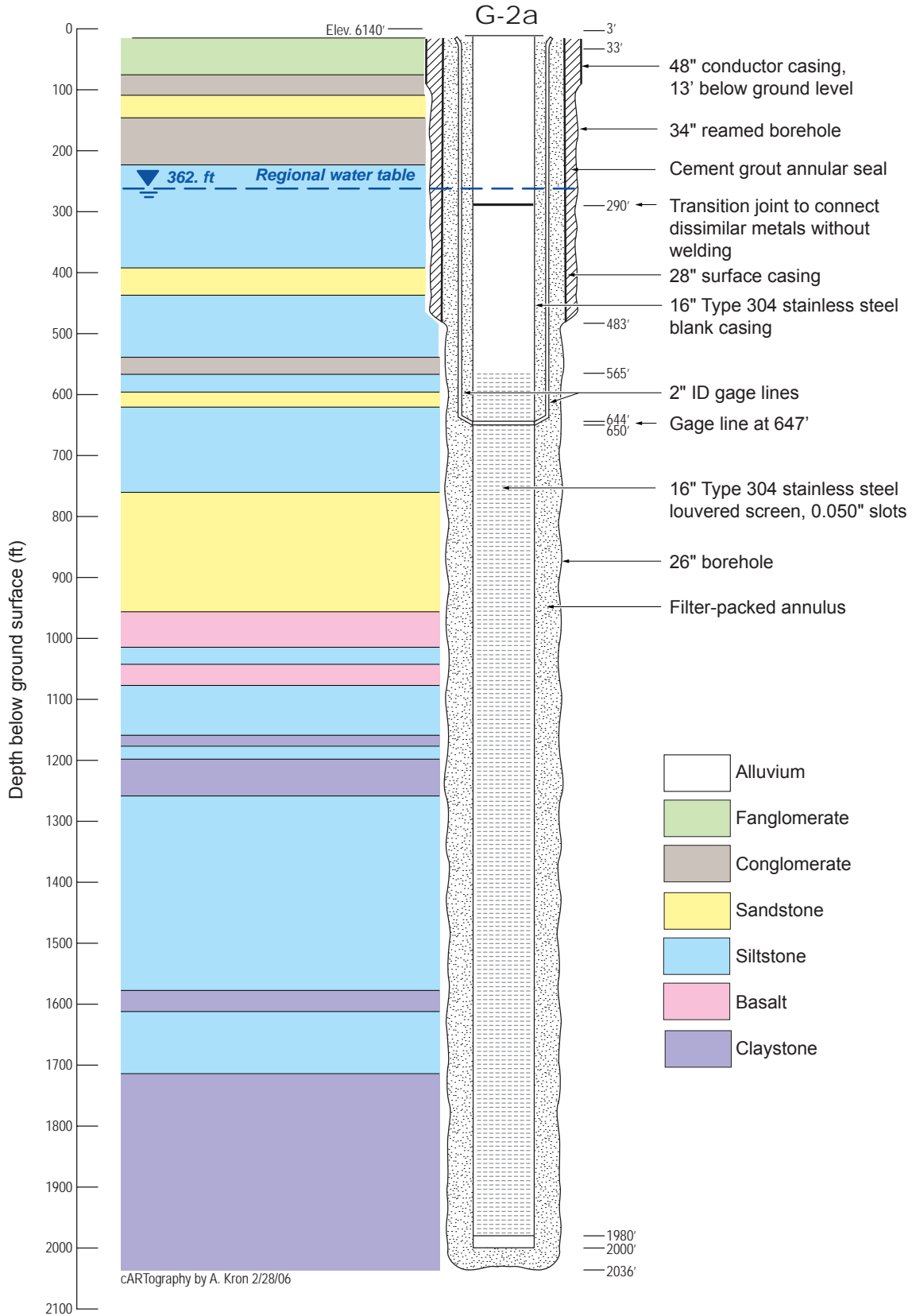
Figure E-16.9. Completion diagram and stratigraphy of well G-2A
