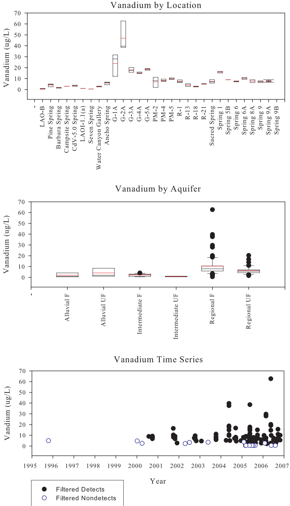
Figure C-49. Vanadium
