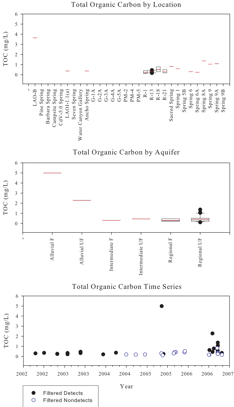
Figure C-16. Total Organic Carbon
