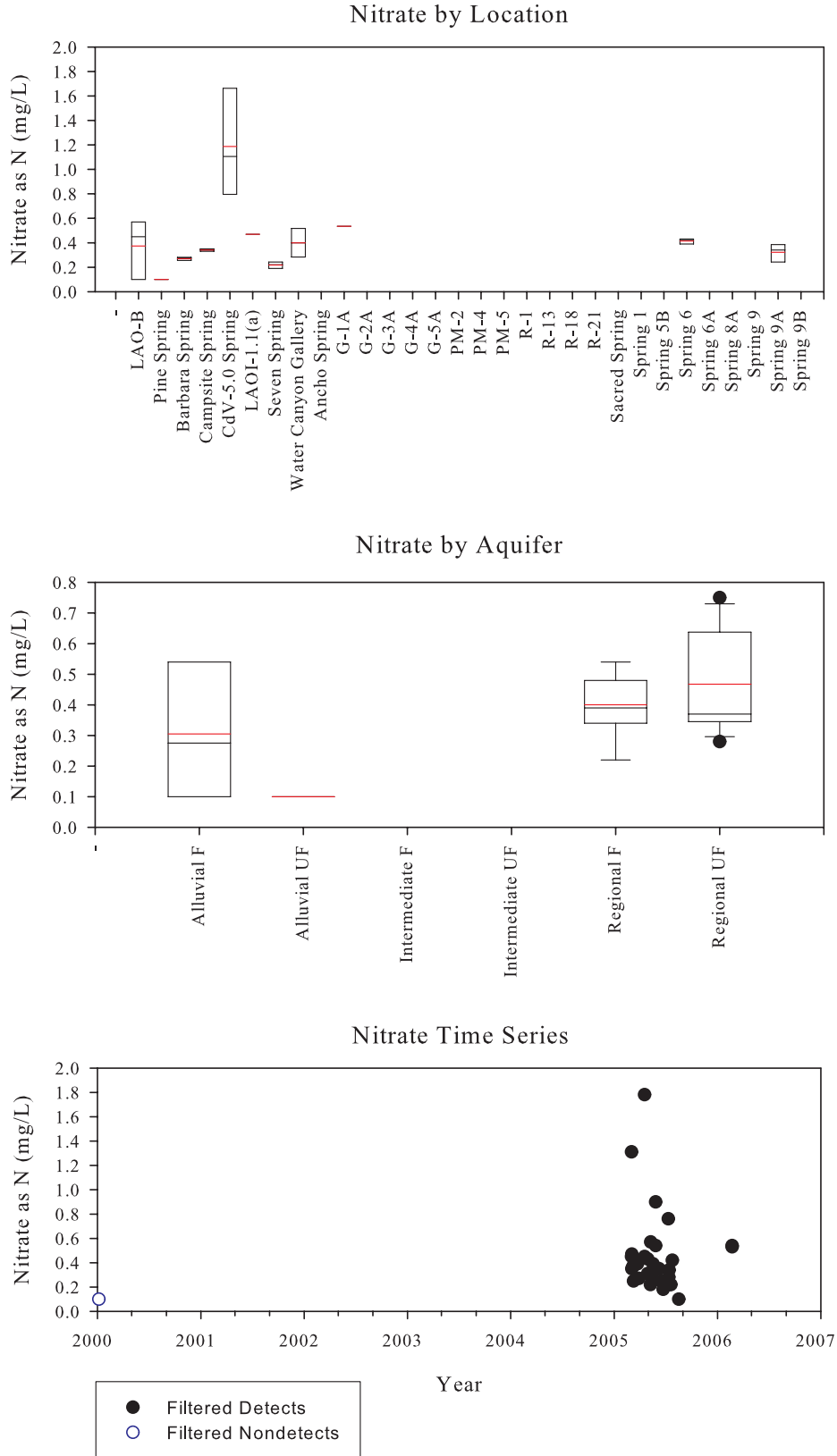
Figure C-8. Nitrate
