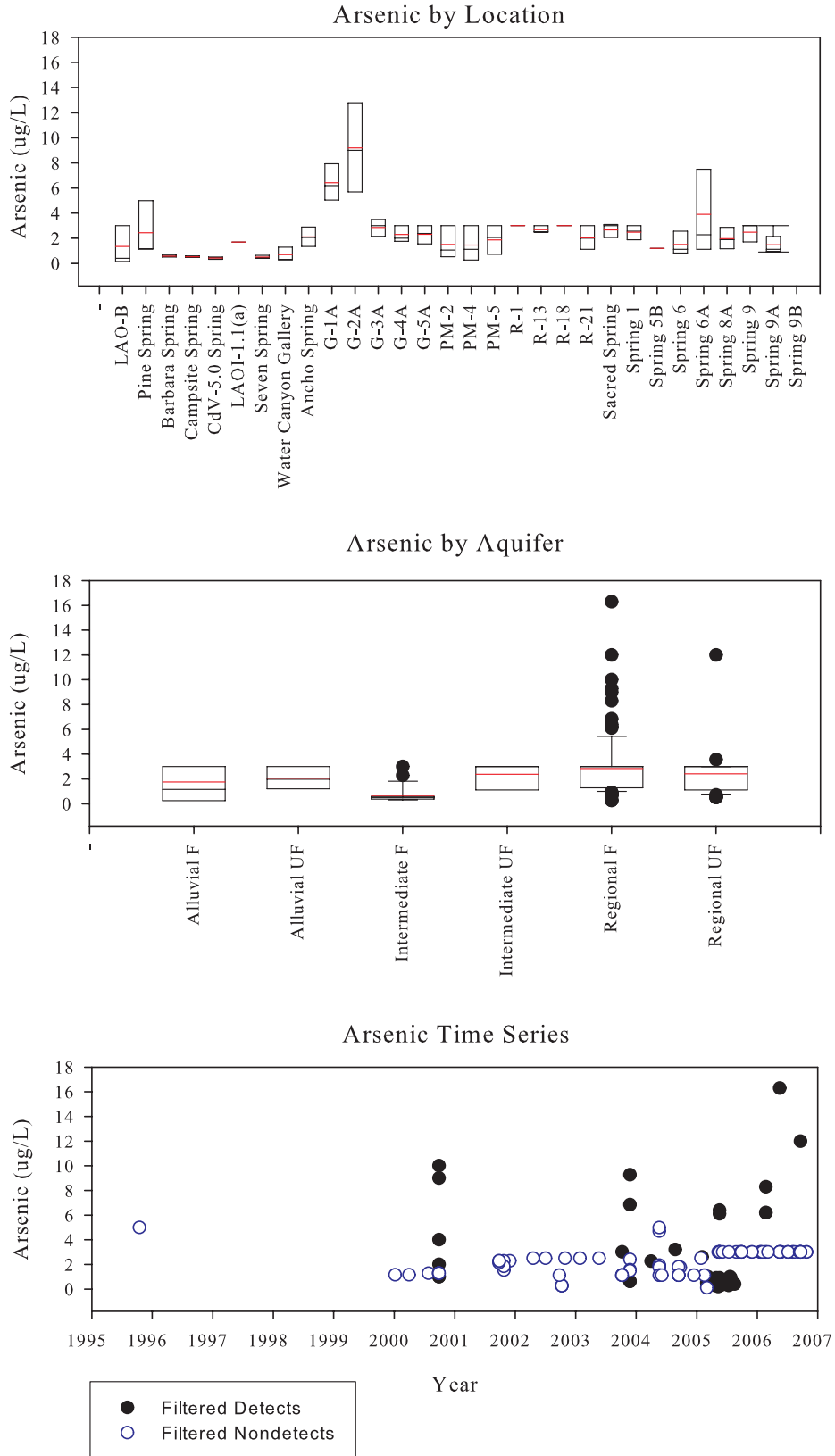
Figure C-23. Arsenic
