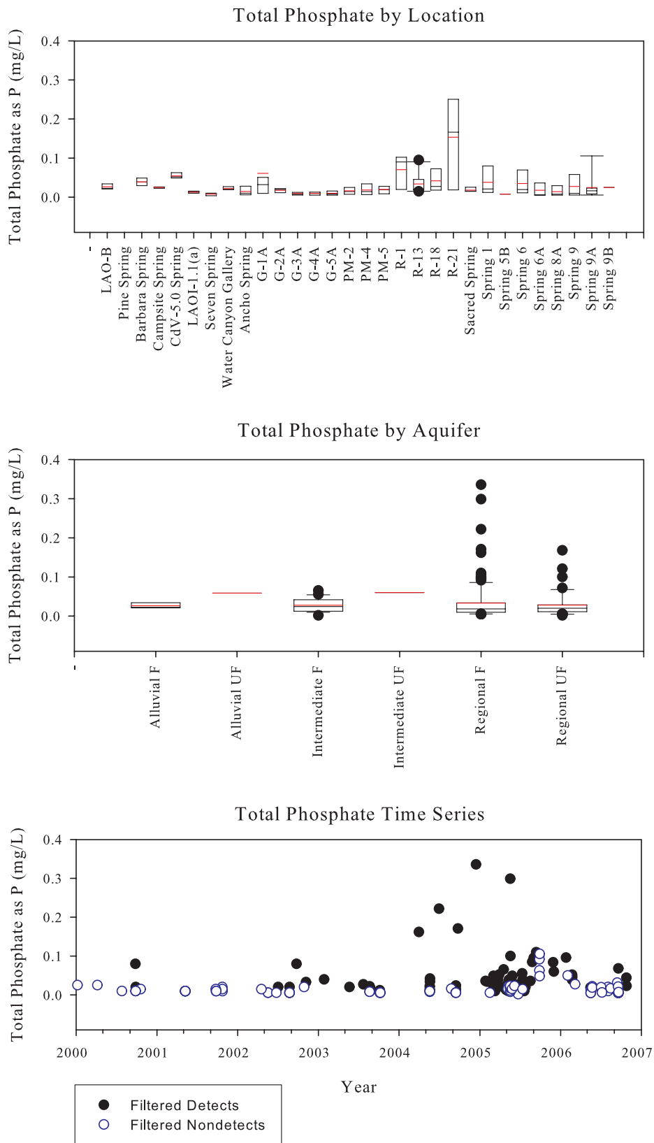
Figure C-17. Total Phosphate as Phosphorus
