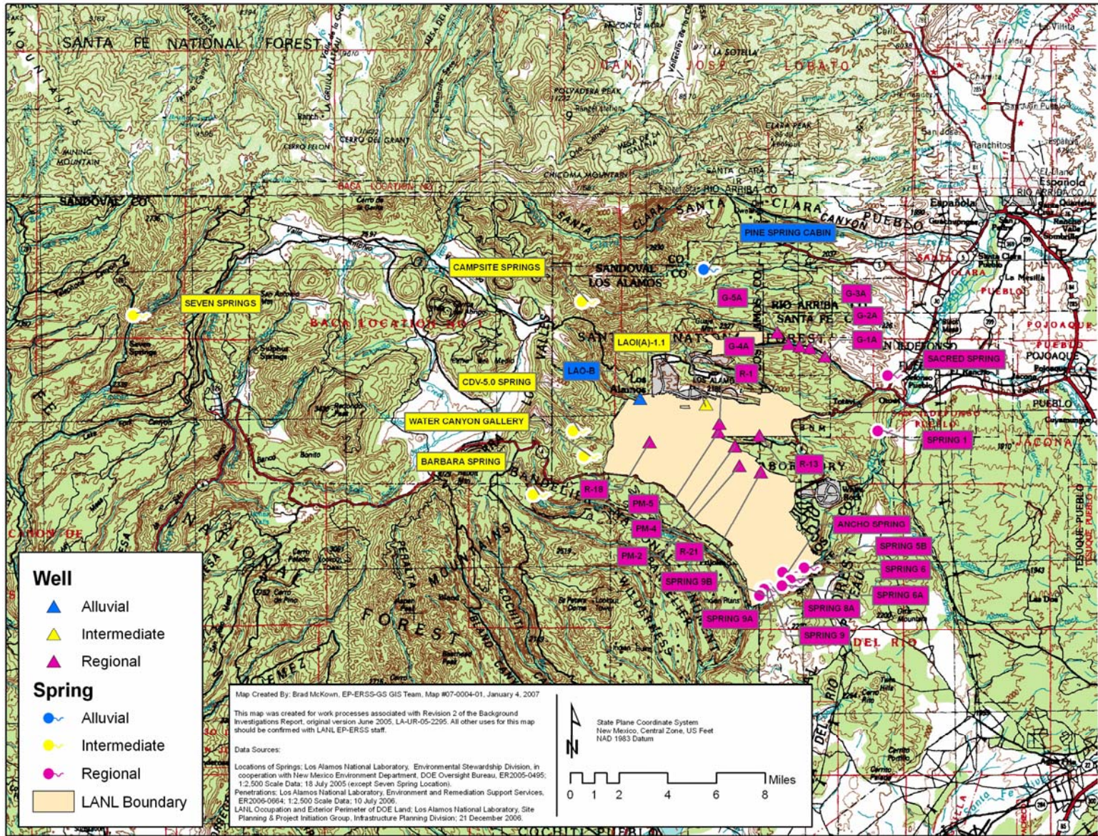
Figure 1.2-1. Location of 30 groundwater background sites in the Jemez Mountains and near Los Alamos National Laboratory, New Mexico
