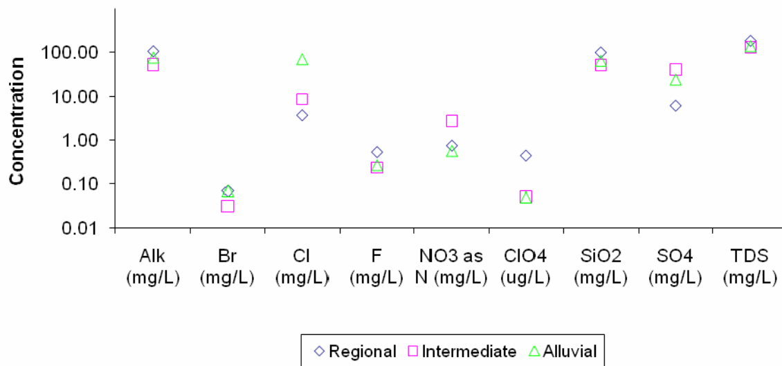
Figure ES-1a. Screening values for selected major chemical constituents for regional, perched intermediate, and alluvial groundwaters
