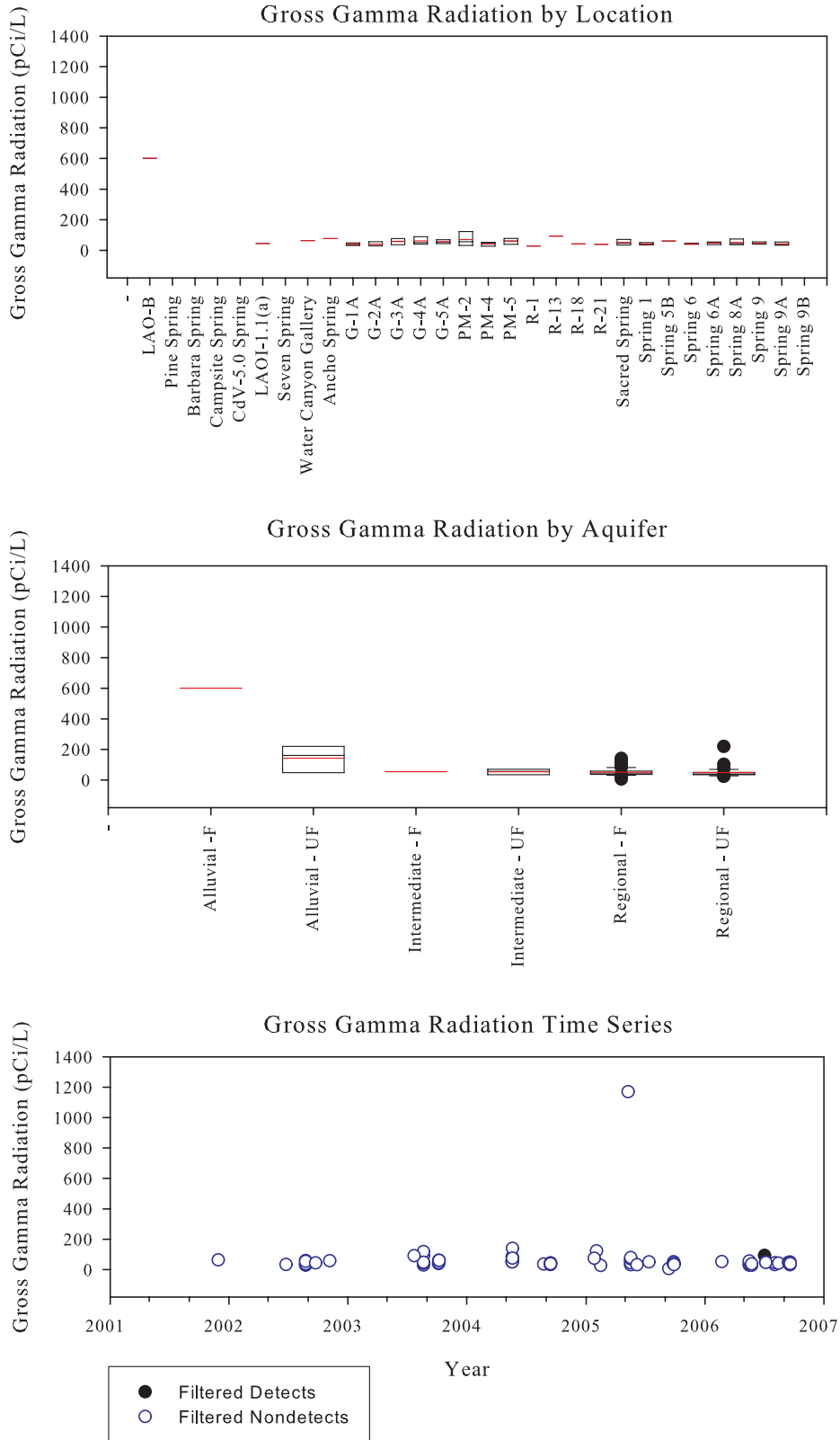
Figure C-56. Gross Gamma
