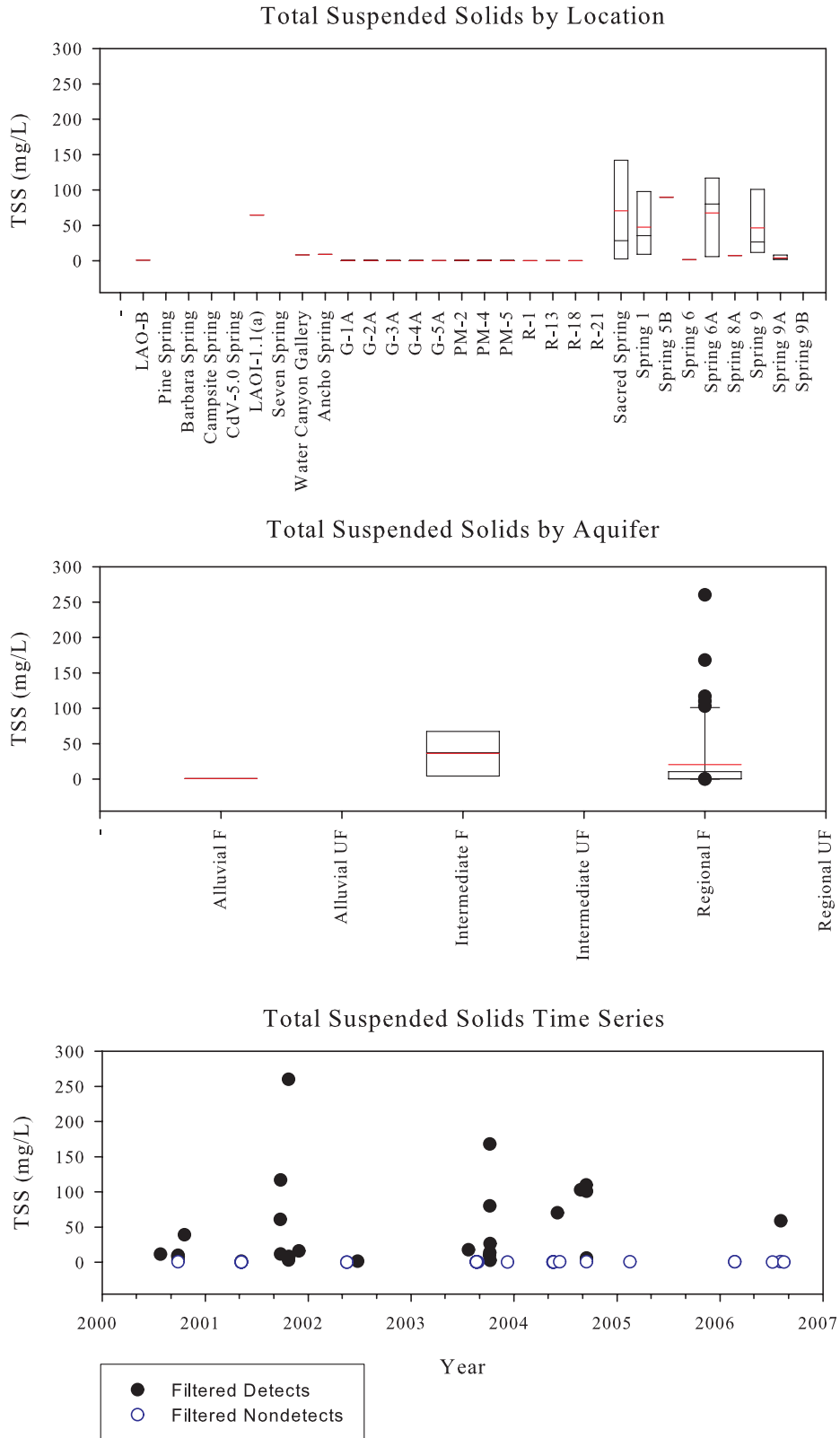
Figure C-18. Total Suspended Solids
