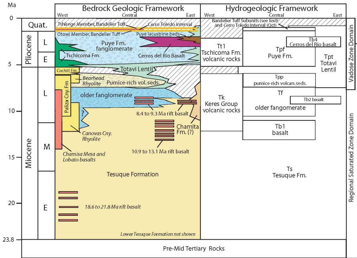
Figure 2.1-4. Revised stratigraphy of the Pajarito Plateau (Broxton and Vaniman 2005, 088707)
