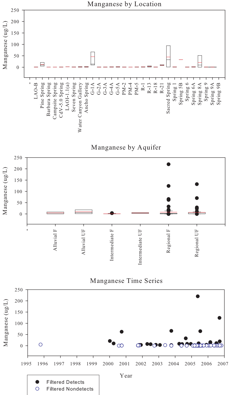
Figure C-36. Manganese
