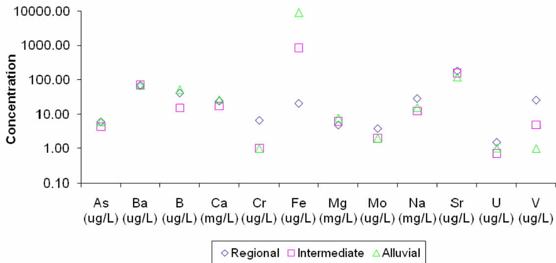
Figure ES-1b. Screening values for selected metals for regional, perched intermediate, and alluvial groundwaters
