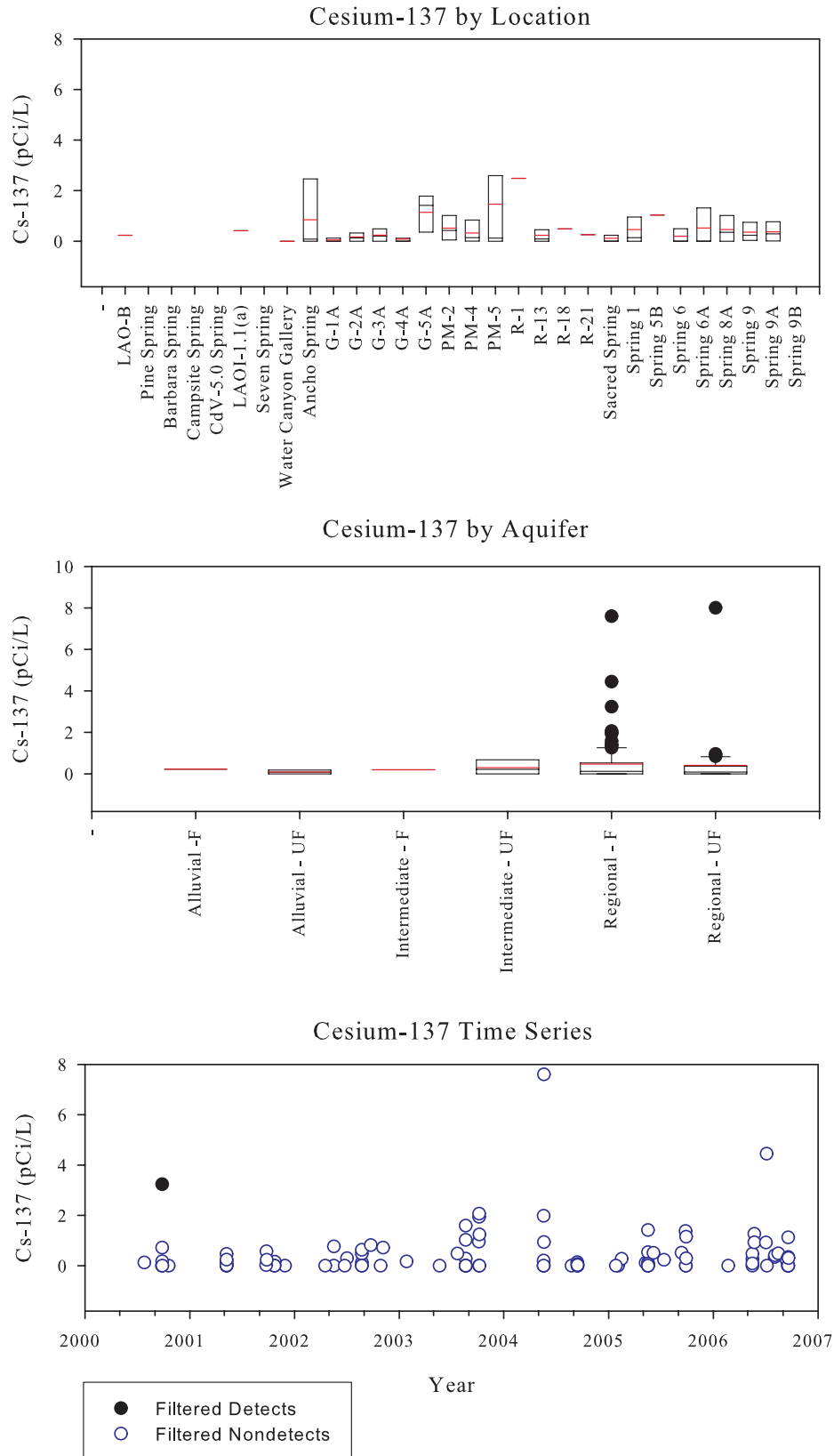
Figure C-53. Cesium-137
