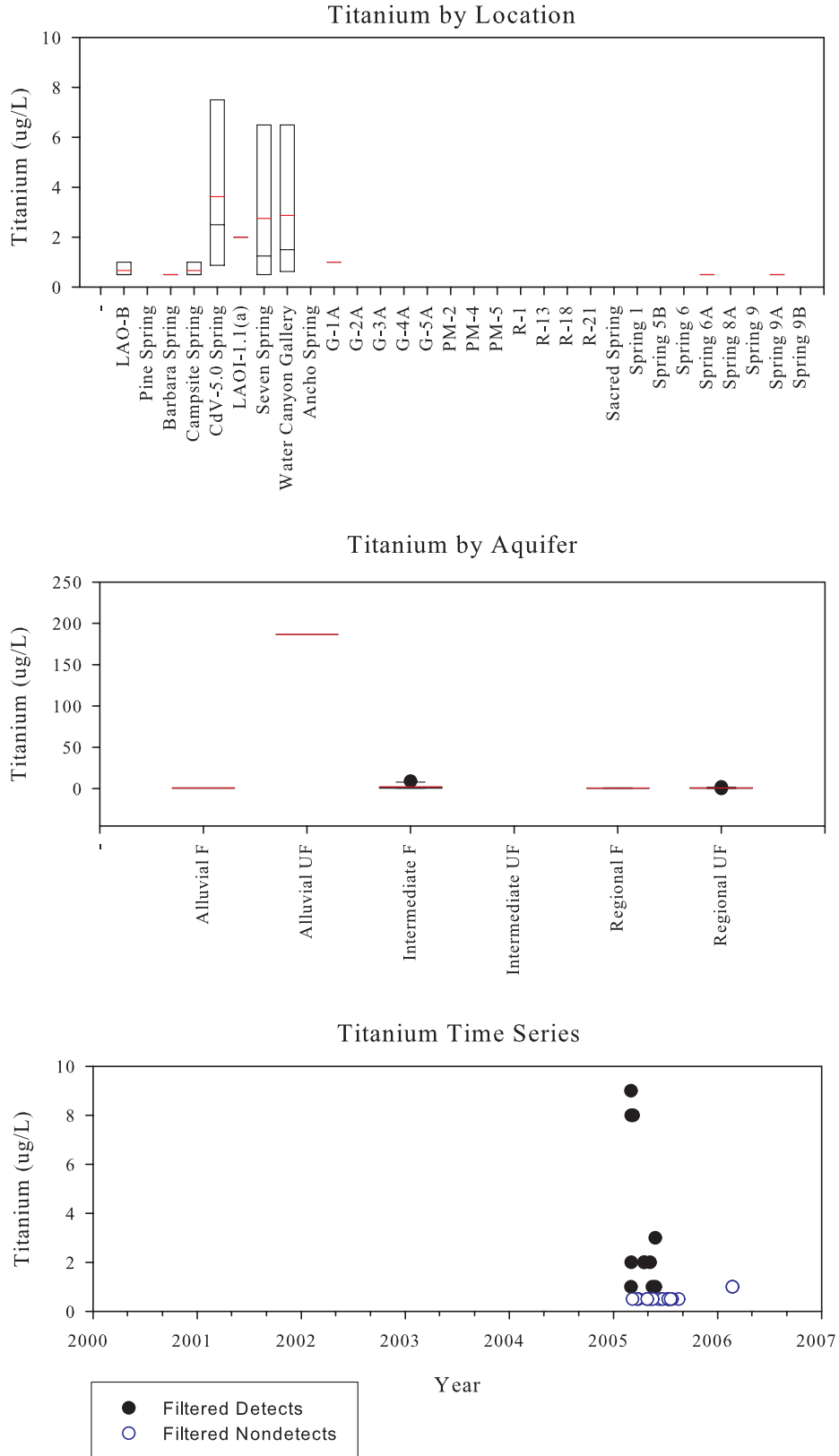
Figure C-47. Titanium
