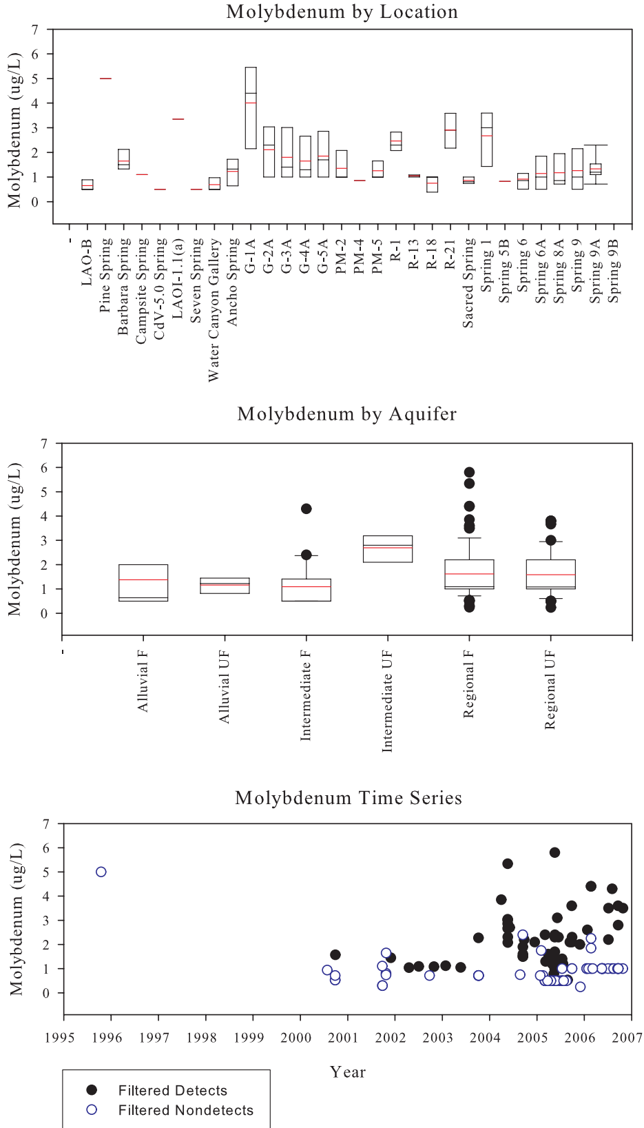
Figure C-38. Molybdenum
