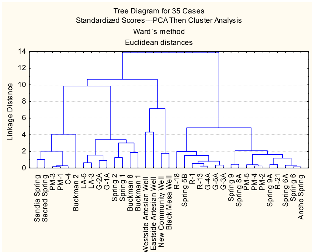
Figure 4.5-1. Groundwater groupings determined by PCA and CA
