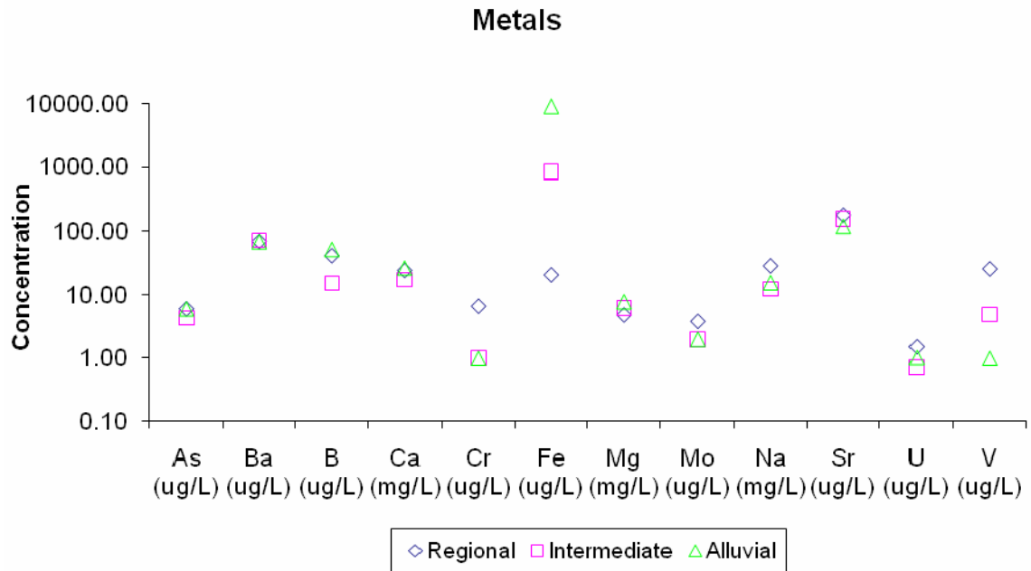
Figure 4.3-1b. Screening values for selected metals for regional, perched intermediate, and alluvial groundwaters
