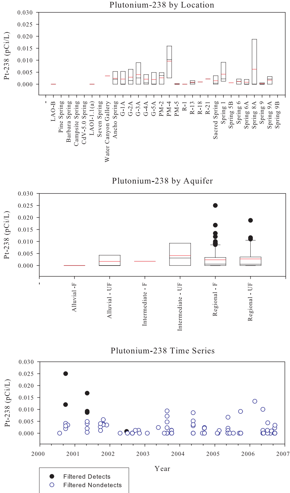
Figure C-57. Plutonium-238
