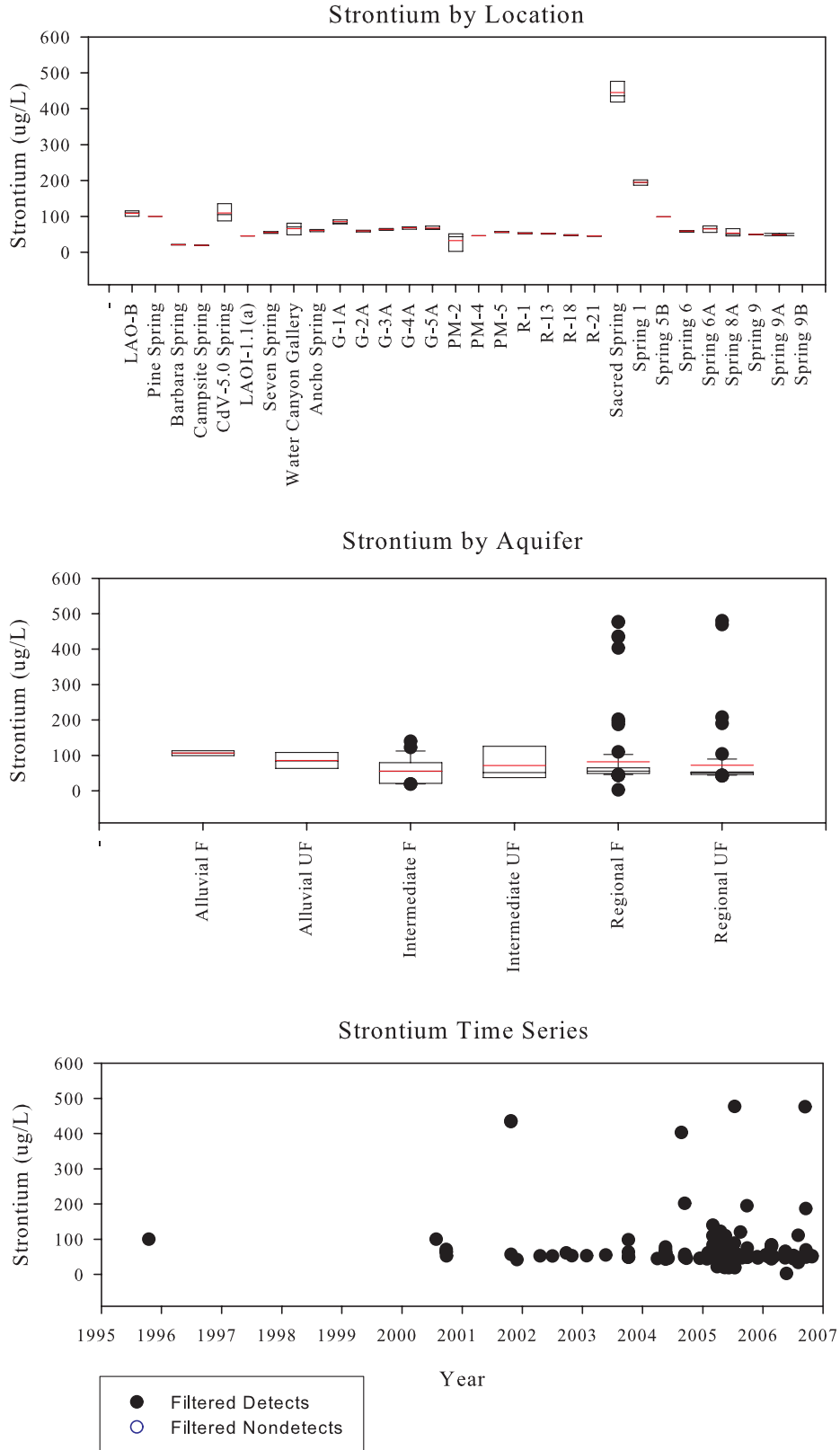
Figure C-44. Strontium
