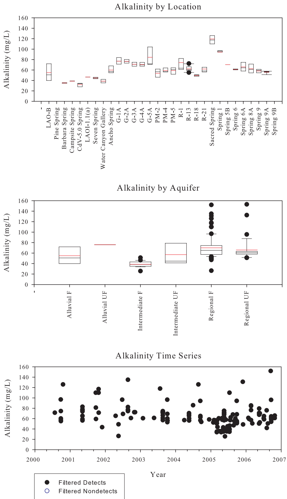
Figure C-1. Alkalinity CO 3 +HCO 3
