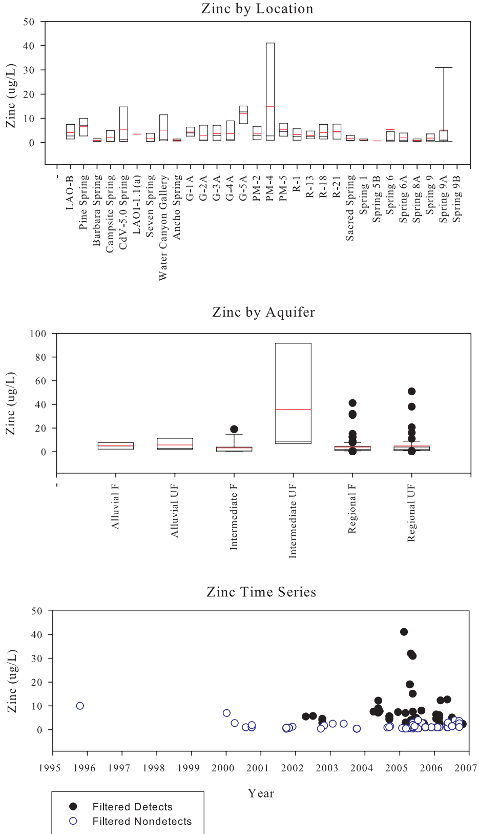
Figure C-50. Zinc
