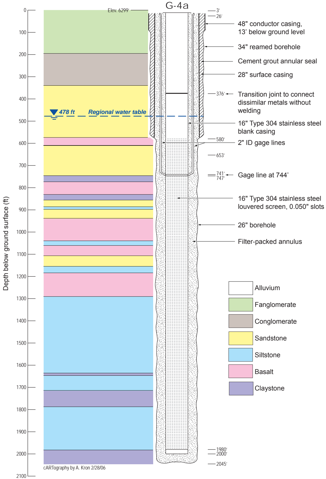
Figure E-16.11. Completion diagram and stratigraphy of well G-4A
