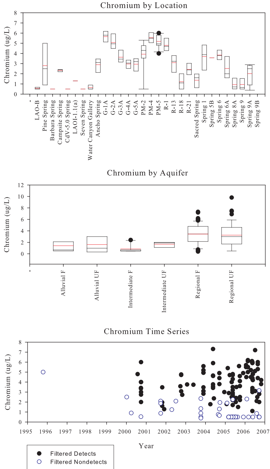
Figure C-29. Chromium
