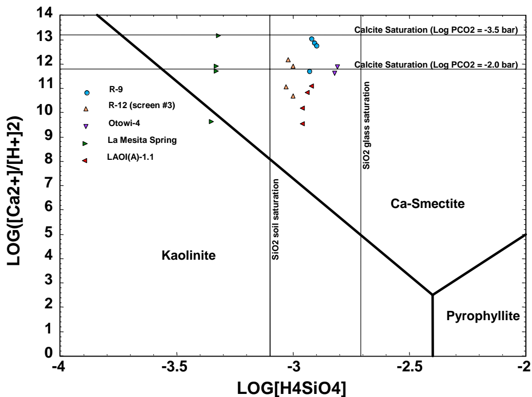
Figure 2.2-5. Activity diagram of \log[H_4SiO_4] versus \log activity (Ca^{2+}/[H^+]^2) at 25°C for wells Otowi-4, R-9, R-12 (screen #3), LAOI(A)-1.1, and La Mesita Spring
