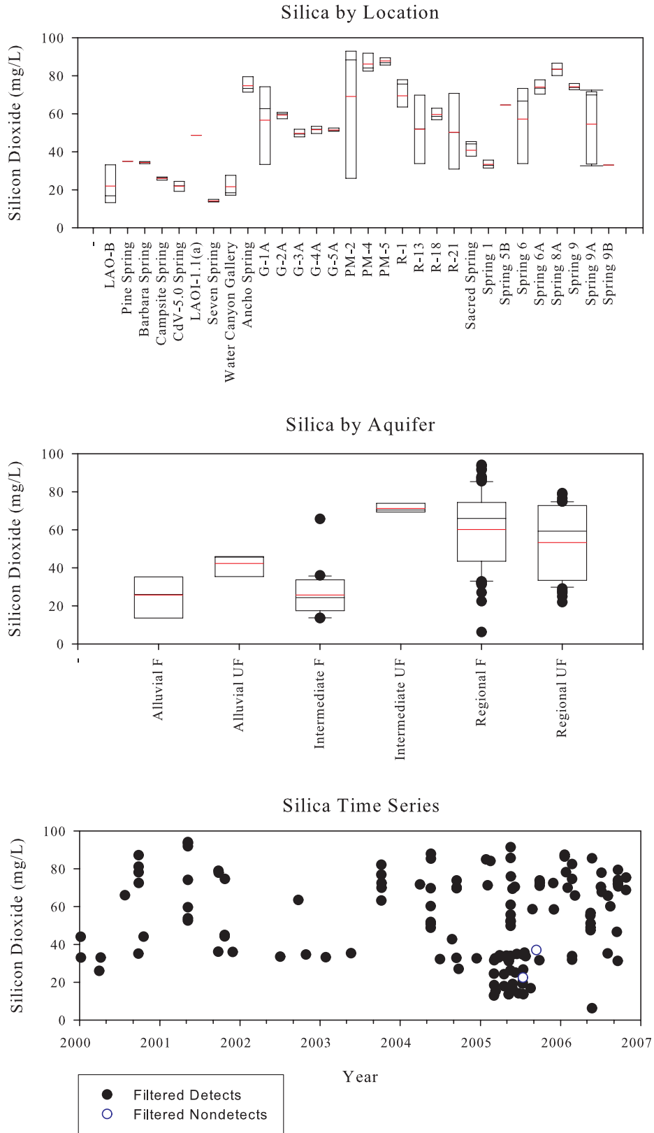
Figure C-12. Silicon Dioxide
