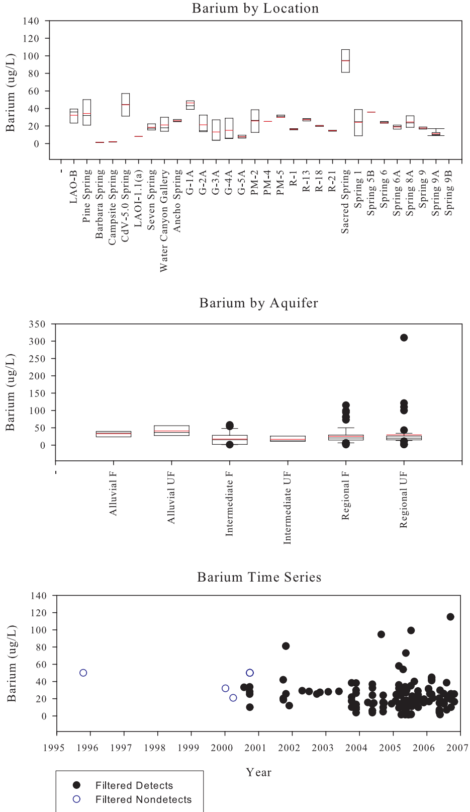
Figure C-24. Barium
