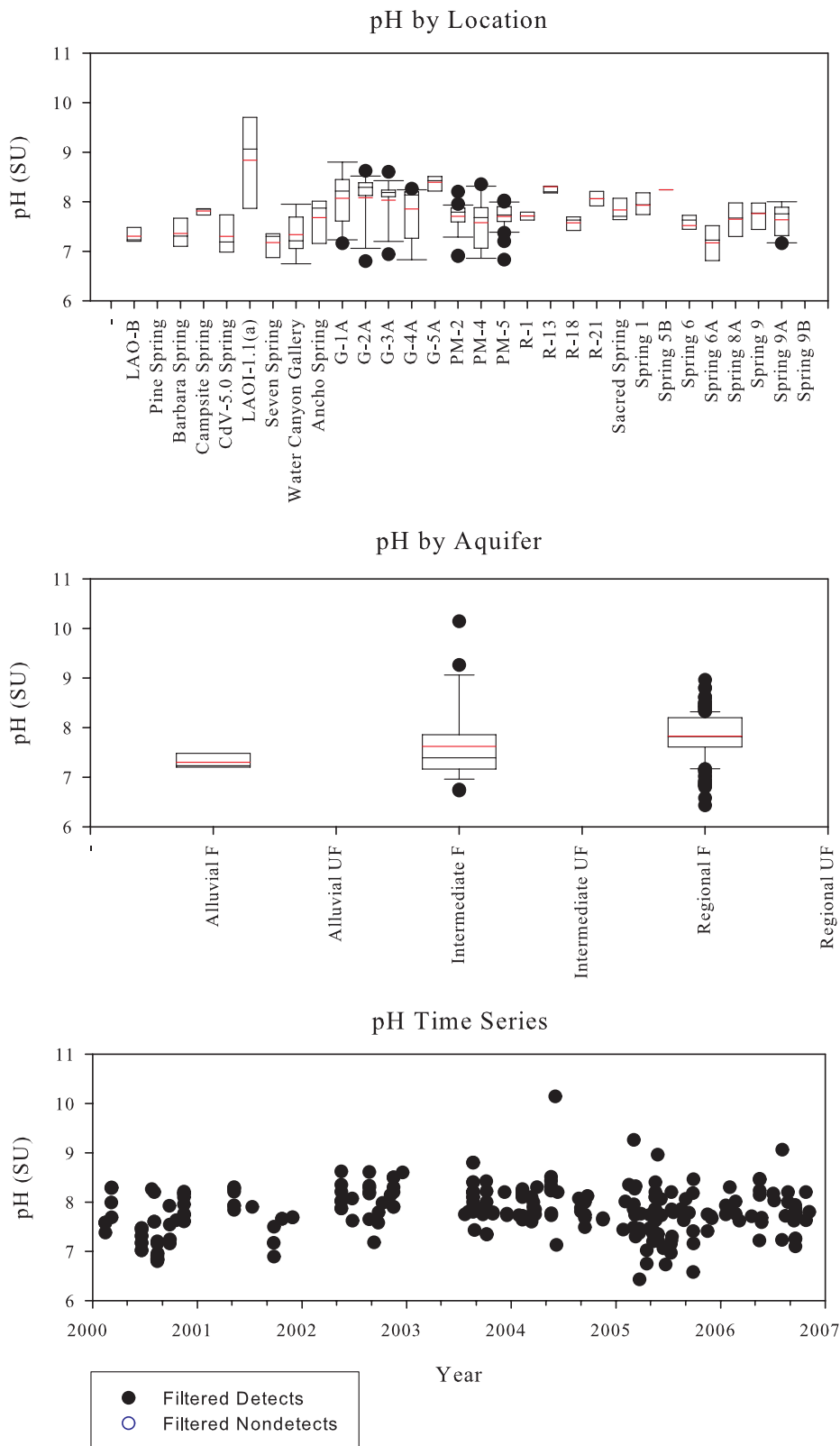
Figure C-19. pH
