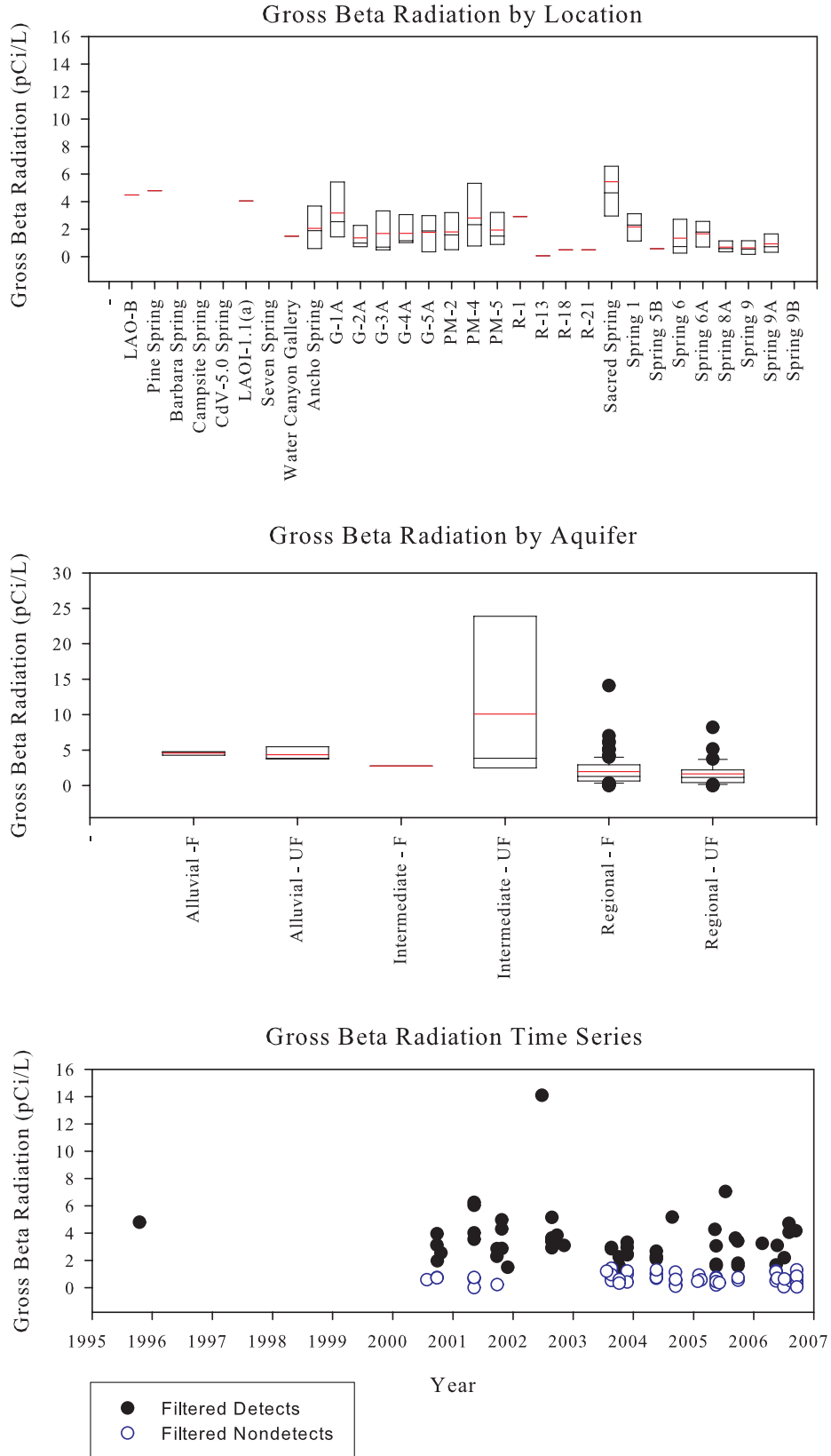
Figure C-55. Gross Beta
