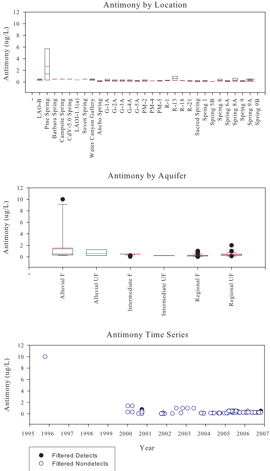
Figure C-22. Antimony
