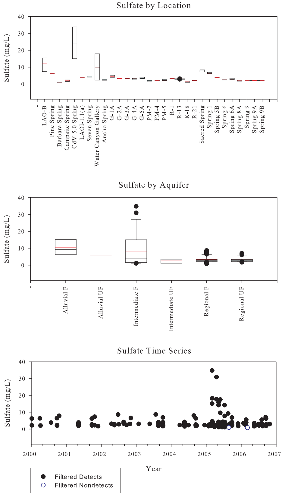
Figure C-13. Sulfate
