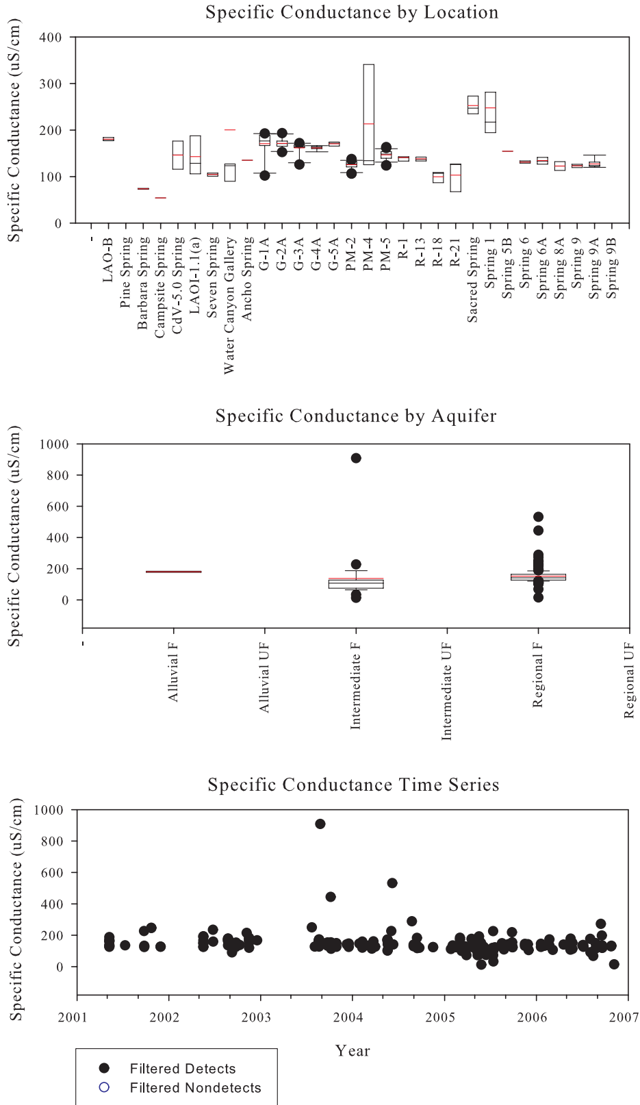
Figure C-20. Specific Conductance
