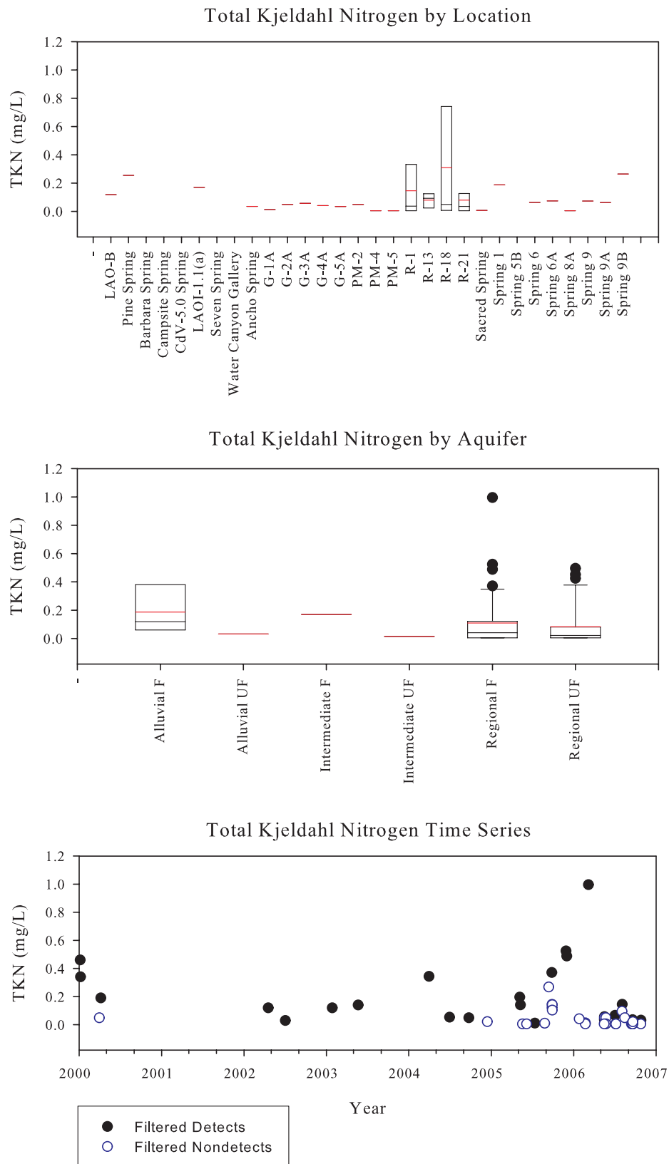
Figure C-15. Total Kjeldahl Nitrogen
