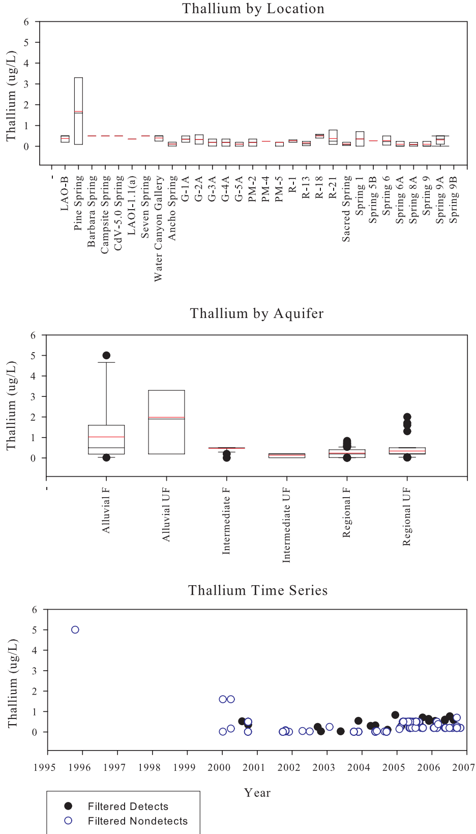
Figure C-45. Thallium
