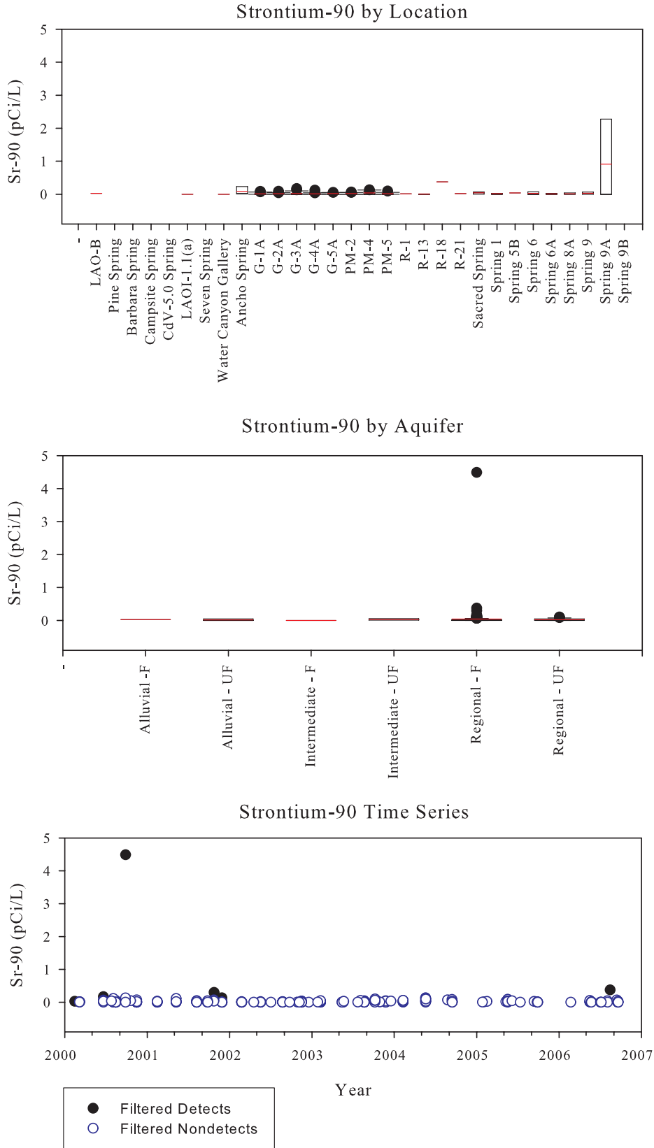
Figure C-58. Strontium-90
