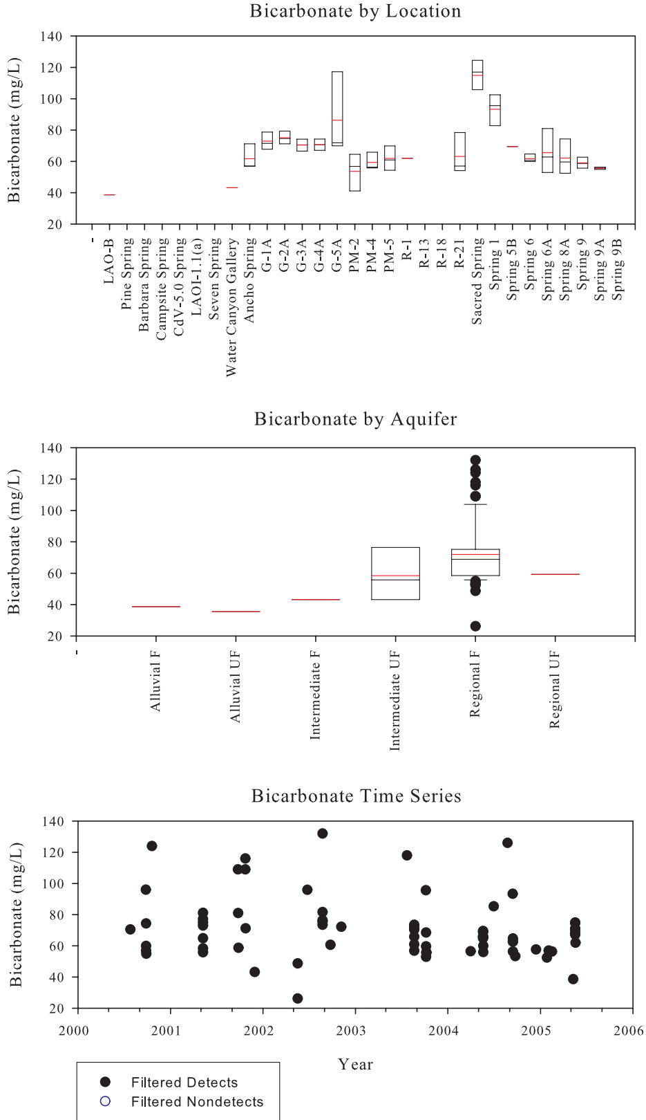
Figure C-2. Alkalinity HCO 3
