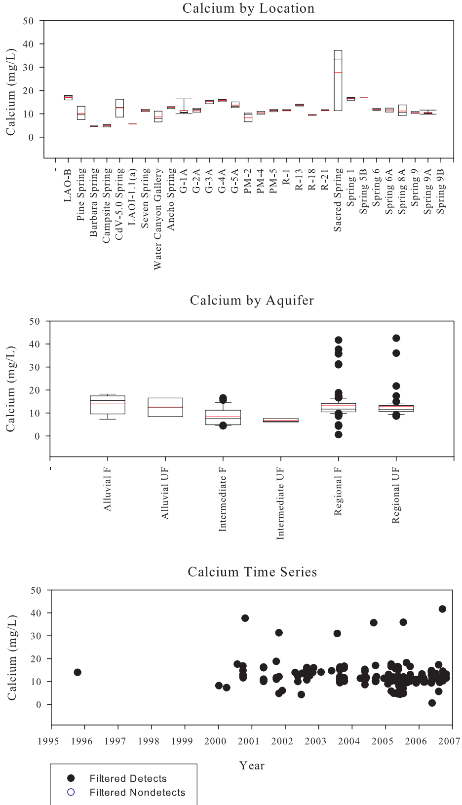
Figure C-28. Calcium
