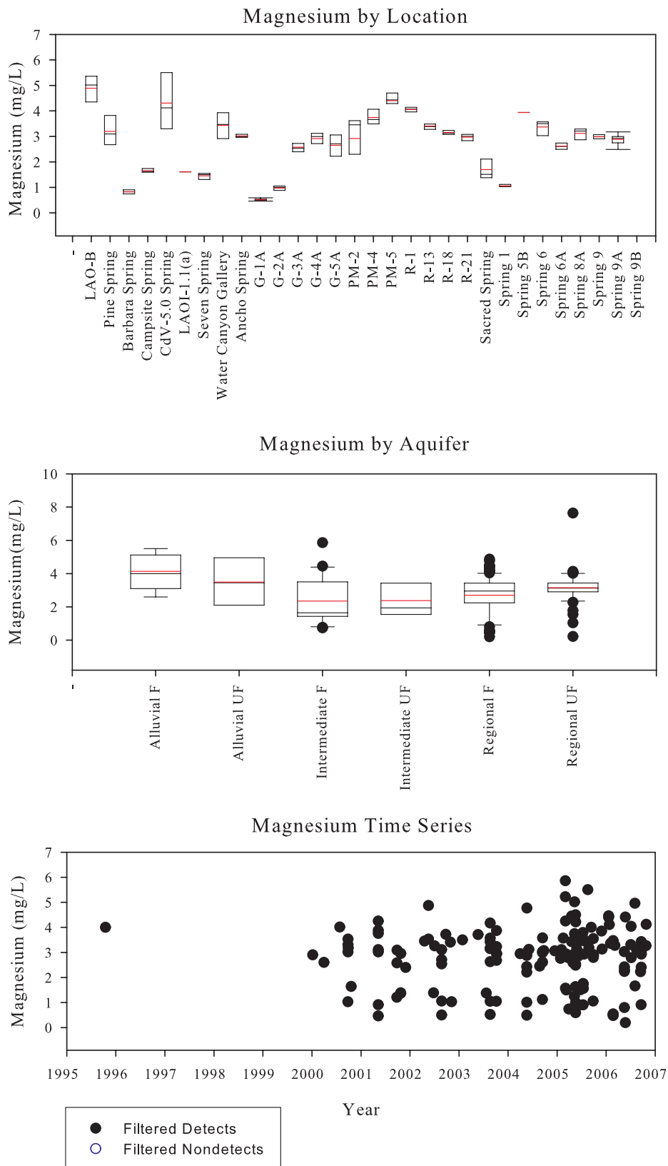
Figure C-35. Magnesium
