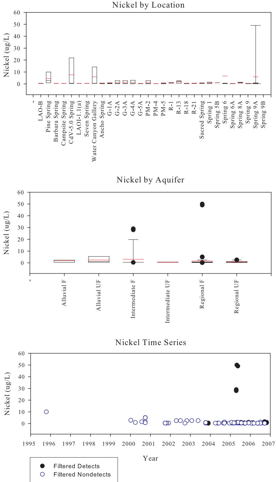
Figure C-39. Nickel
