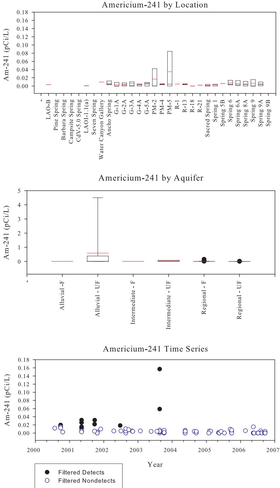
Figure C-52. Americium-241
