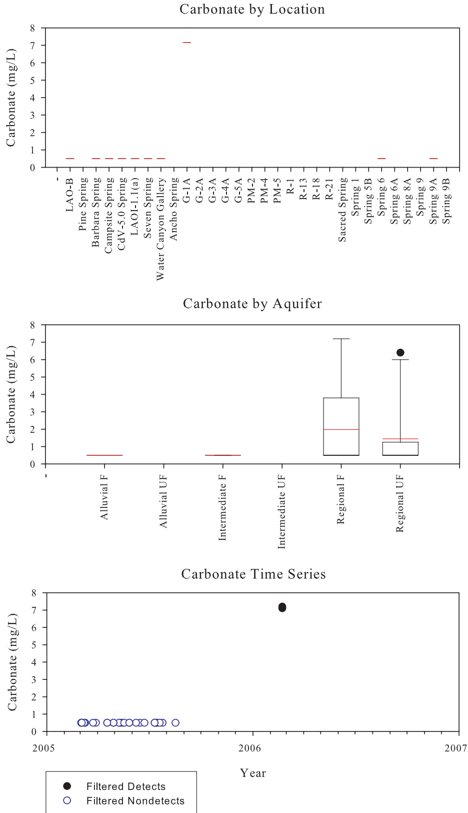
Figure C-5. Carbonate
