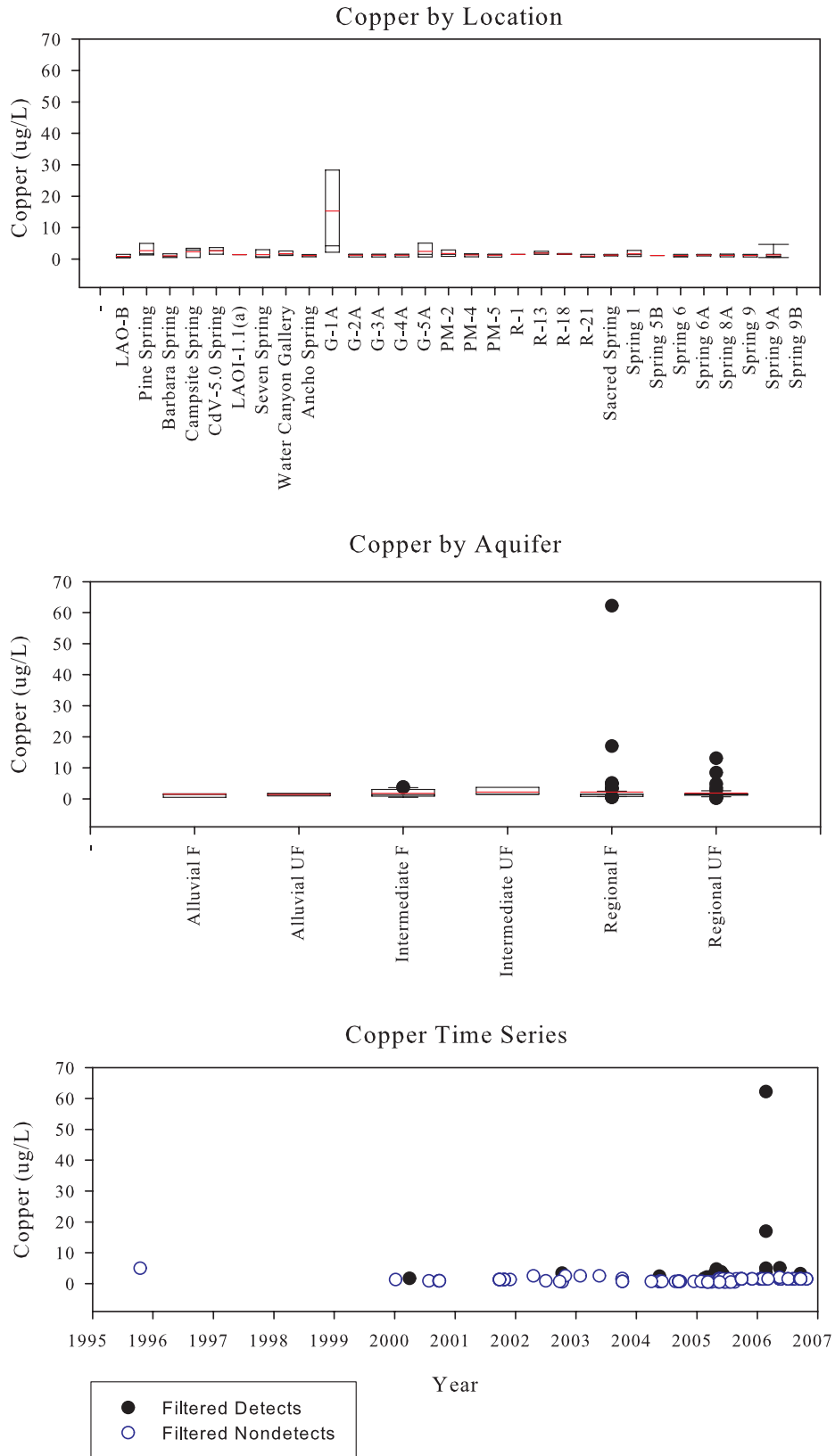
Figure C-31. Copper
