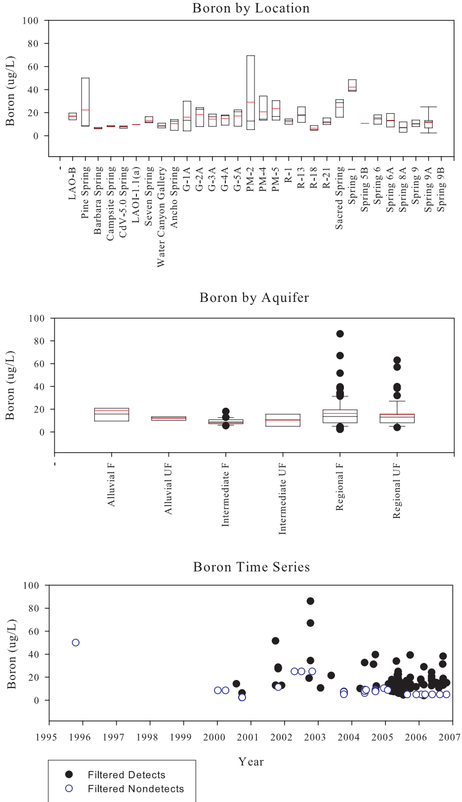
Figure C-26. Boron
