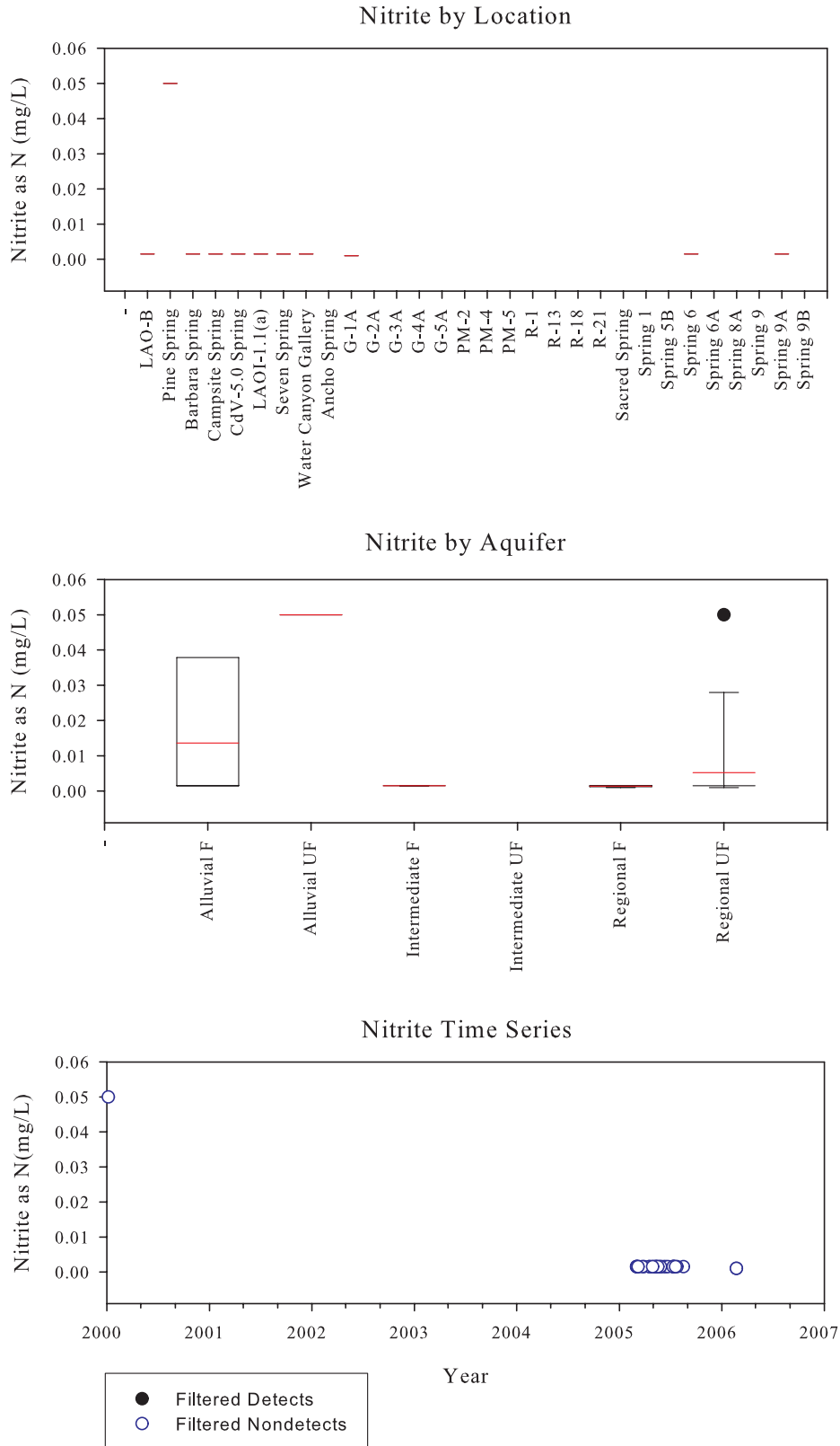
Figure C-10. Nitrite
