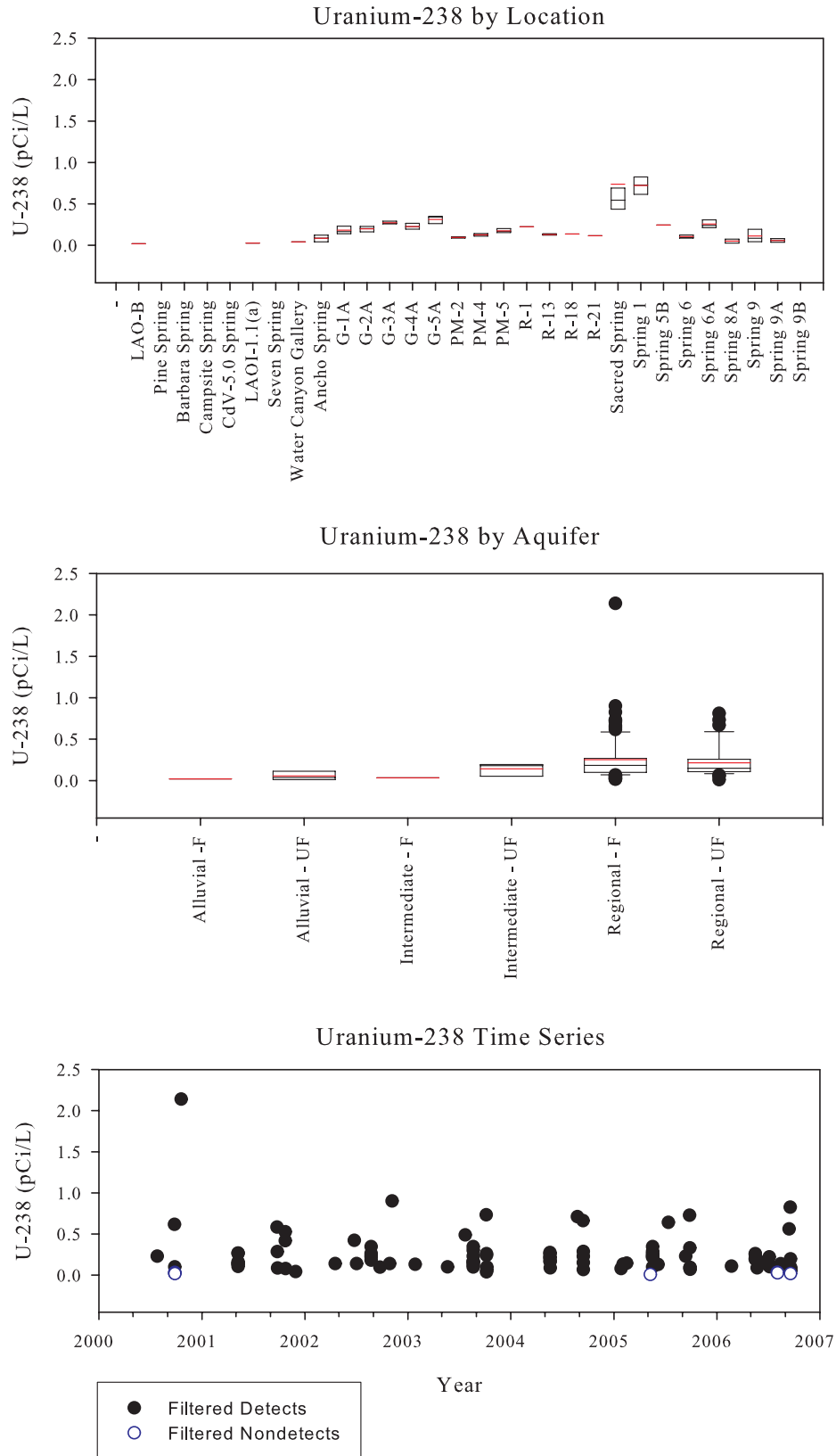
Figure C-60. Uranium-238
