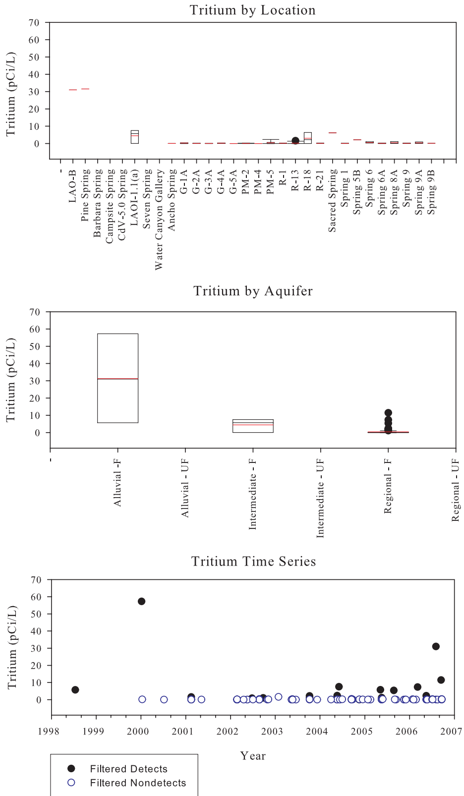
Figure C-51. Tritium
