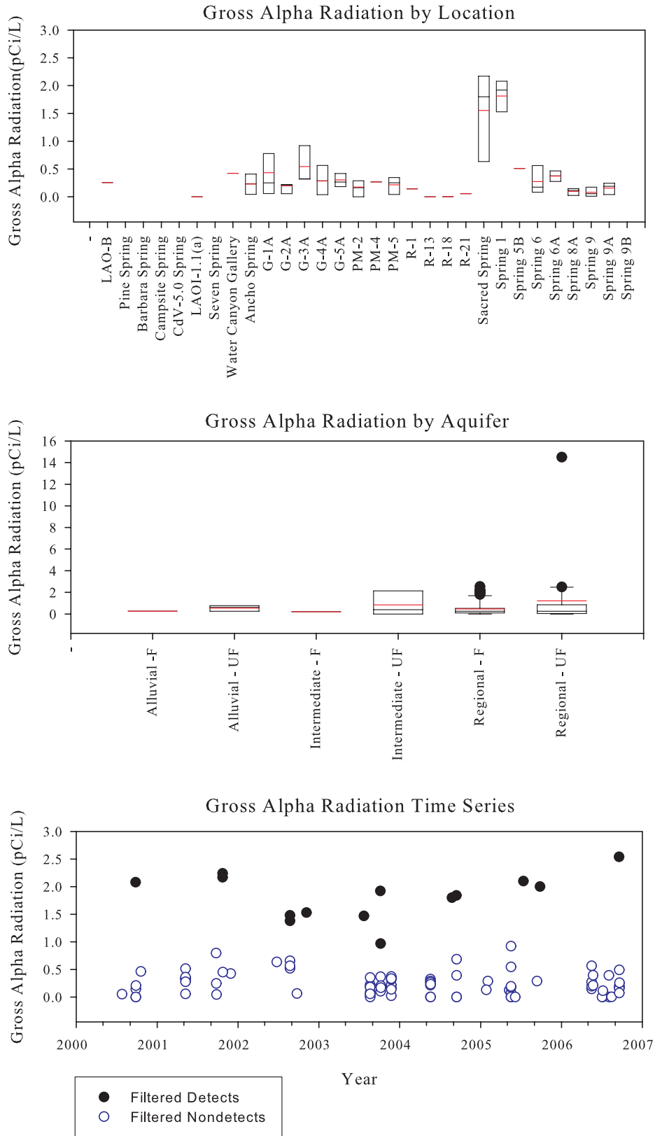
Figure C-54. Gross Alpha
