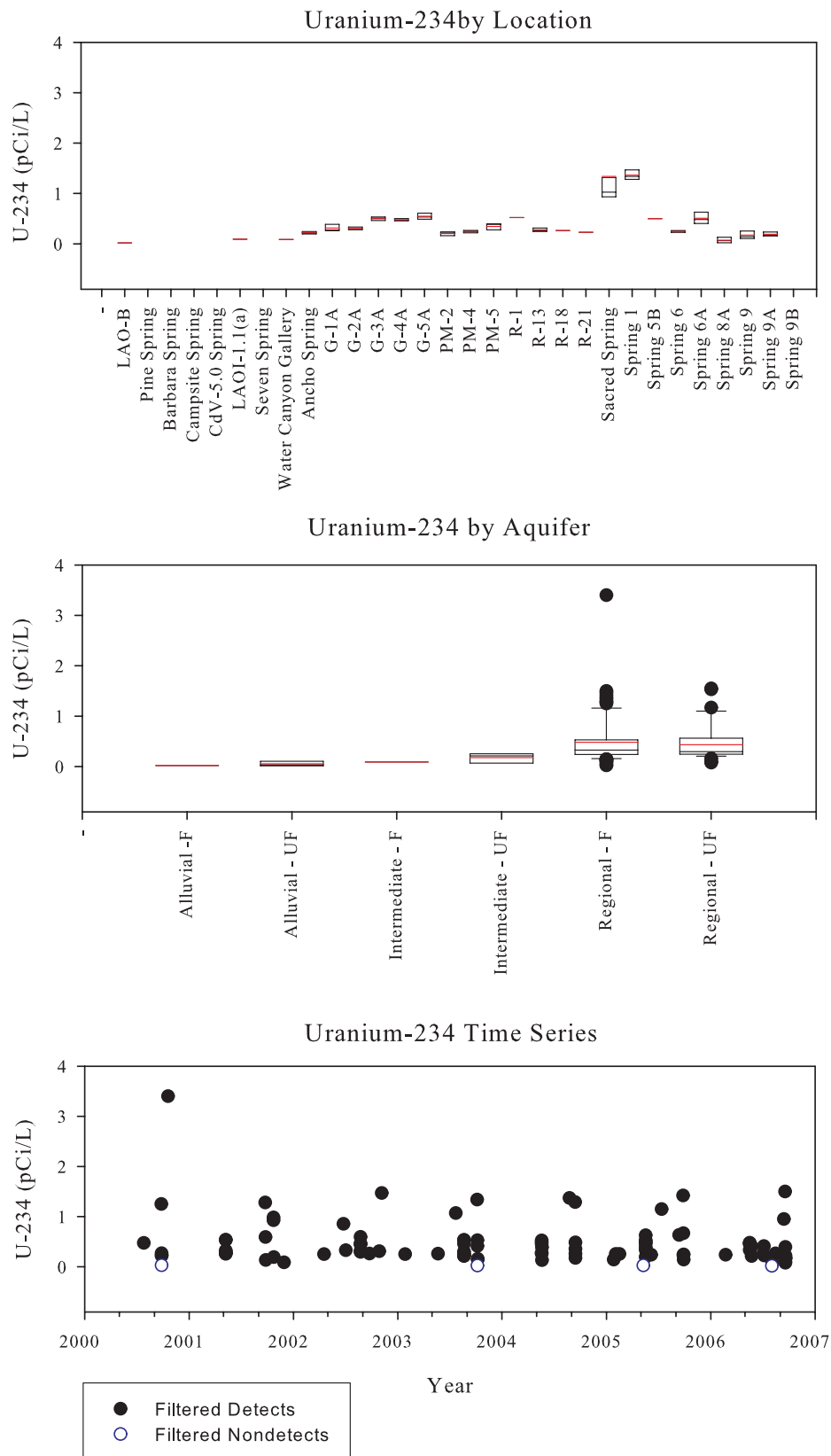
Figure C-59. Uranium-234
