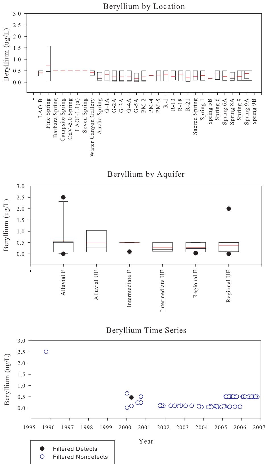
Figure C-25. Beryllium
