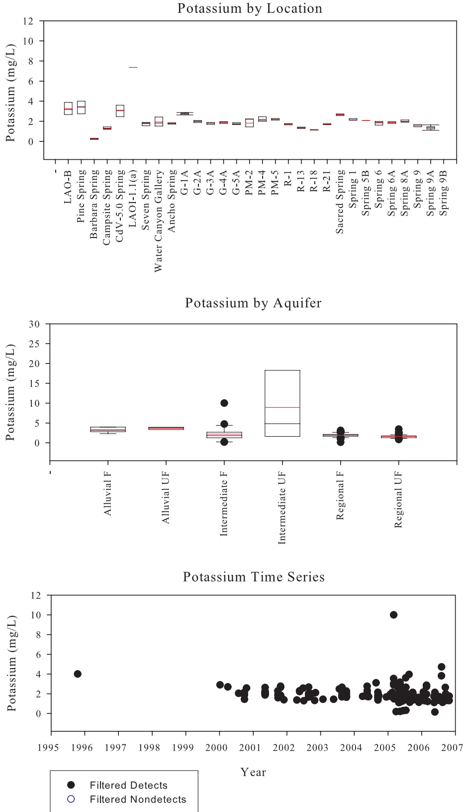
Figure C-40. Potassium
