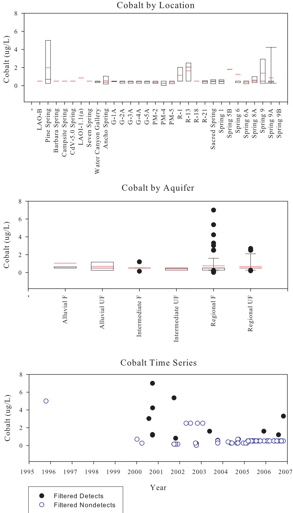
Figure C-30. Cobalt
