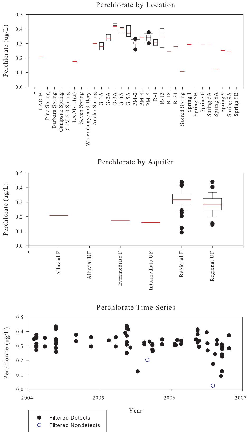
Figure C-11. Perchlorate
