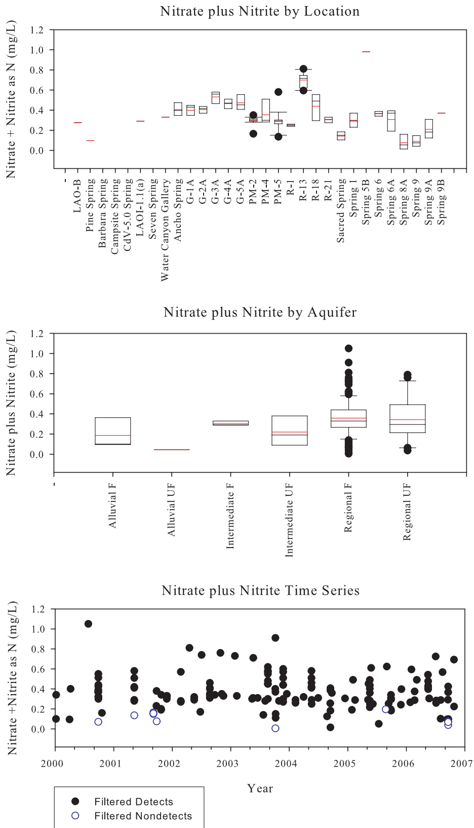
Figure C-9. Nitrate + Nitrite
