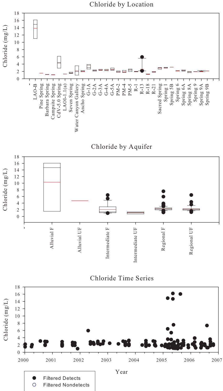
Figure C-6. Chloride
