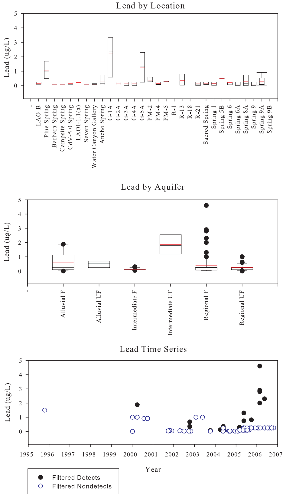
Figure C-33. Lead
