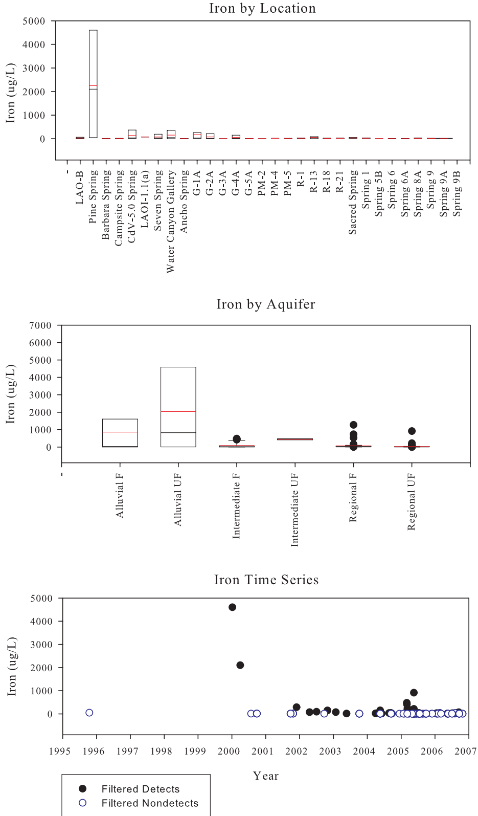
Figure C-32. Iron
