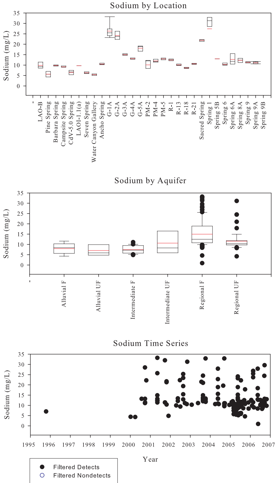
Figure C-43. Sodium
