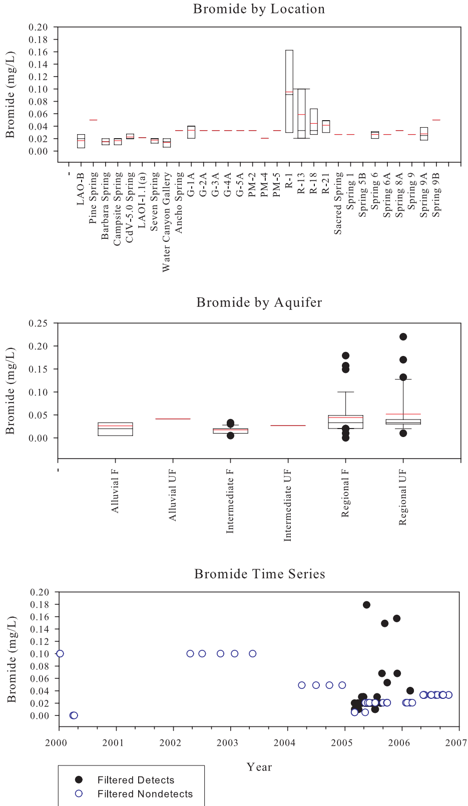
Figure C-4. Bromide
