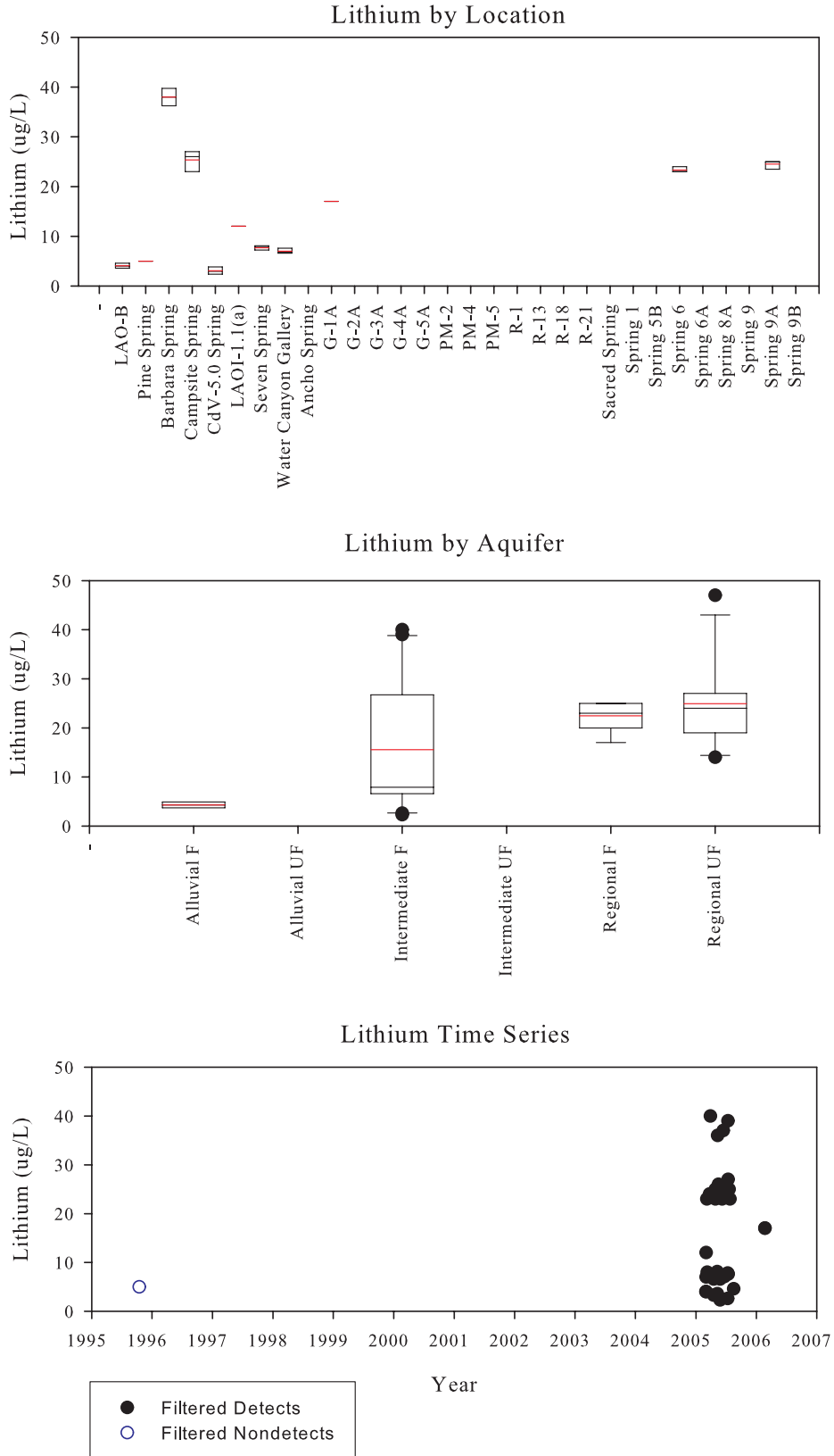
Figure C-34. Lithium
