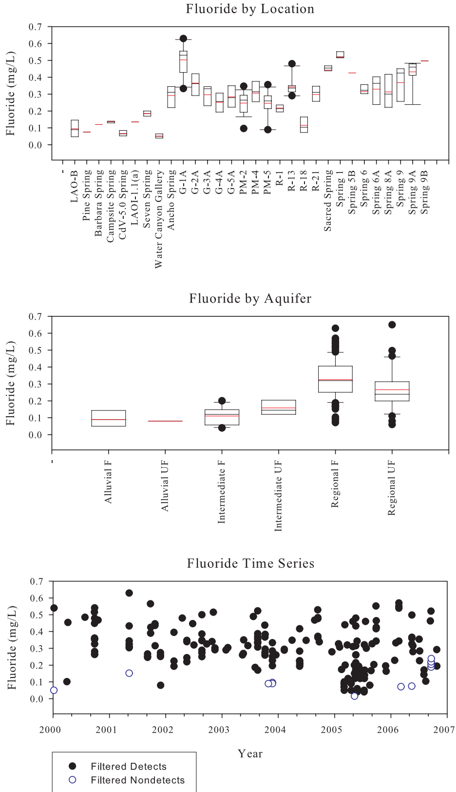
Figure C-7. Fluoride
