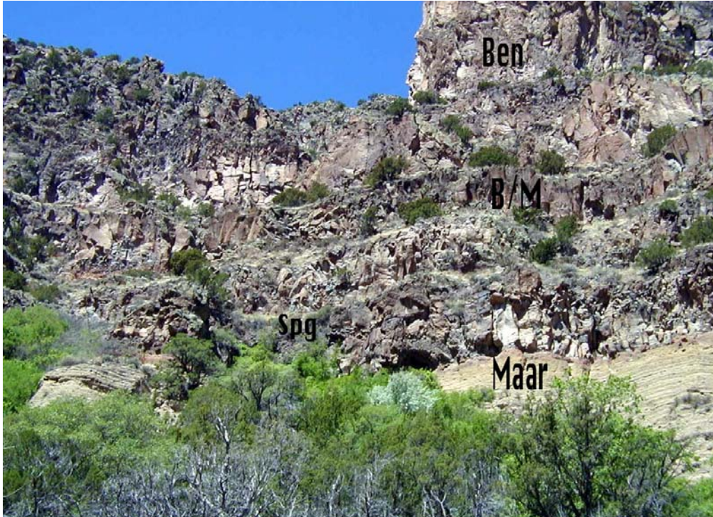
Figure E-1.1. Photograph looking toward the northwest wall of White Rock Canyon showing the location of Spring 9B relative to the local geology. The spring issues from the approximate contact of basaltic hydromagmatic (maar) deposits and an overlying basalt flow. At least two more basalt lavas are interbedded with thin intervals of maar deposits (symbol B/M, located on uppermost basalt). The lava sequence is capped by a thick benmoreite flow (Ben).
