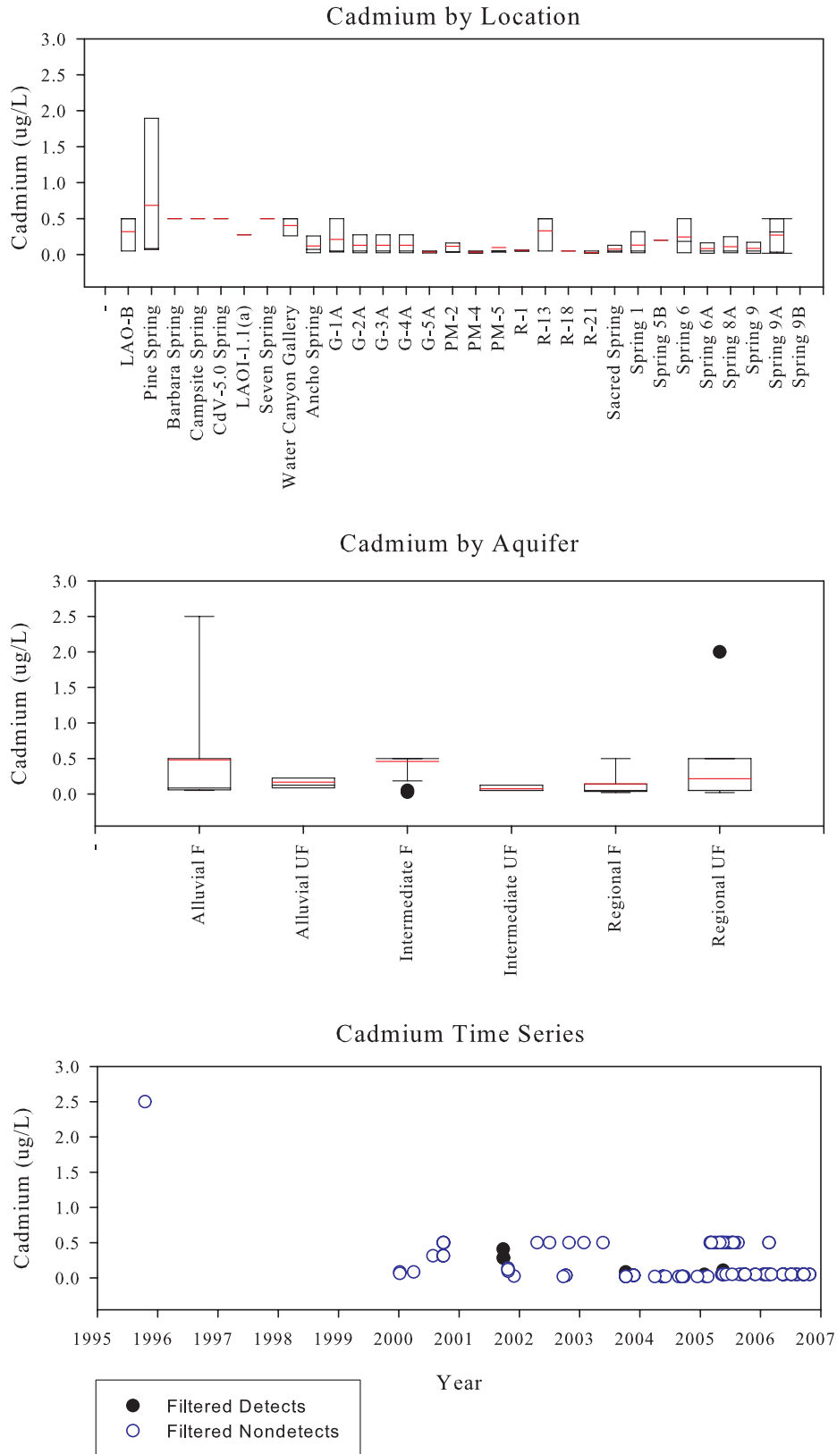
Figure C-27. Cadmium
