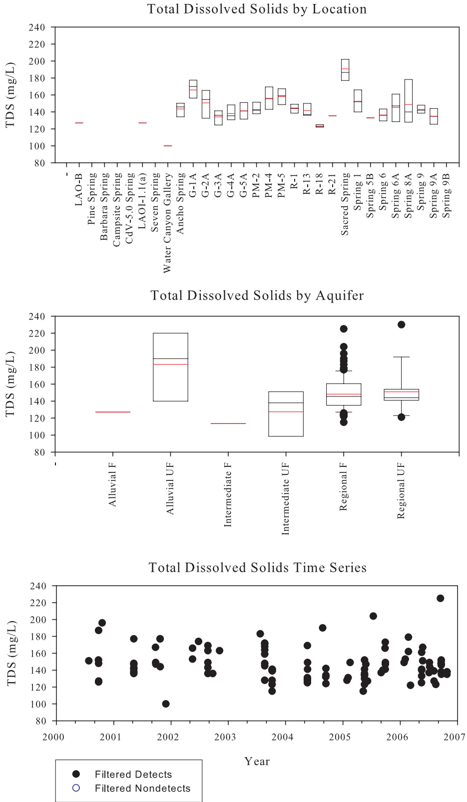
Figure C-14. Total Dissolved Solids
