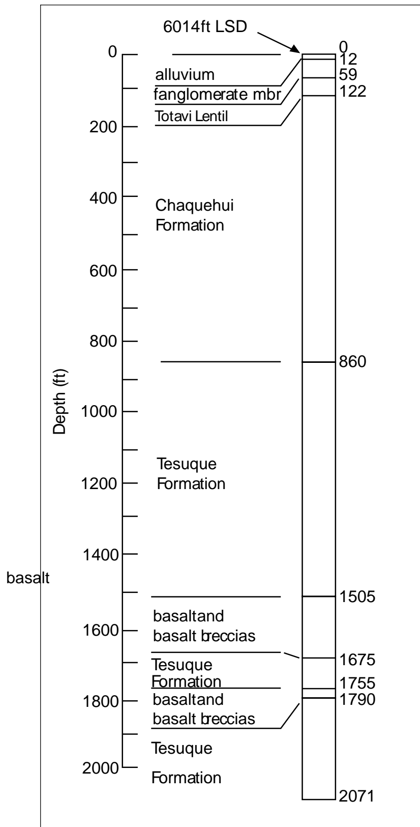
Figure E-16.8. Stratigraphy at well G-1A
