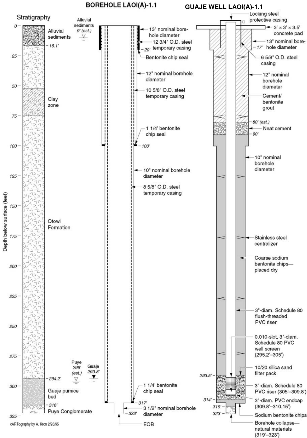
Figure E-7.1. Stratigraphy and completion diagram of LAOI(A)-1.1 well
