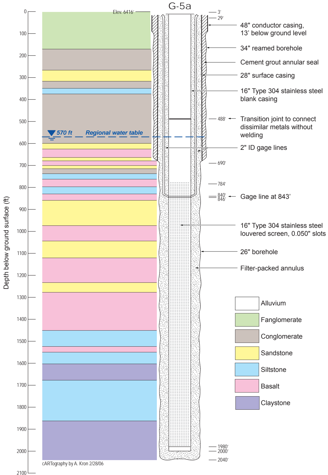
Figure E-16.12. Completion diagram and stratigraphy of well G-5A
