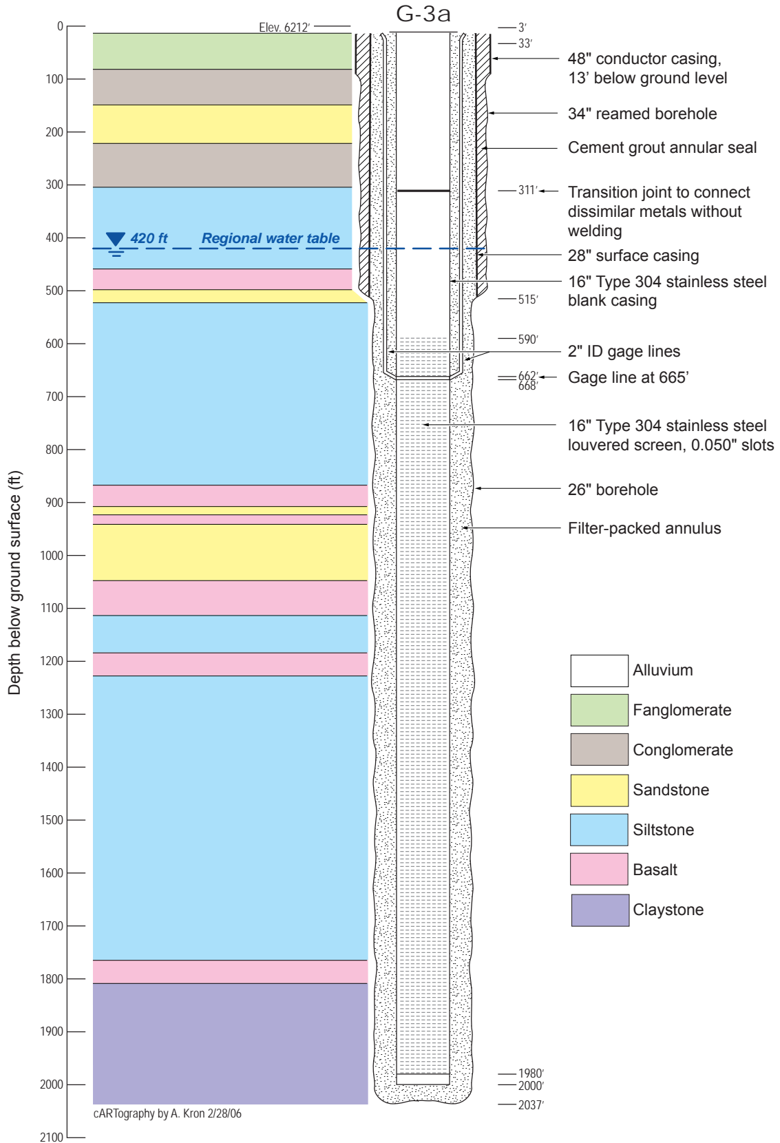
Figure E-16.10. Completion diagram and stratigraphy of well G-3A
