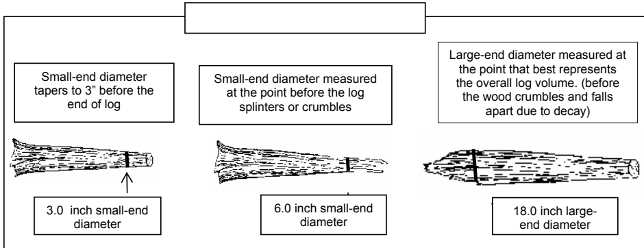
Figure 14-7. Diameter measurements
