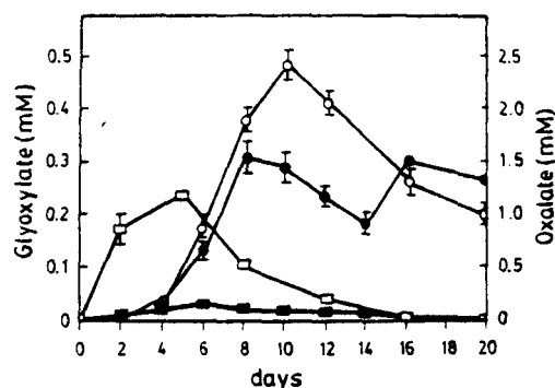
FIG. 2. Time course for oxalate and glyoxylate concentrations in extracellular fluid of C. subvermispora . Cultures grown in defined medium containing ammonium tartrate at an initial concentration of 10 mM (open symbols) or 1 mM (solid symbols) were analyzed to determine their oxalate (circles) and glyoxylate (squares) concentrations.
