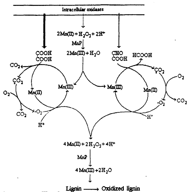
FIG. 6. Proposed scheme for MnP-dependent extracellular oxidation of organic acids in cultures of C. subvermispora .
