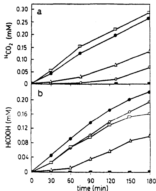
FIG. 4. In vitro oxidation of oxalate and glyoxylate by MnP. Oxalate oxidation was followed by determining ^{14}\text{CO}_2 evolution from [ ^{14}\text{C} ]oxalate (a), and glyoxylate oxidation was followed by determining formate production (b). Reaction mixtures contained 1 mM oxalate (a) or 0.25 mM glyoxylate (b) as individual substrates (○) and in combination (△). Reaction mixtures containing the individual substrates plus 5 \mu\text{M} hydrogen peroxide (□) or 10 \mu\text{M} Mn(III) acetate (●) and reaction mixtures containing the individual substrate but lacking Mn(II) (■) were also examined.
