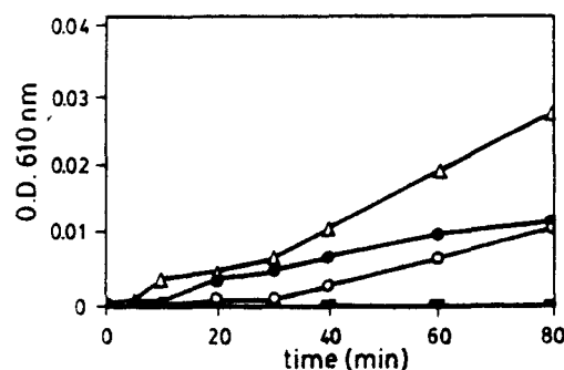
FIG. 5. Organic acid-supported oxidation of phenol red by MnP from C. subvermispora . Assays were conducted with oxalate (○), glyoxylate (●), and oxalate plus glyoxylate (△). No oxidation was observed in reaction mixtures lacking Mn(II) (■). O.D. 610 nm, optical density at 610 nm.
