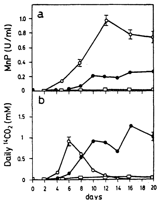
FIG. 3. Time course for MnP titers and oxalate mineralization in cultures. Cultures grown in defined medium containing 10 mM ammonium tartrate (○), defined medium containing 1 mM ammonium tartrate (●), or defined medium containing 10 mM ammonium tartrate but lacking Mn(II) (□) were analyzed to determine MnP activity (a) and [ ^{14}\text{C} ]oxalate mineralization (b).
