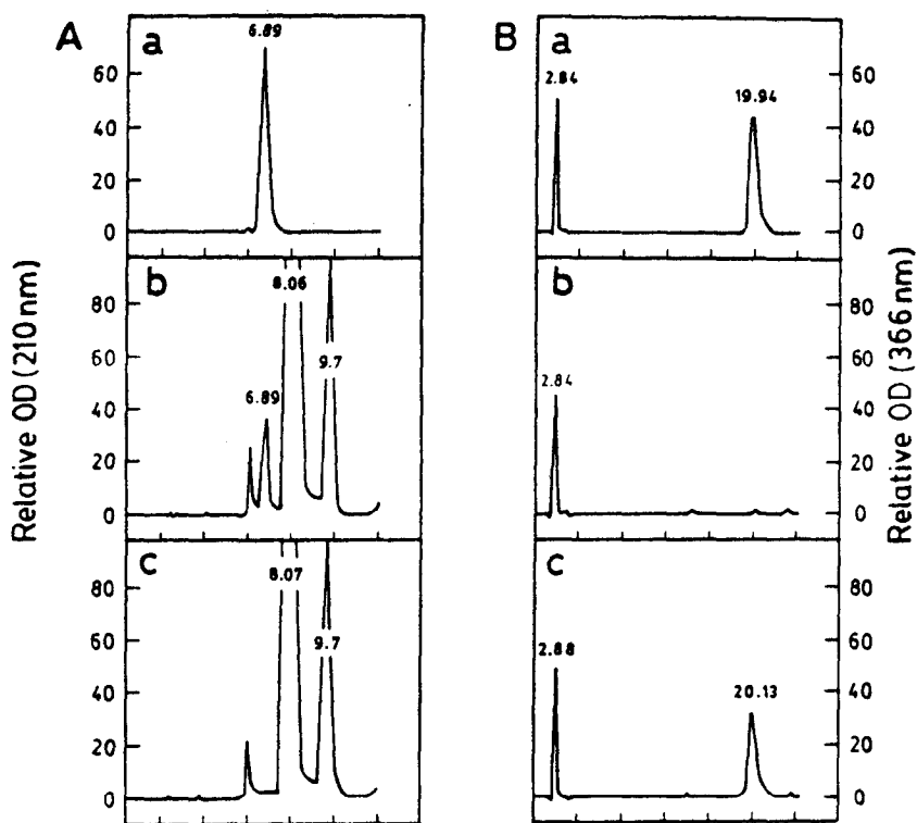
FIG. 1. Identification of oxalate and glyoxylate in the extracellular fluid of C. subvermispora cultures. (A) Underivatized samples were analyzed by ion exclusion HPLC, and elution profiles were determined for oxalate (a), extracellular fluid from day 6 cultures (b), and culture fluid after treatment with oxalate oxidase (c). Major peaks of the profile (8.06 and 9.7 min) were also detected with uninoculated cultures. (B) Samples were derivatized with 2,4-dinitrophenylhydrazine for reverse-phase HPLC analysis of glyoxylate (a), uninoculated growth medium (b), and extracellular fluid of day 9 cultures (c). OD (210 nm), optical density at 210 nm; OD (366 nm), optical density at 366 nm.
