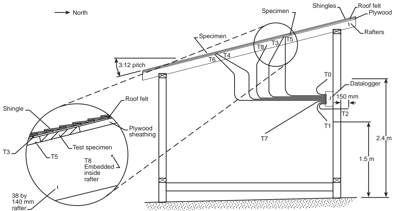
Figure 2—Schematic cross section of instrumented field exposure structure showing location of thermocouples (T0–T8) and channels for datalogger–multiplexer.
