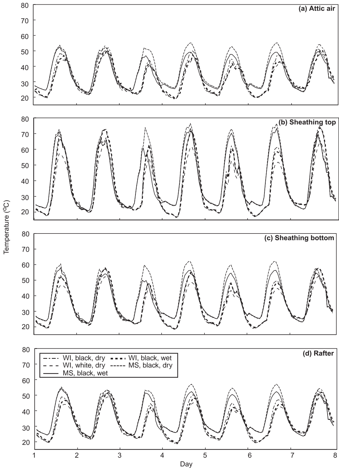
Figure 15—Influence of exposure site and attic humidity during 7 hottest consecutive days in exposure period.
