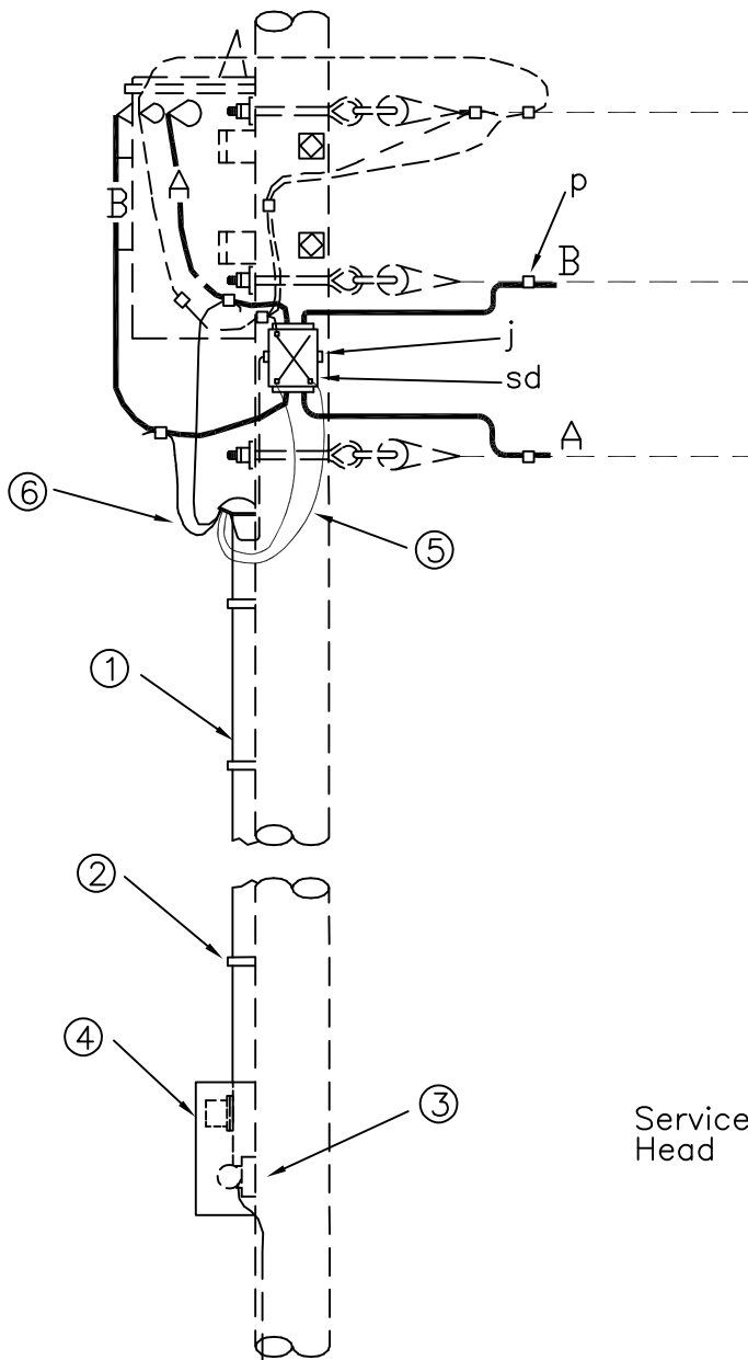
TRIPLEX SERVICE
