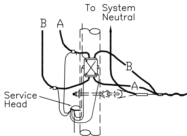
TRIPLEX SERVICE
