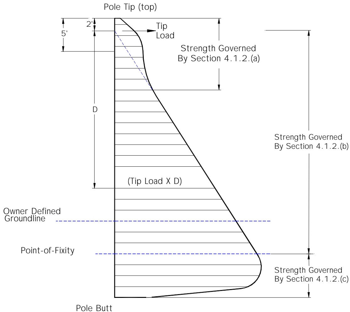
FIGURE 1 Minimum Ultimate Moment Capacity Diagram along the Pole
