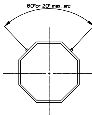
TYPICAL ORIENTATION FOR STEPBOLT CLIPS OR NUTS
