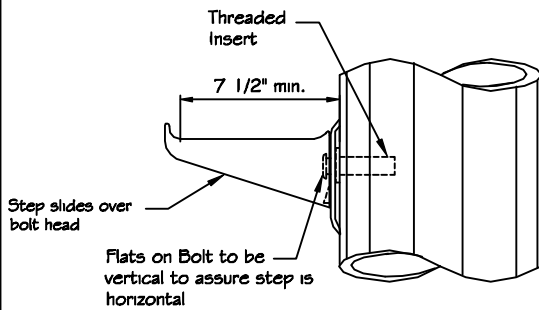
FOR GALVANIZED AND PAINTED STEEL
