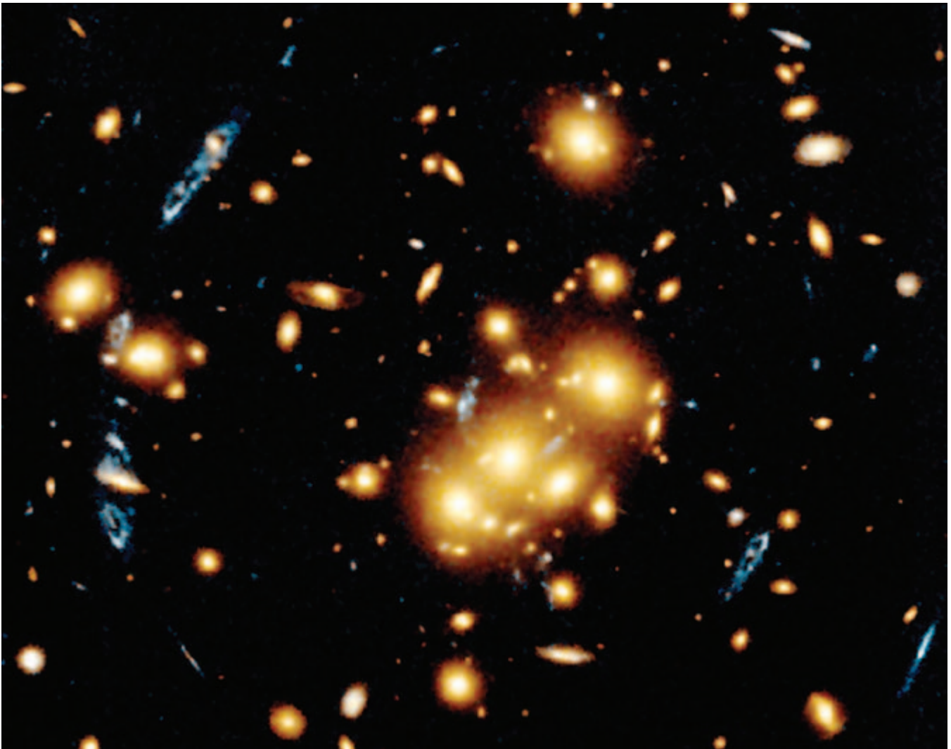
The ring of distortions gives valuable information about the distribution of dark, unseen matter in the cluster. The ring, a prediction of General Relativity, is called an "Einstein Ring." Credit: NASA/Hubble Space Telescope (HST)
