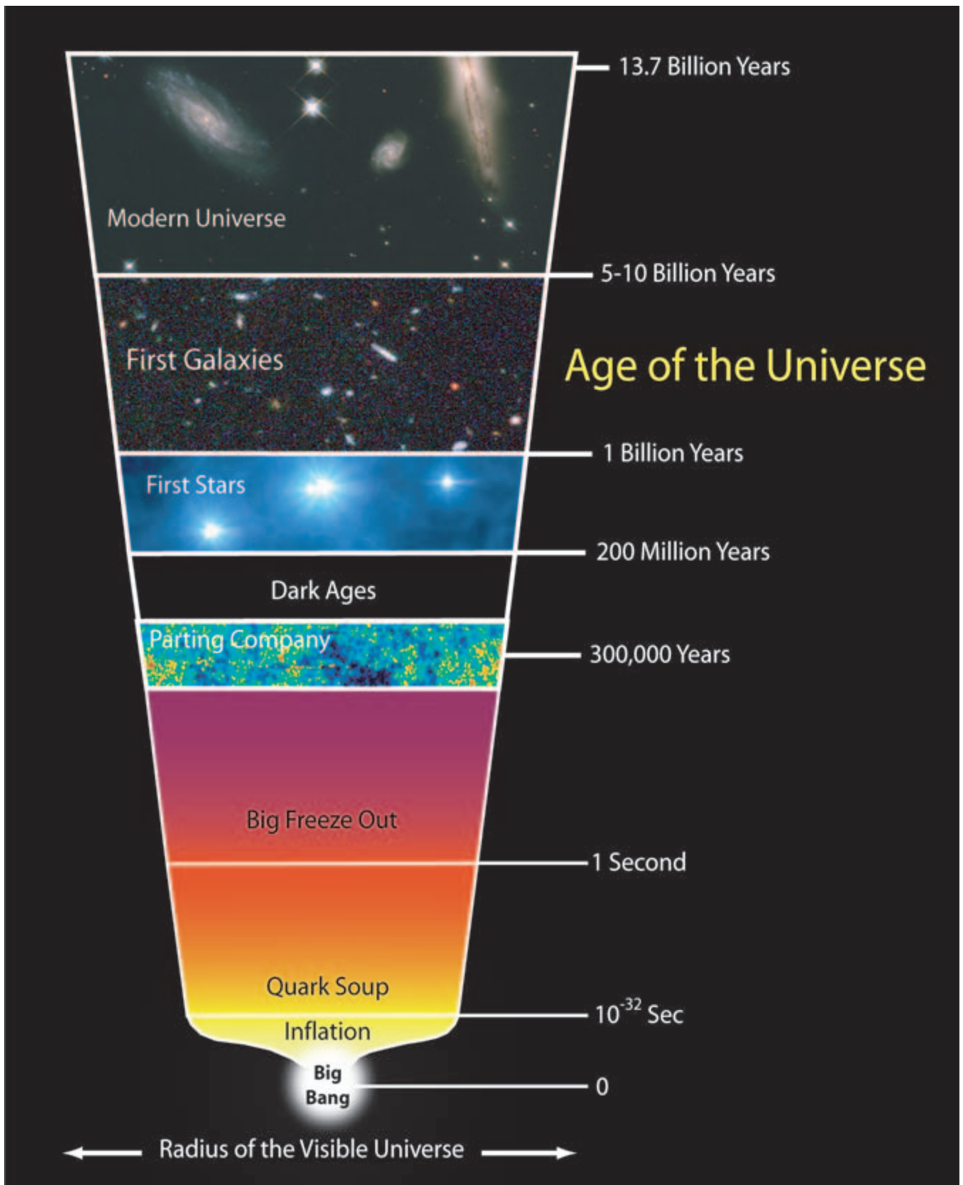
The figure illustrates the timeline of the universe's expansion from the Big Bang to the present. Key stages include the initial inflation, the formation of quark soup, the Big Freeze Out, the parting company (recombination), the dark ages, the formation of the first stars and galaxies, and the modern universe. The timeline is marked with specific time intervals: 10^{-32} seconds for inflation, 1 second for the Big Freeze Out, 300,000 years for the parting company, 200 million years for the first stars, 1 billion years for the first galaxies, and 5-10 billion years for the modern universe. The total age of the universe is 13.7 billion years. The diagram also indicates the radius of the visible universe.
