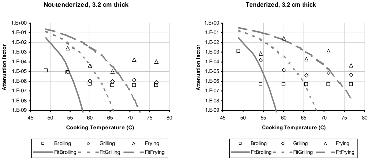
Figure 4: Best fit curves to Spring (1999) data for broiling, grilling, and frying 3.2 cm thick intact (not tenderized) and non-intact (tenderized steaks). Not shown: data for 1.3 and 1.9 cm thick steaks.
