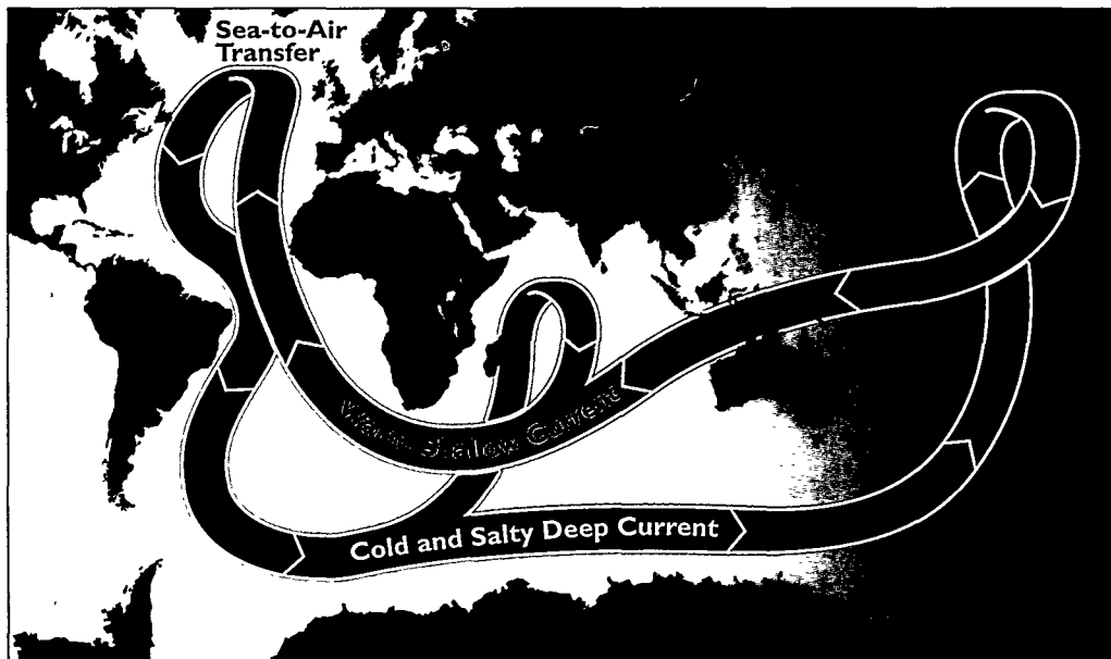
A GLOBAL CONVEYOR BELT The connectedness of the world's oceans is suggested by this schematic depiction of the "great ocean conveyor." Evaporation in the North Atlantic and transfer of the vapor to the Pacific leaves behind saltier water, which then sinks and drives the cold deep current. The warm surface current has a direct impact on world weather, accounting, for example, for Northern Europe's relatively mild winters. Many of the details of this global conveyor were revealed by early AEC-sponsored research.
