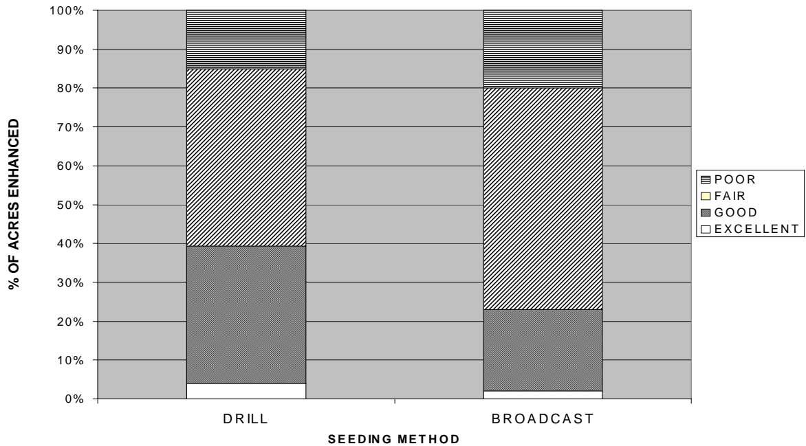
FIGURE 2. FORB / LEGUME ENHANCEMENT ESTABLISHMENT RATINGS FOR SEEDING METHODS
