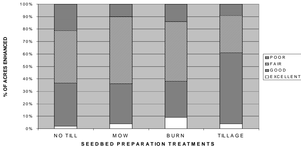
FIGURE 1. FORB / LEGUME ENHANCEMENT ESTABLISHMENT RATINGS FOR SEEDBED PREPARATION TREATMENTS
