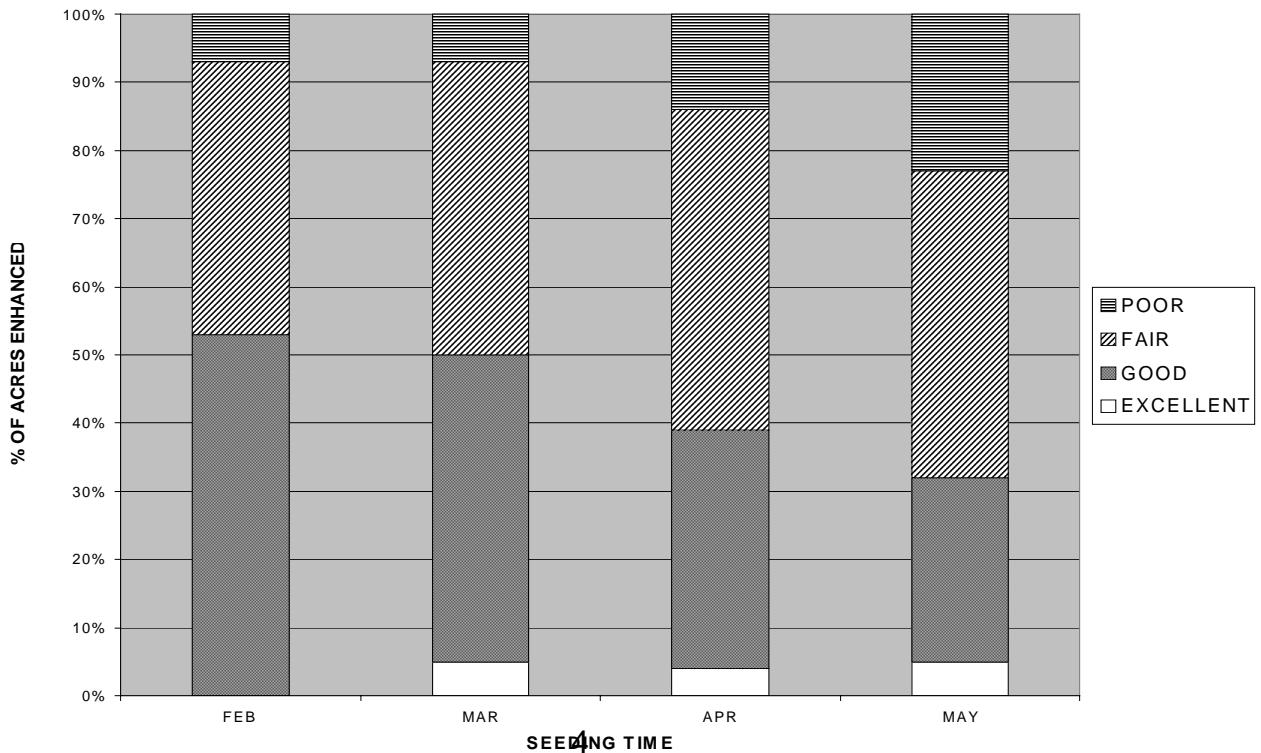
FIGURE 3. FORB / LEGUME ENHANCEMENT ESTABLISHMENT RATINGS FOR TIME OF SEEDING
