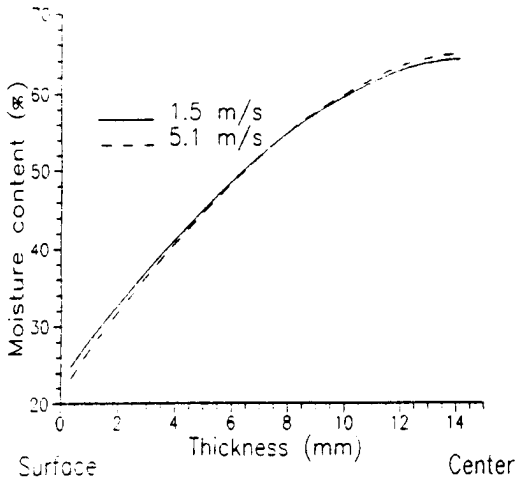
FIG. 2. Effect of air velocity on calculated moisture content gradient at 50 percent average moisture content.
