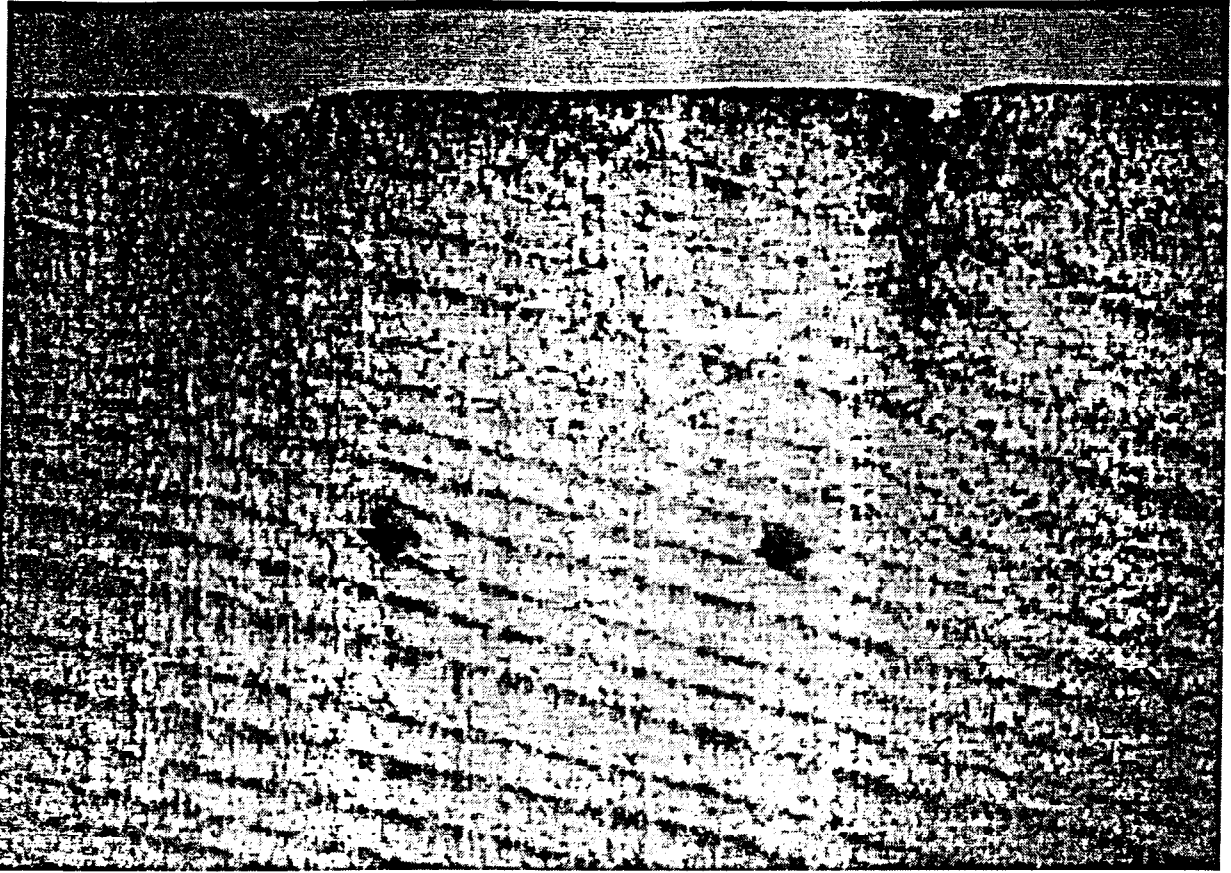
Figure 3-End view of incision from a knife-like 5-mm-deep incision at an incision density of 8,500/\text{m}^2 into dry Douglas Fir.
