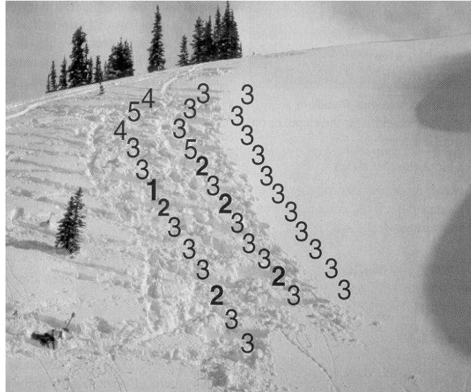
Figure 1: Spatial measurements of point stability on a small slope (Columbia Mountains, western Canada) using the rutschblock test ( N = 36 ). The slope median stability test score was 3 with a quartile coefficient of variation (QCV) of 0 (the interquartile range only included test scores of 3). For comparison, the coefficient of variation which, however, is not an appropriate measure for ordinal stability data was 25%. The slope does not show any spatial structure except some small clusters of lower and higher stability (near the tree at the top of the slope) (from Jamieson, 1995, p.161).
