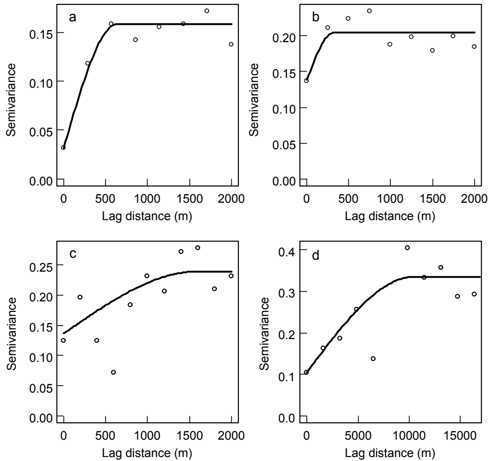
Figure 6: Multi-scale geostatistical analysis: sample ( \circ ) and model (—) indicator semi-variogram for surface hoar presence at increasing scale. (a) Using results from 30 penetration resistance (SMP) profiles and 54 manual profiles within a region. (b) Using only results from the 54 manual profiles within the region. (c) Using only the 27 manual profiles in another region. (d) Using the 30 SMP profiles and all 81 manual profiles from both regions (from Schweizer and Kronholm, 2007).
