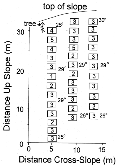
Figure 1: Spatial measurements of point stability on a small slope (Columbia Mountains, western Canada) using the rutschblock test ( N = 36 ). The slope median stability test score was 3 with a quartile coefficient of variation (QCV) of 0 (the interquartile range only included test scores of 3). For comparison, the coefficient of variation which, however, is not an appropriate measure for ordinal stability data was 25%. The slope does not show any spatial structure except some small clusters of lower and higher stability (near the tree at the top of the slope) (from Jamieson, 1995, p.161).
