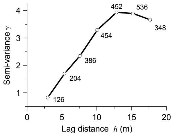
Figure 3: Semi-variogram for the spatial data from Mt. Abbott shown in Figure 2. Numbers indicate numbers of point pairs. The geostatistical analysis suggests a range of about 10-15 m (from Campbell, 2004, p. 87).
