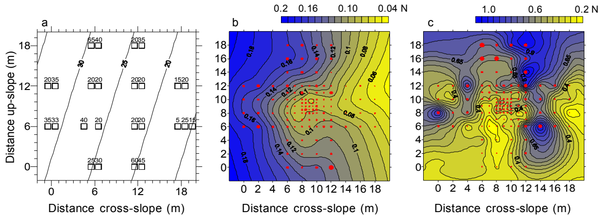
Figure 4: (a) Results of stability measurements (rammrutsch) on a small slope for a buried layer of surface hoar (17 January 2003). The drop height (in cm) that is a measure of stability, is shown above the test location. A linear slope stability trend was found and indicated by 5 cm contours. The median drop height was 20 cm with a quartile coefficient of variation of 27% before and 22% after trend removal [from Kronholm, 2004]. (b) Penetration resistance (SMP) of the same layer of buried surface hoar as shown above in (a). The layer was found at all measurement locations on the slope and showed a strong slope-scale trend in resistance. Red circles indicate measurement locations and are scaled to the measured resistance. A pure-nugget semi-variance was found after trend removal, i.e. no additional spatial structure was found after linear trend removal. (c) Same type of figure as in (b) for a wind-slab of small rounded grains and some facets. The layer showed smaller-scale spatial structure with a range of about 6 m.
