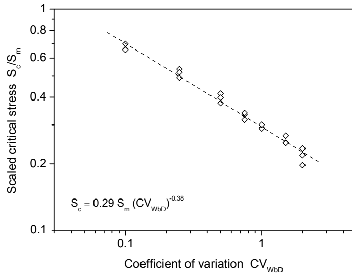
Figure 7: Simulation results using a lattice automaton model: effect of random variations in weak layer strength on slope failure strength. Variation of weak layer strength is given as the coefficient of variation of the Weibull distribution CV_{WbD} . The critical stress S_c at which the slope fails is scaled to the average weak layer strength S_m . Dotted lines indicates power law fit to simulation results (adapted from Fyffe, 2006).
