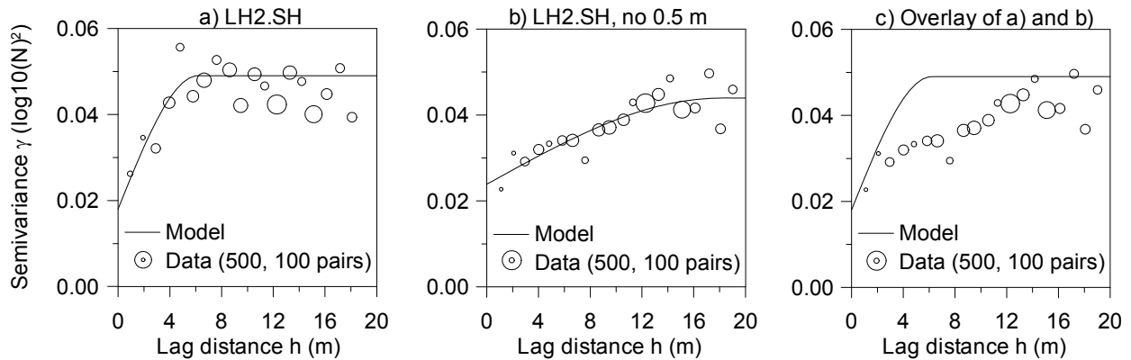
Figure 8: (a) Spherical semi-variogram model fitted to the penetration resistance (SMP) of a layer of buried surface hoar (LH2.SH) at a planar, wind-protected site. Circles are scaled to the number of point-pairs. (b) When the measurements with the smallest spacing (0.5 m) were removed from the data, the semi-variogram changed significantly, demonstrating that the sampling scheme is critically important for interpreting the results of the geostatistical analysis. (c) shows the modeled semi-variogram for all the data, with the data points for the data with the 0.5 m grid removed to emphasize the difference when the fine grid is removed (from Birkeland et al., 2004b).
