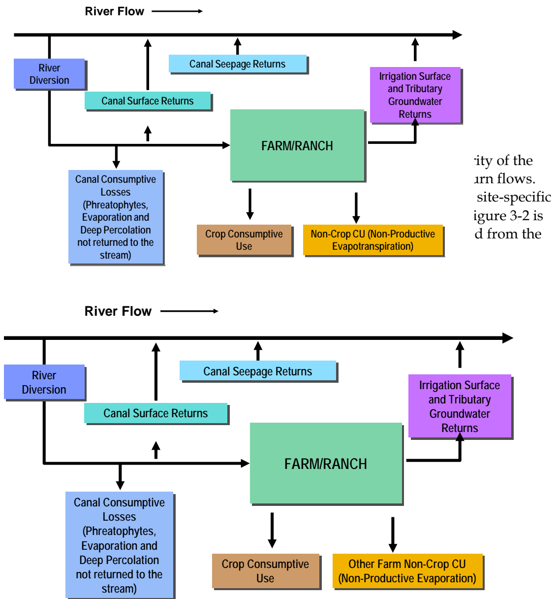
Figure 3-2 Irrigation System Schematic Including Return Flows
