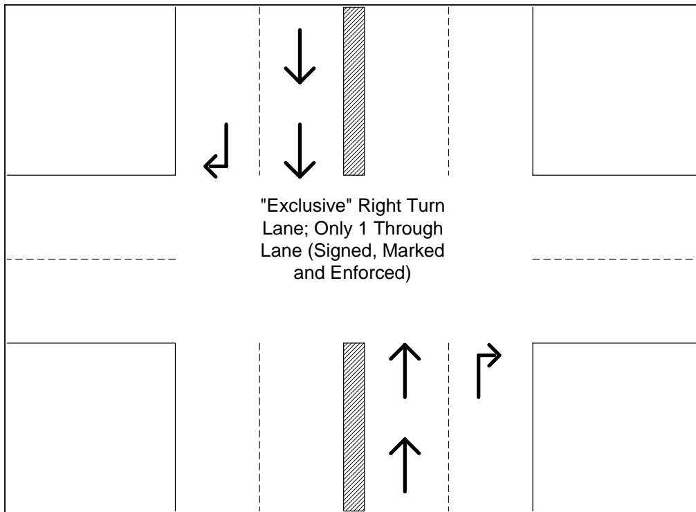
Figure IV-7. Exclusive Right Turn Lane
