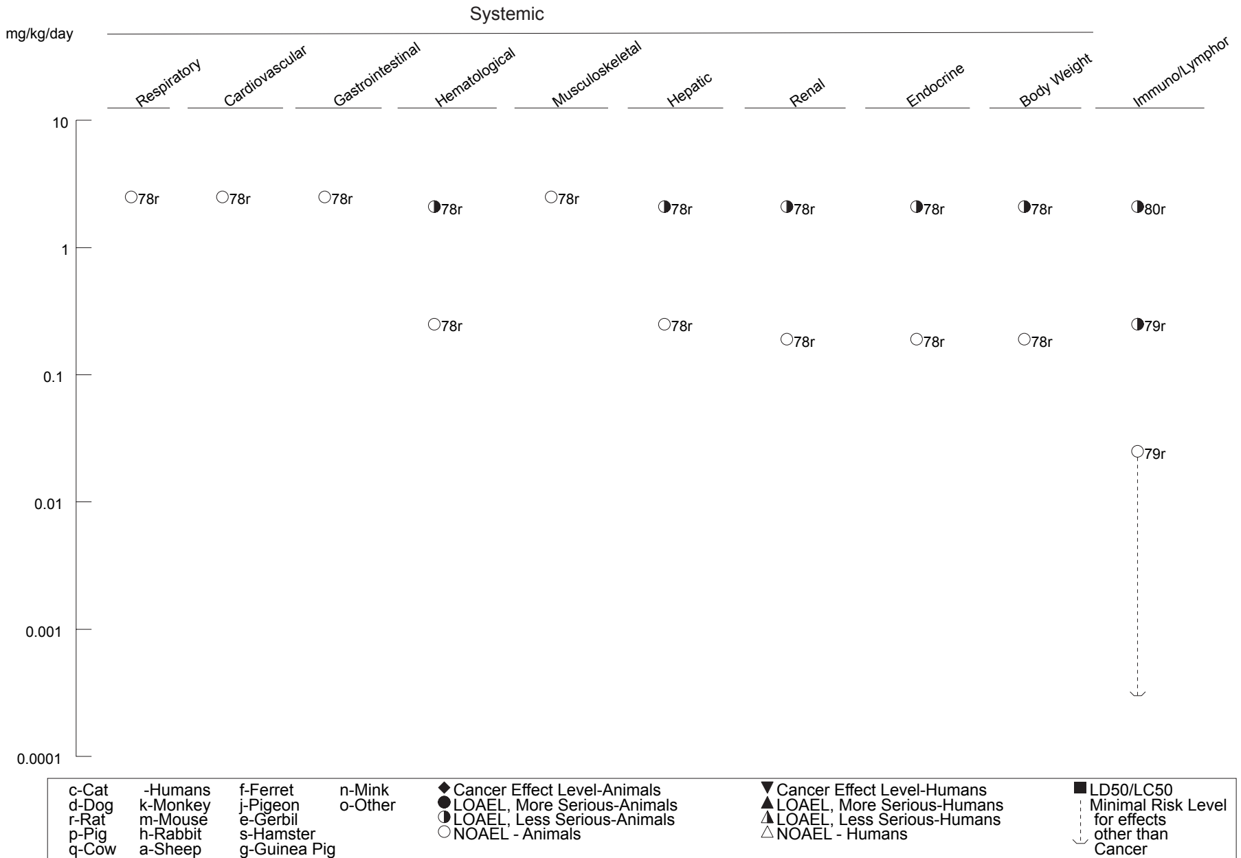
Figure 3-8 Levels of Significant Exposure to Tributyltins - Oral (Continued) Chronic (≥365 days)
