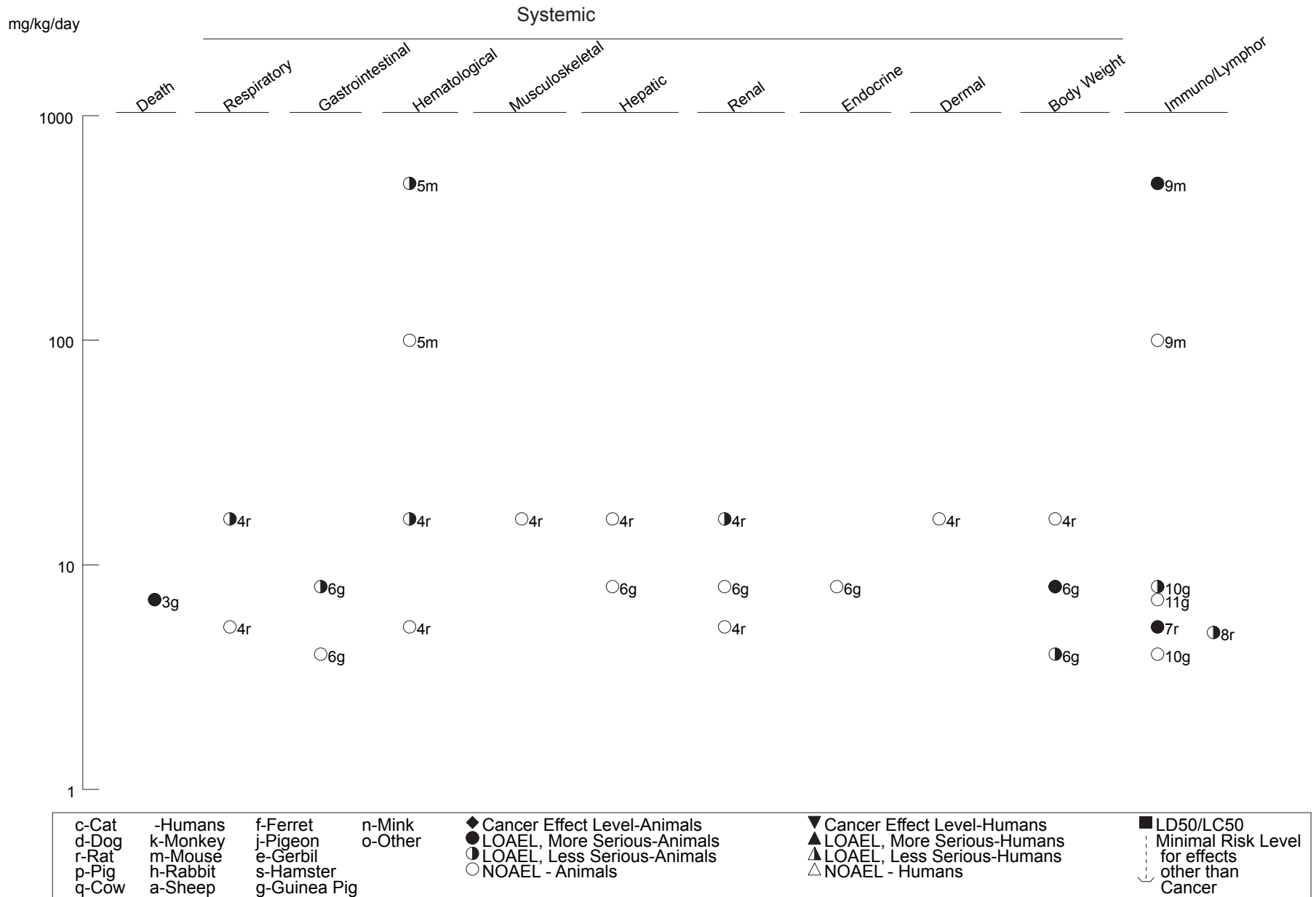
Figure 3-4 Levels of Significant Exposure to Dioclyltins - Oral (Continued) Intermediate (15-364 days)
