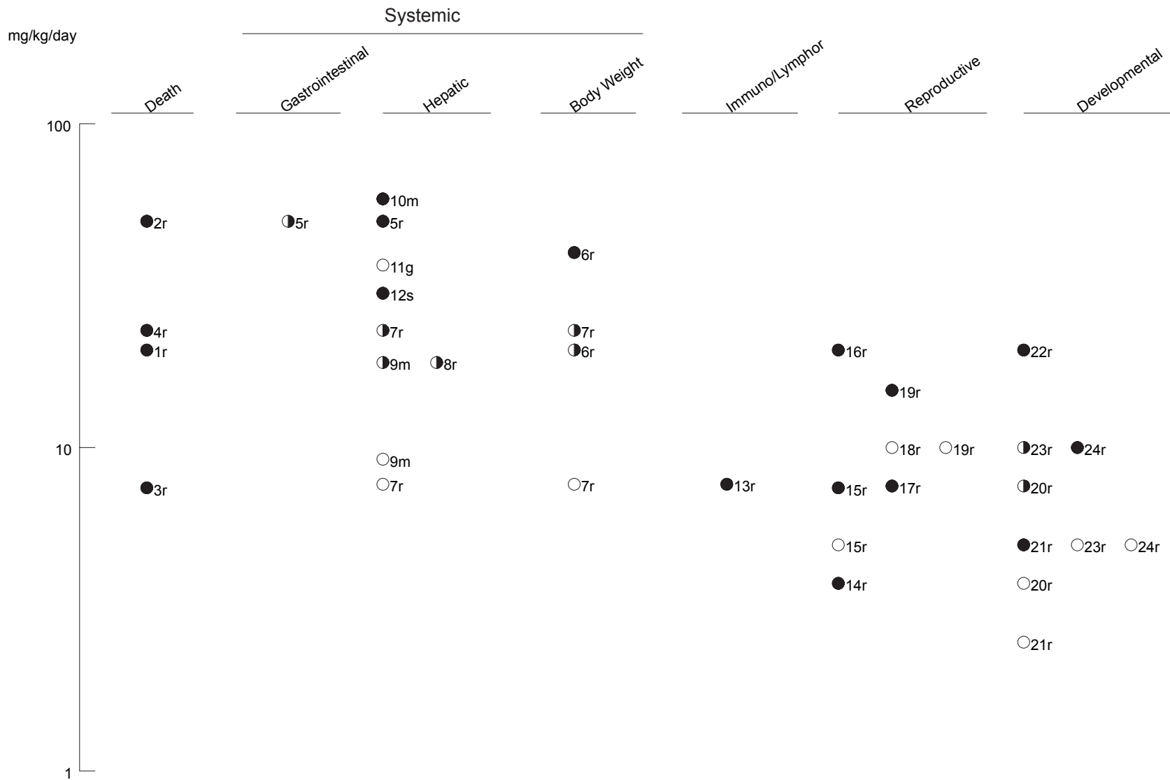
Figure 3-3 Levels of Significant Exposure to Dibutyltins - Oral Acute ( \leq 14 days)
