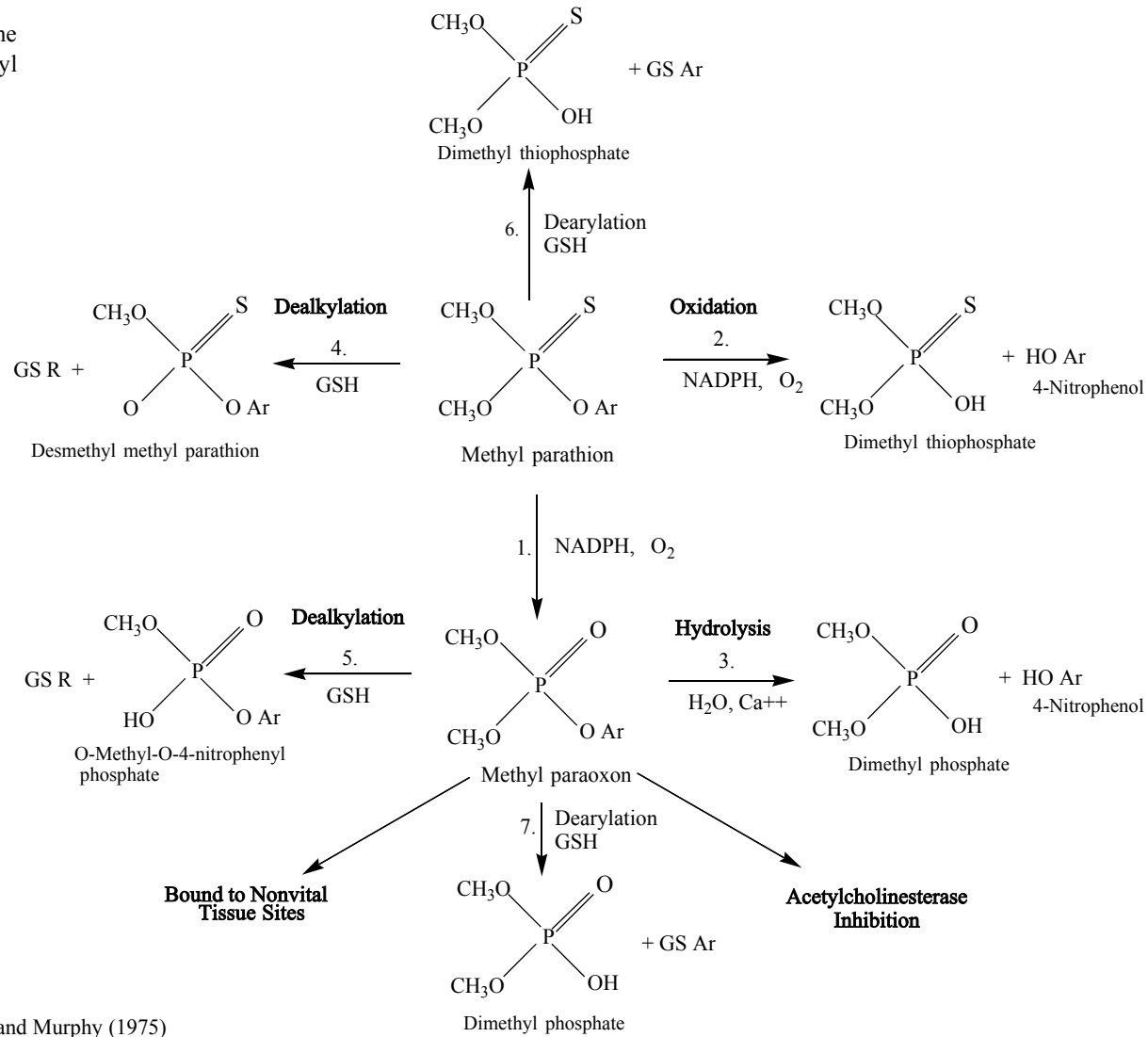
Figure 3-3. Proposed Metabolic Pathways of Methyl Parathion
