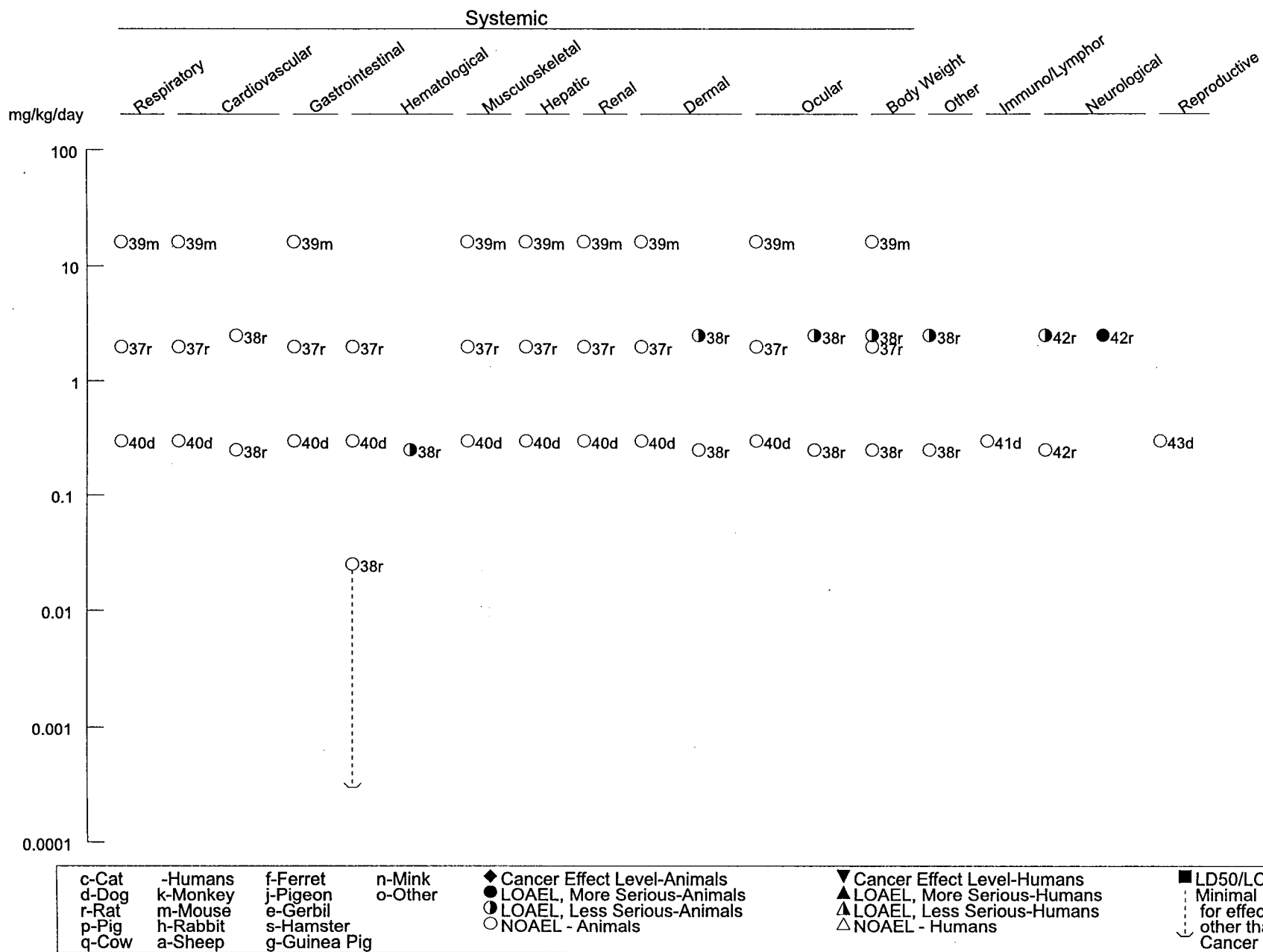
Figure 3-2. Levels of Significant Exposure to Methyl Parathion - Oral (continued) Chronic ( \geq 365 days)
