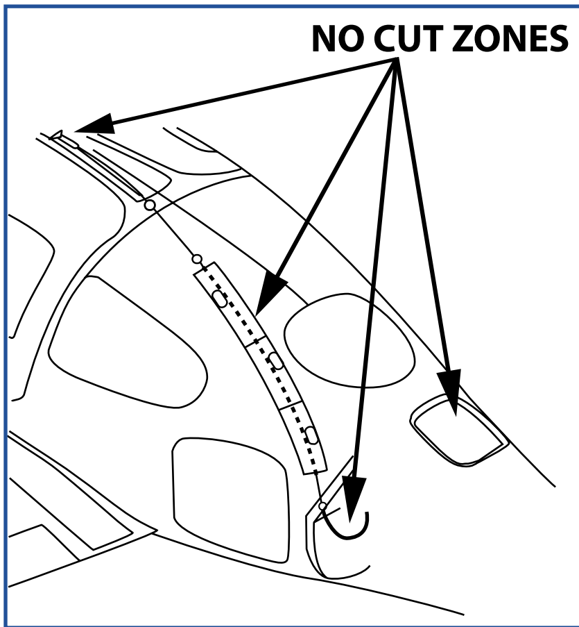
Above: A diagram of the No Cut Zones on Cirrus Design Aircraft. Page 27 Top: A diagram of the areas to stay clear when approaching a Ballistic parachute-equipped aircraft accident. Bottom: A ground extration test of the Cirrus Airframe Parachute System (CAPS). Illustrations courtesy of Cirrus Design, Air Safety Department.
