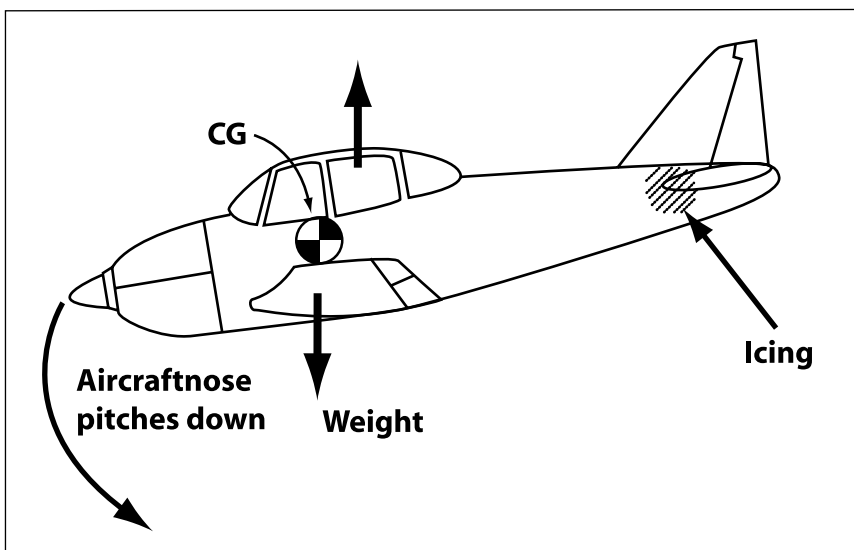
Figure 2. Pitchover due to tail stall
