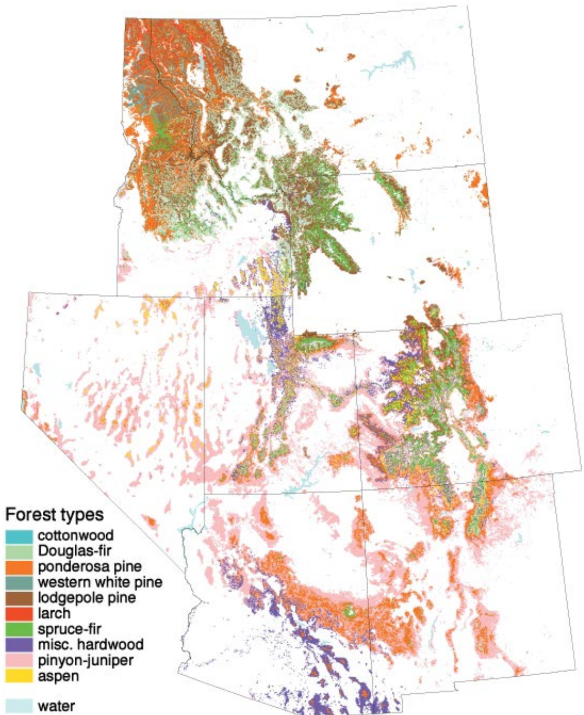
Figure 1—Map of regional forest types derived from satellite imagery at 1 km resolution in the early 1990s. Source: AVHRR satellite, USDA Forest Service, Southern Forest Experiment Station, Forest Inventory and Analysis.
