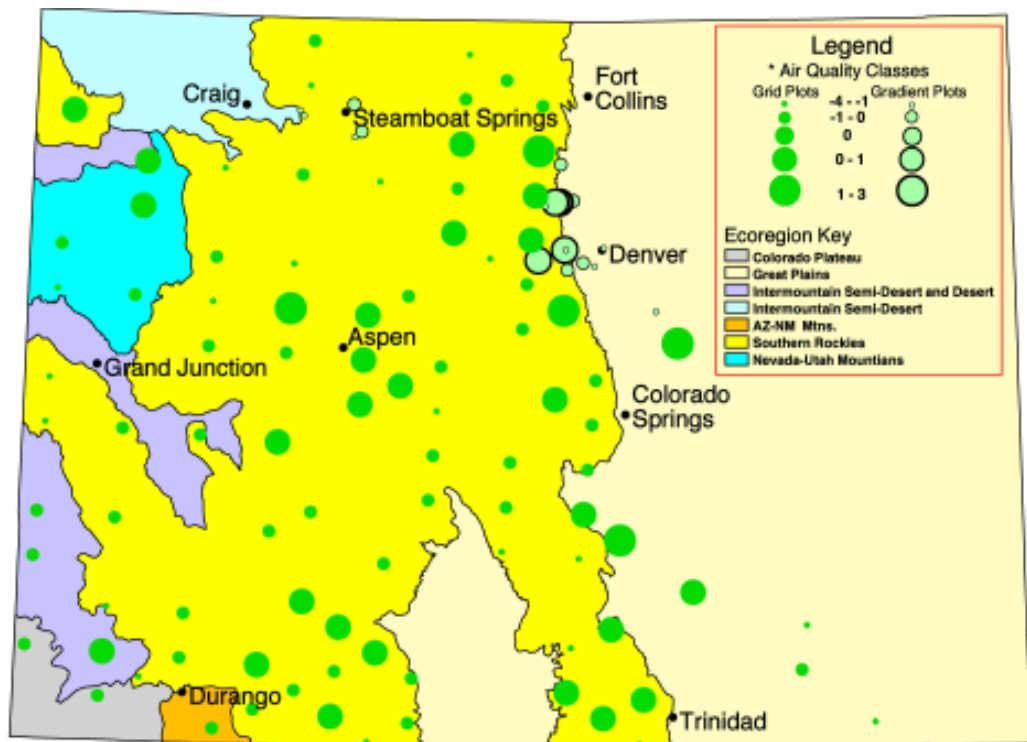
Figure 7 —The clustered (light green) circles represent gradient analysis sites where lichens were sampled in Colorado. The gradient is designed to assess relative tolerance of lichen species to varying levels of air pollution; hence, sites are located at intervals from known pollution sites to known good air quality sites. Lichen plots on the FHM grid (dark green) depict air quality based on the index developed for lichen species from the gradient. Larger circles represent higher air quality.
