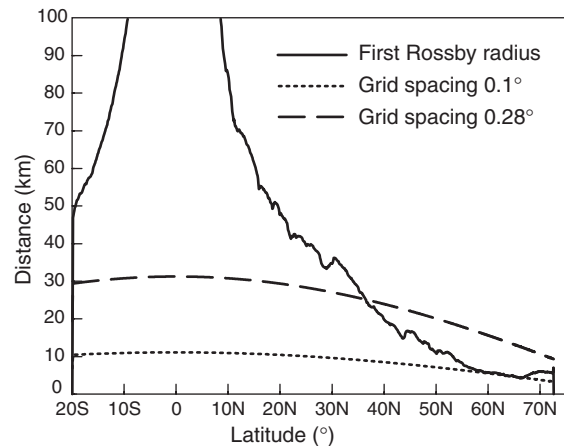
Figure A. Zonally Averaged Rossby Radius The zonally averaged Rossby radius is computed from the time-mean density of the 0.1^\circ North Atlantic POP simulation. This radius is compared with the grid spacing of the 0.1^\circ and 0.28^\circ POP models.
