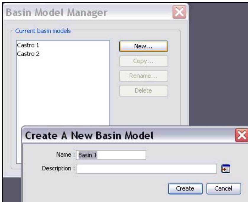
Figure 13. Create a new basin model.
