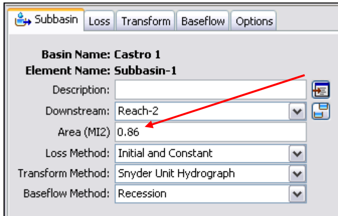
Figure 31. Subbasin area.
