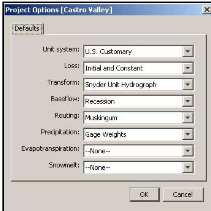
Figure 27. Setting the project options.
