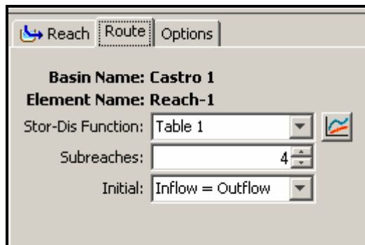
Figure 36. Modified Puls data for Reach-1.
