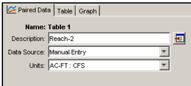
Figure 10. Component Editor for a storage-discharge function.
