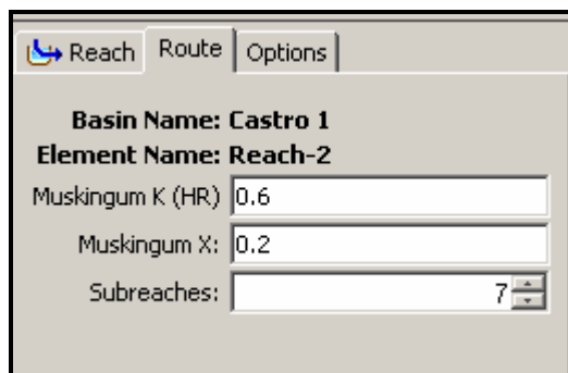
Figure 37. Muskingum data for Reach-2.
