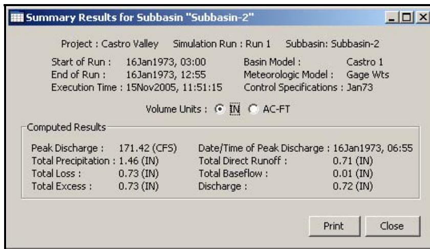
Figure 51. Summary table of Subbasin-2 results.
