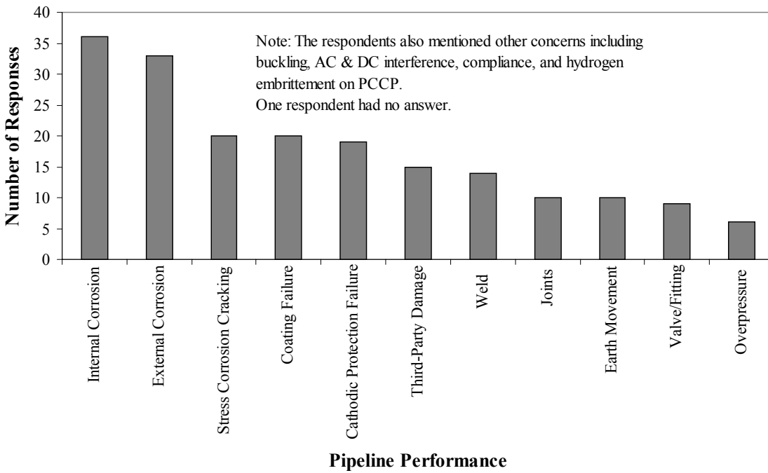
Figure VI.3: Companies Major Concerns for Pipeline Performance
