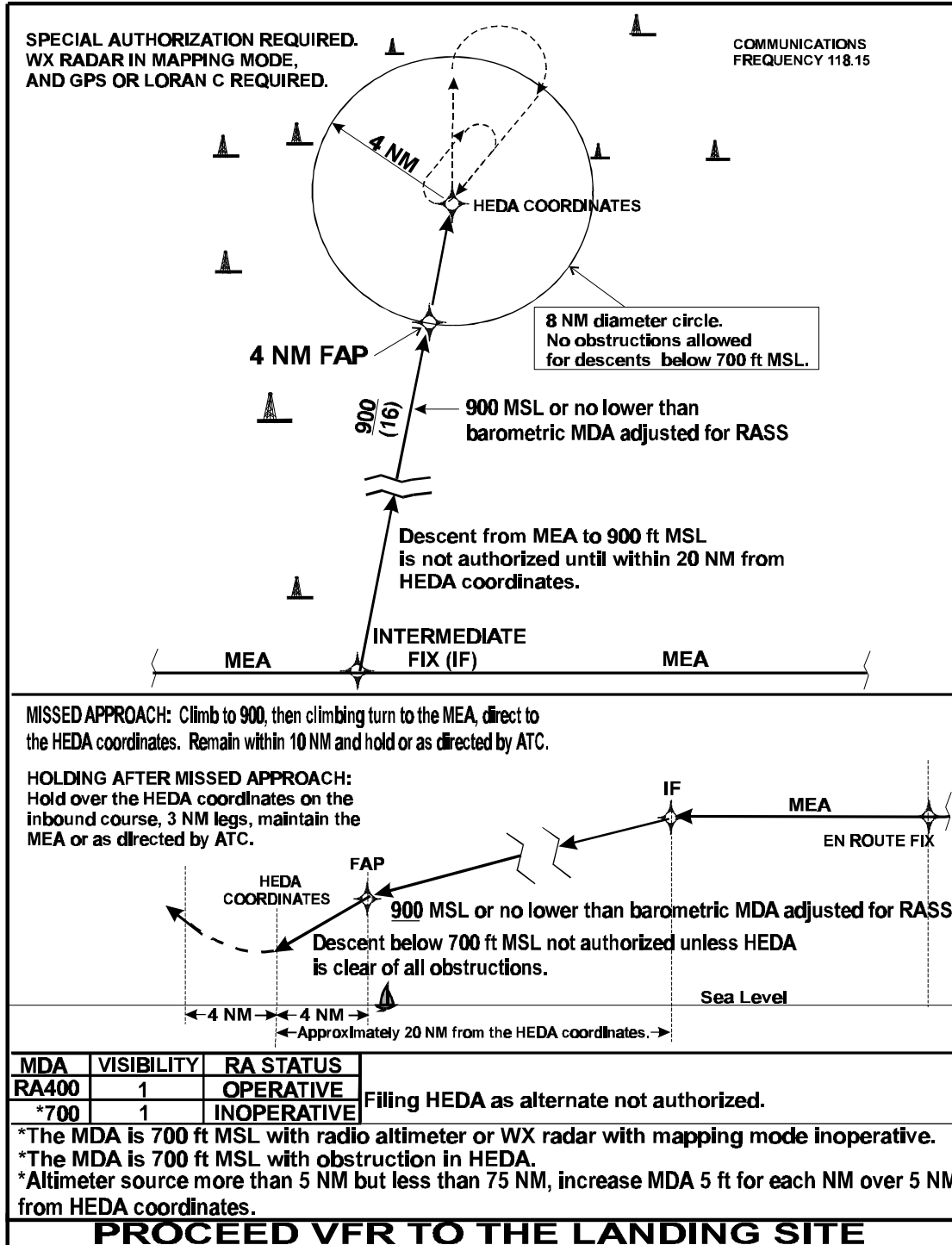
Figure 5-5. SAMPLE HEDA CHART.
