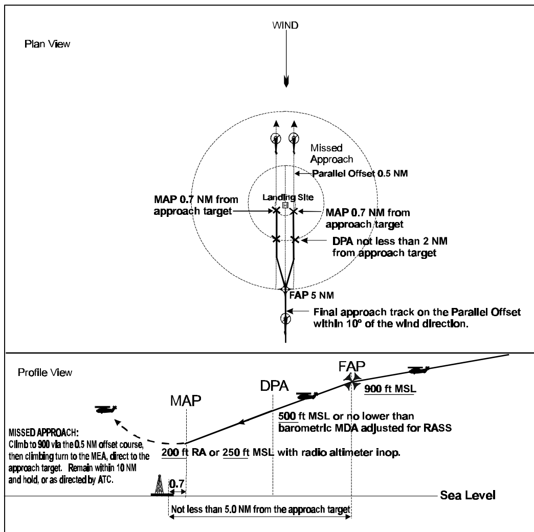
Figure 2-4. PARALLEL OFFSET OSAP
