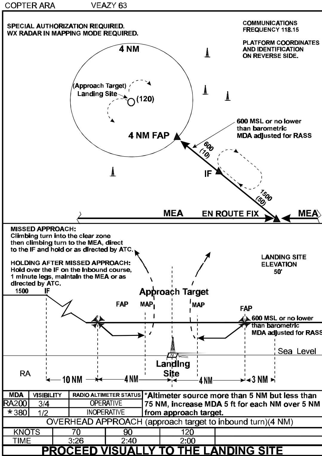
Figure 5-3. SAMPLE ARA CHART FOR SINGLE PLATFORM
