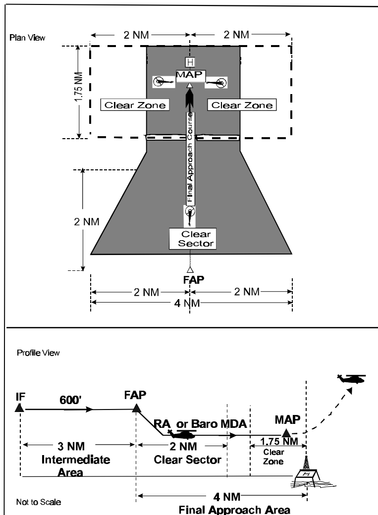
Figure 3-3. CLEAR ZONE AND CLEAR SECTOR
