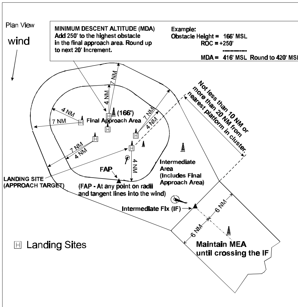
Figure 3-2. CLUSTER APPROACH TARGET AREA
