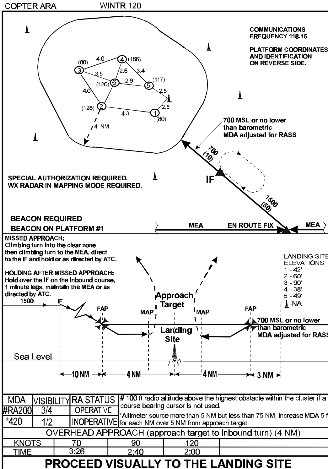
Figure 5-4. SAMPLE ARA CHART FOR PLATFORM CLUSTER.
