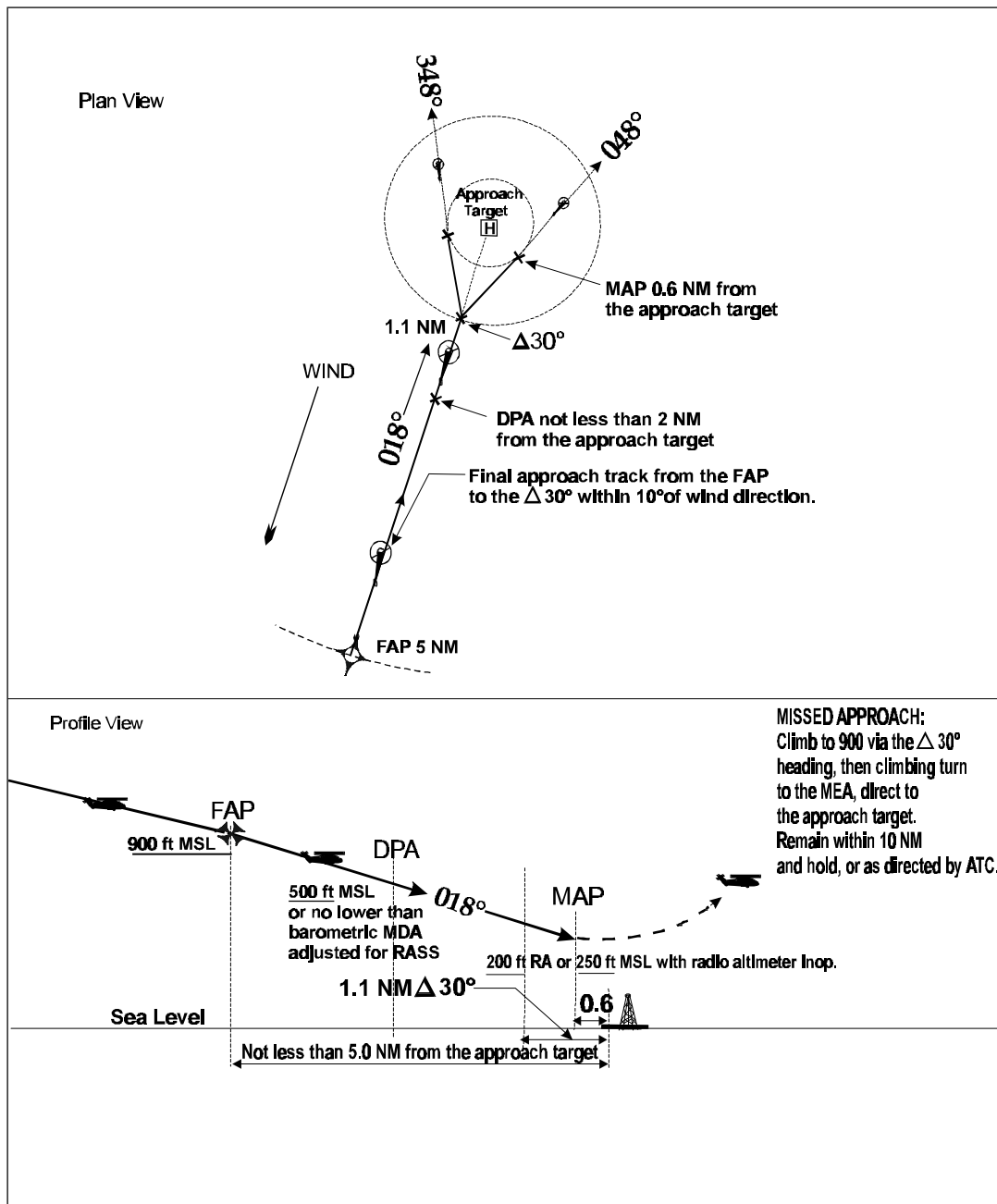
Figure 2-3. DELTA 30° OSAP
