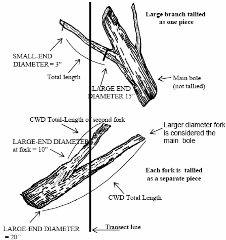
Figure 6-6: CWD tally rules for forked trees
