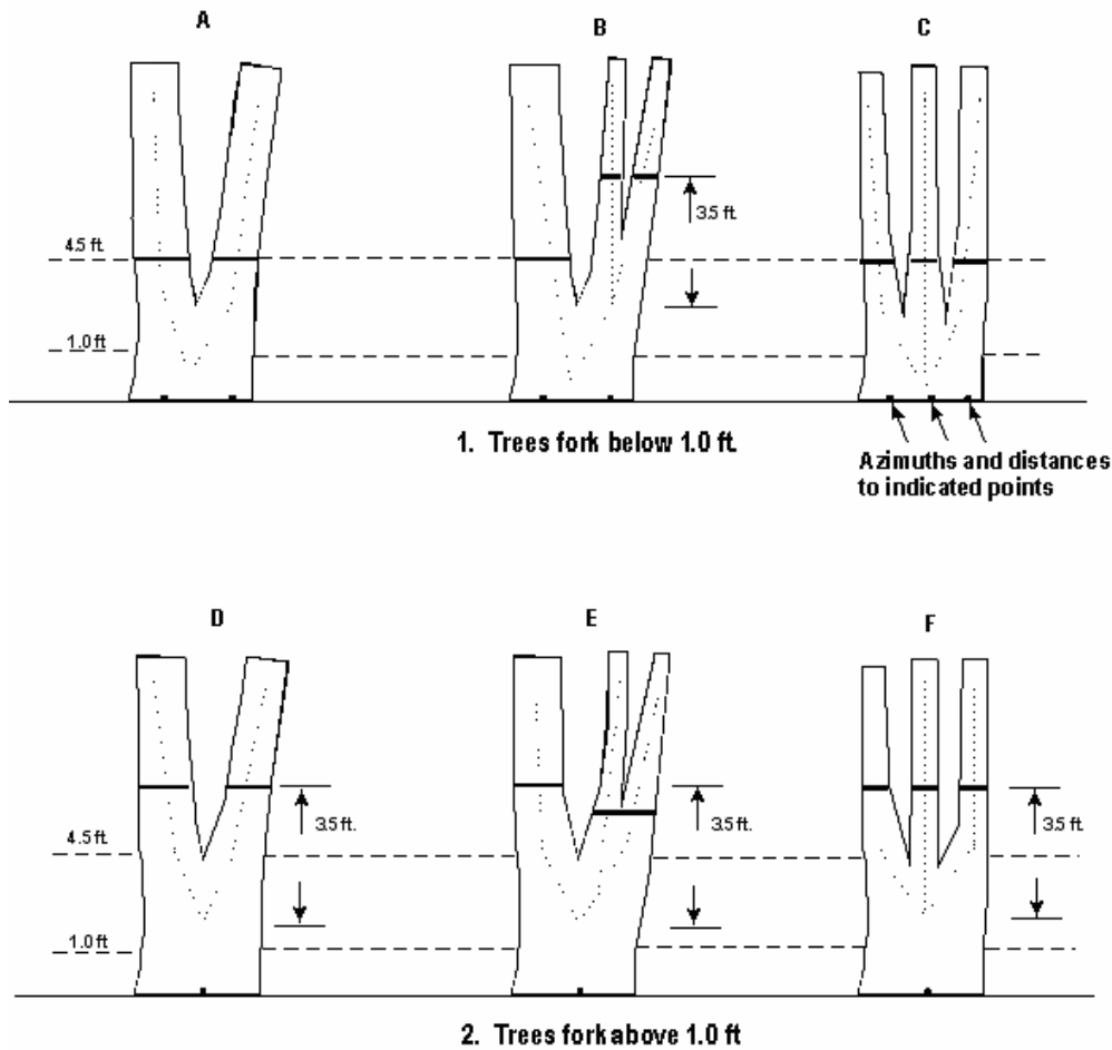
Figure 7-9: Summary of where to measure DBH, distance, and azimuth on forked trees.
