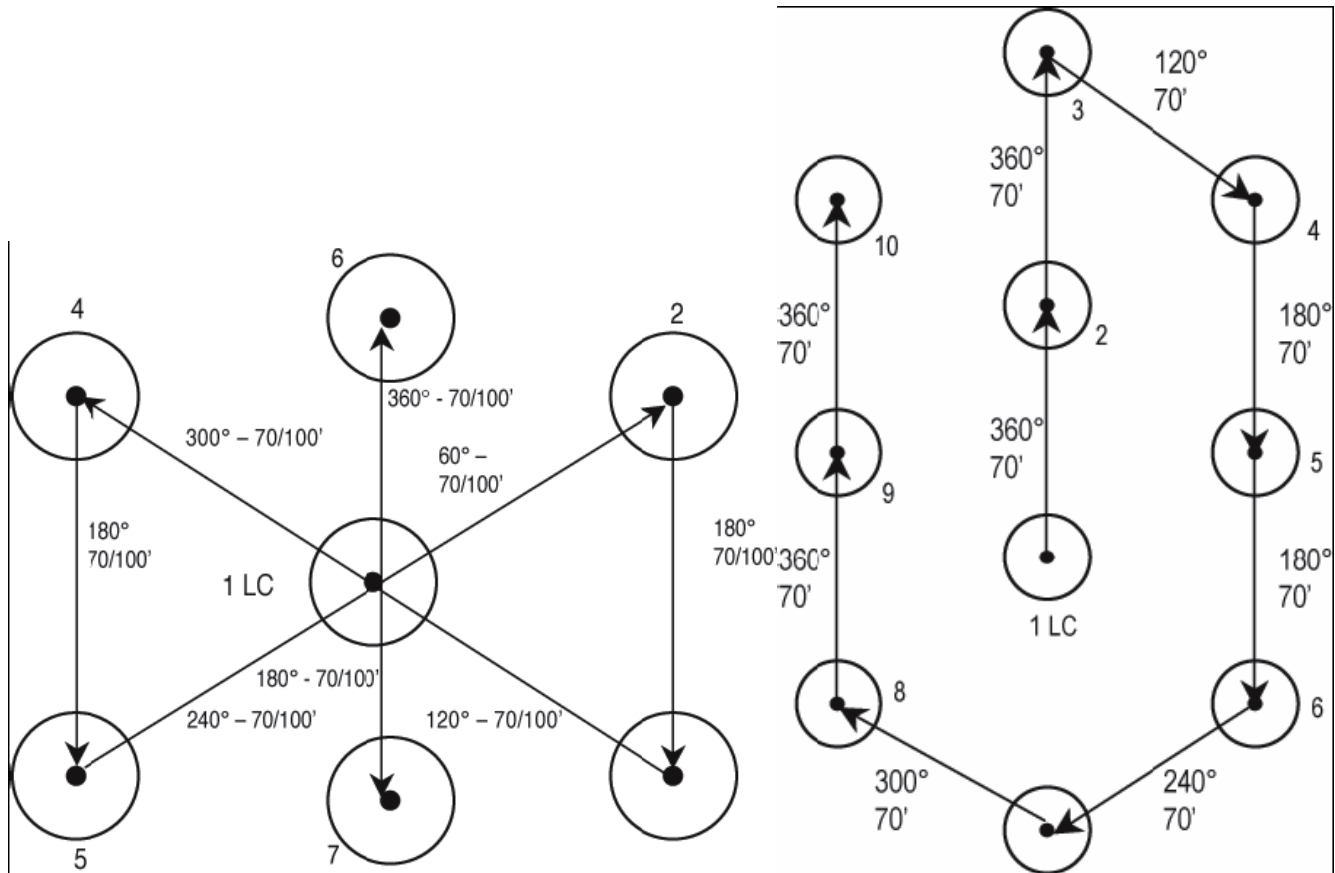
Figure A1-1. Previous variable-radius plot layouts.
