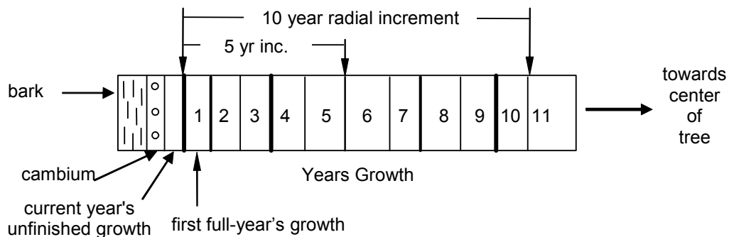
Figure 7-21: Bored tree core showing where to measure 5 and 10 year radial increments.
