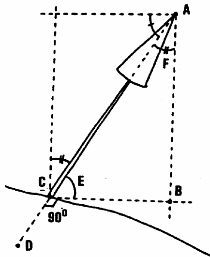
Figure 7-22: Measuring height of leaning tree.
