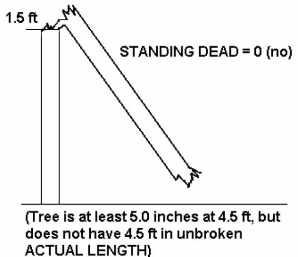
Figure 7-4: Example of an unbroken length of < 1.5 feet.
