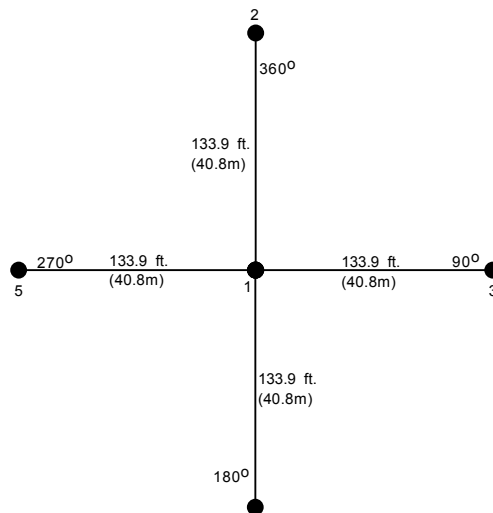
Figure A1-3: Locating stake positions 1-5 (Distance and cardinal directions from stake position 1)
