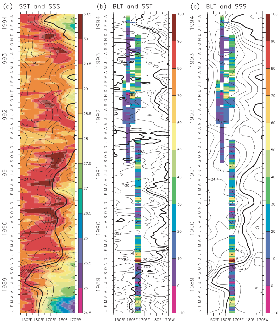
Figure 2. (a) Reynolds and Smith [1994] sea surface temperature (SST) (shaded) and Delcroix et al. [2000] gridded sea surface salinity (SSS) (contoured). (b) Smoothed 15-day barrier layer thickness (BLT) computed from moored data (pixel time series, in units of meters) and Reynolds and Smith SST (contoured). (c) BLT (pixel time series) and gridded SSS (contoured). SST contour interval (CI) is 0.5°C and dark contour is 29.0°C; SSS CI is 0.2 psu and dark contour is 35.0 psu.
