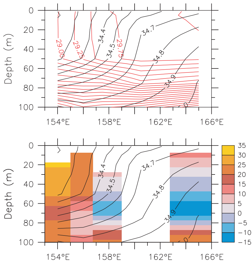
Figure 6. Time-averaged zonal-depth sections between 0^\circ , 154^\circ\text{E} and 0^\circ , 165^\circ\text{E} for 27 October to 1 November 1992. (top) Subsurface temperature (red contours; CI is 0.25^\circ\text{C} ) and subsurface salinity (black contours; CI is 0.1 psu). (bottom) Zonal currents (shaded, in units of centimeters per second) and subsurface salinity (black contours; CI is 0.1 psu).
