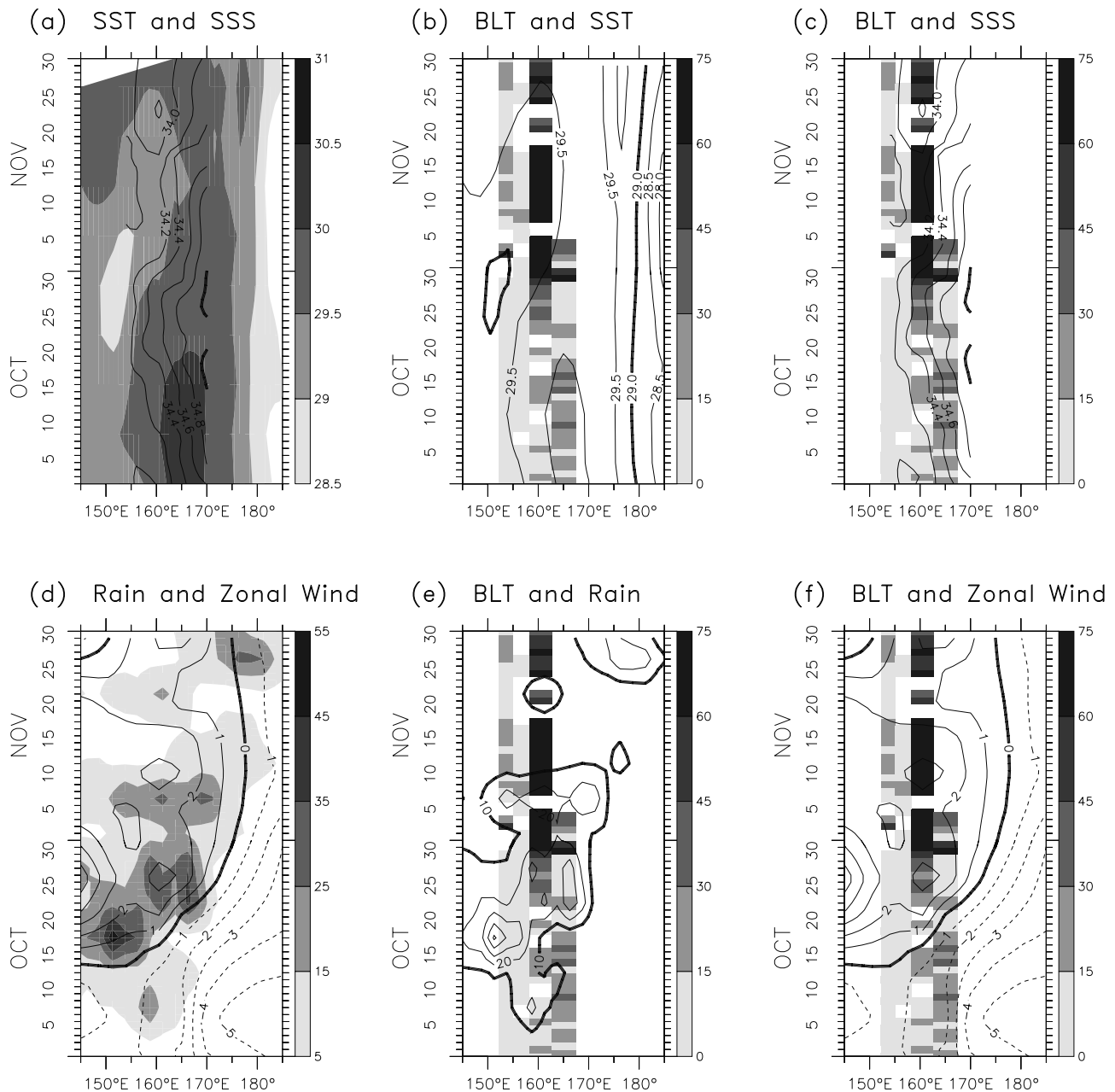
Figure 5. Surface fields along the equator during October and November 1992. (a) Reynolds and Smith [1994] SST (shaded) and SSS from moorings along the equator at 154°E, 156°E, 160.5°E, 165°E, and 170°E (contoured). (b) BLT and Reynolds and Smith SST. (c) BLT and moored SSS. (d) Xie and Arkin [1997] pentad rainfall rates (shaded) and TAO gridded zonal winds (contoured). (e) BLT and Xie and Arkin rainfall rates. (f) BLT and TAO zonal winds. SST CI is 0.5°C and dark contour is 29.0°C. SSS CI is 0.2 psu and dark contour is 35.0 psu. Only positive BLT values are shown. Zonal wind CI is 1 m s -1 , westerly winds are solid lines, easterly winds are dashed lines, and the zero contour is dark. Rain rate CI is 10 mm d -1 and dark contour is 10 mm d -1 .
