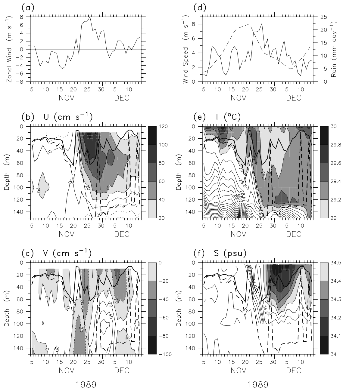
Figure 4. Moored 0^\circ , 165^\circ\text{E} daily averaged time series from 5 November 1989 through 14 December 1989: (a) zonal wind (in units of meters per second); (b) zonal velocity (CI is 20\text{ cm s}^{-1} , eastward flow above 20\text{ cm s}^{-1} shaded); (c) meridional velocity (CI is 20\text{ cm s}^{-1} , southward flow shaded); (d) wind speed (solid line, in units of meters per second); (e) temperature (CI is 0.2^\circ\text{C} , temperatures higher than 29^\circ\text{C} shaded); and (f) salinity (CI is 0.1\text{ psu} , salinity less than 34.5\text{ psu} shaded). Mixed layer depth (thick solid line) and isothermal mixed layer depth (thick dashed line) as defined by (5)–(6) are superimposed on Figures 4b–4c and 4e–4f. The Xie and Arkin [1997] pentad rain rate at 0^\circ , 165^\circ\text{E} (in units of millimeters per day) is shown as a dashed line in Figure 4d.
