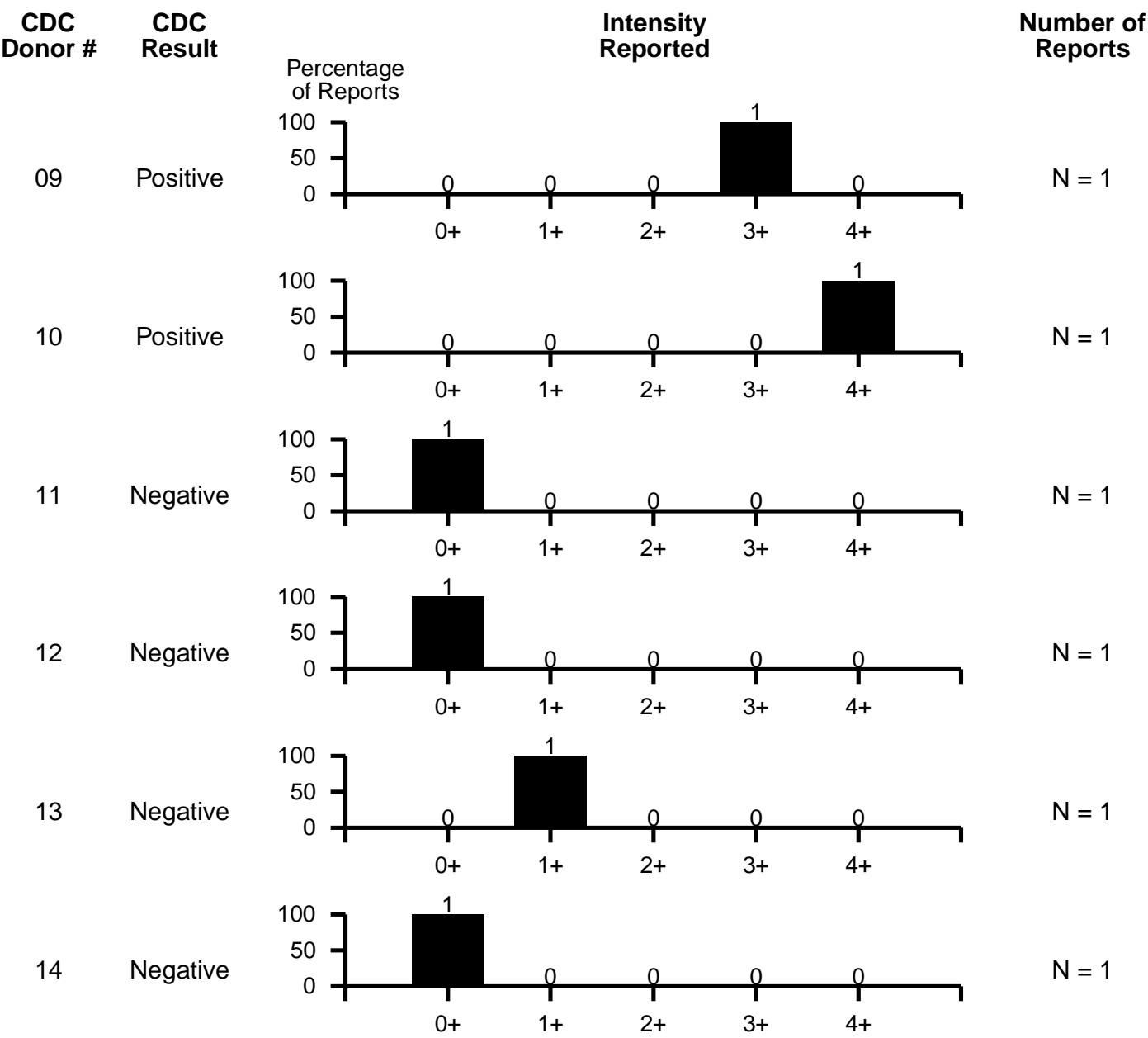
Figure 9. Fluorescence intensity patterns, of HTLV-I/II-infected cells, for IIF results reported to CDC by participant laboratories for the May 20, 1996 shipment
