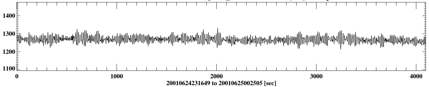
df07202200106242316 1 sec = dt, y range: 1213.8 - 1330.3 [cm], 4096 points
