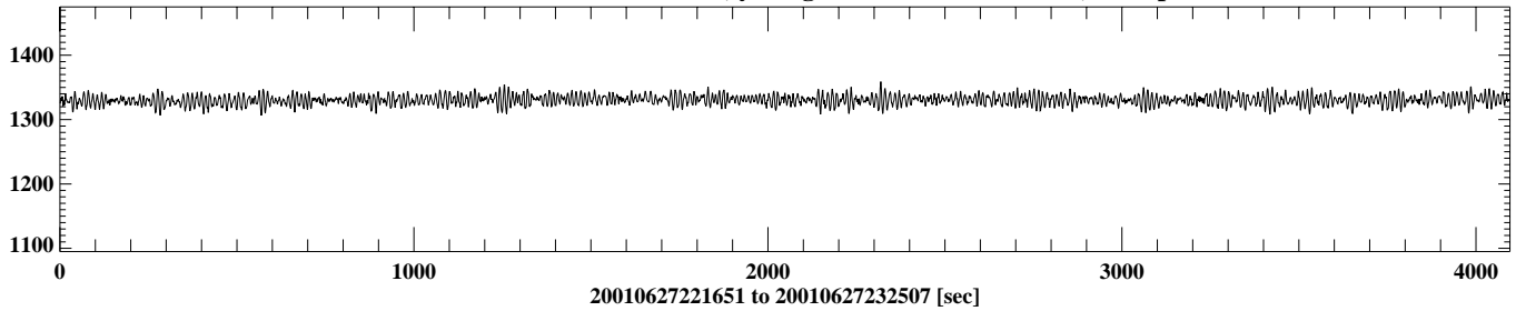
df07202200106272316 1 sec = dt, y range: 1300.3 - 1351.6 [cm], 4096 points
