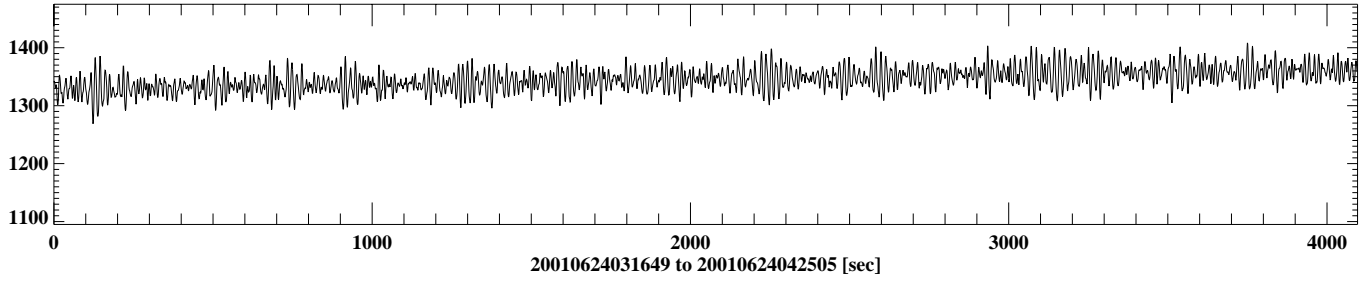
df07202200106240416 1 sec = dt, y range: 1319.6 - 1436.2 [cm], 4096 points
