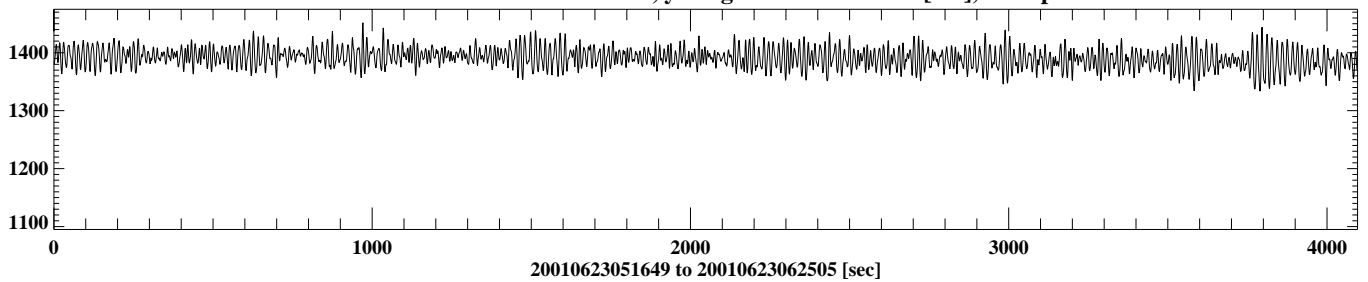
df07202200106230516 1 sec = dt, y range: 1333.7 - 1451.7 [cm], 4096 points
