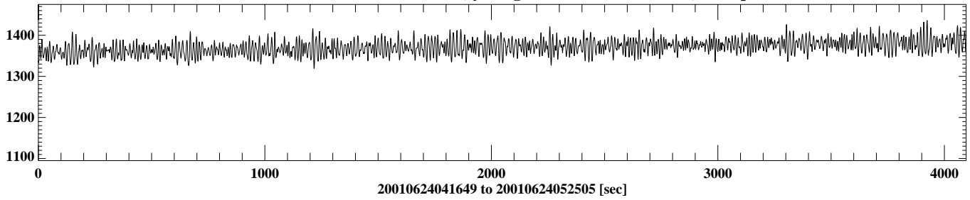
df07202200106240516 1 sec = dt, y range: 1333.5 - 1457.9 [cm], 4096 points
