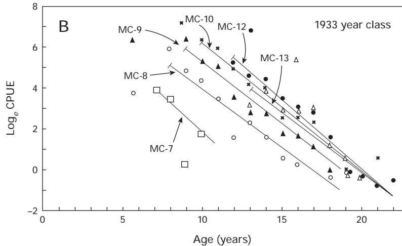
Figure 17. A: Frequency distribution (per mille) of maturation cohorts (MC) of Northeast Arctic cod (1925-30 year classes; shaded area) and Norwegian spring-spawning herring (1933-37 year classes; unshaded area) at maturation. B: Log e CPUE vs. age of the maturation cohorts of the 1933 year class of Northeast Arctic cod.
