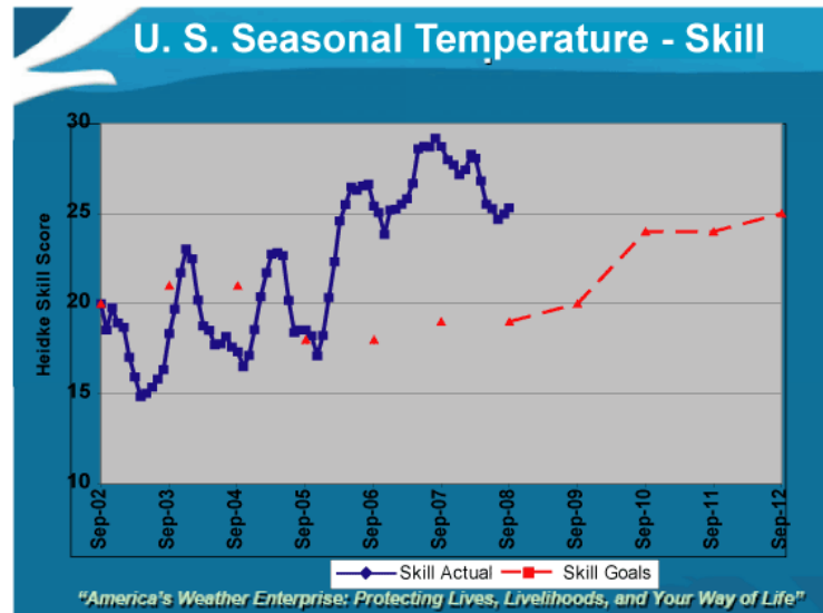
Fig. 3. 48-month running mean of the Heidke skill score of real-time, operational \frac{1}{2} -month lead 3-month temperature outlooks from September 2002 through September 2008 (blue line) (GPRA score). The red line is the GPRA goal.
