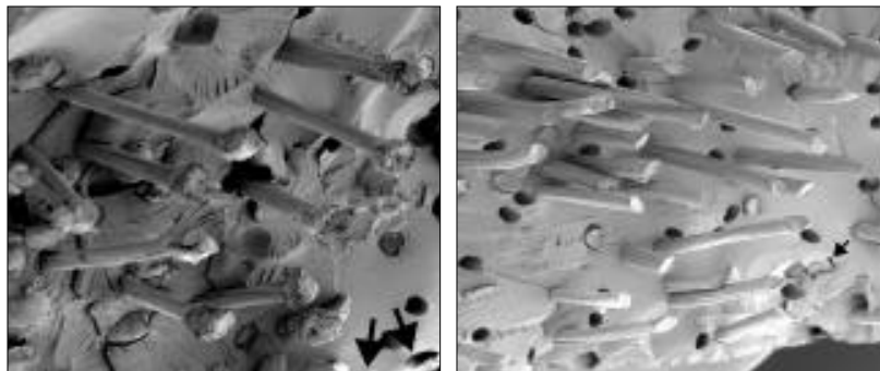
Highly magnified images of fracture surfaces of a bone-shaped short fiber composite (left) and a conventional short straight fiber composite.
