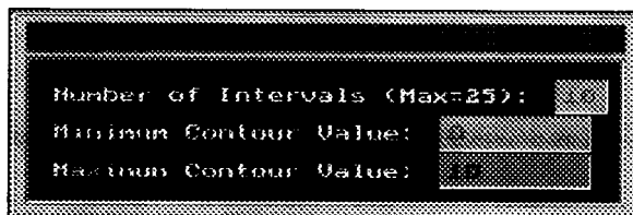
Figure 40. Contour Descriptors
