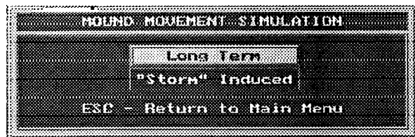
Figure 29. Mound Movement Simulation
