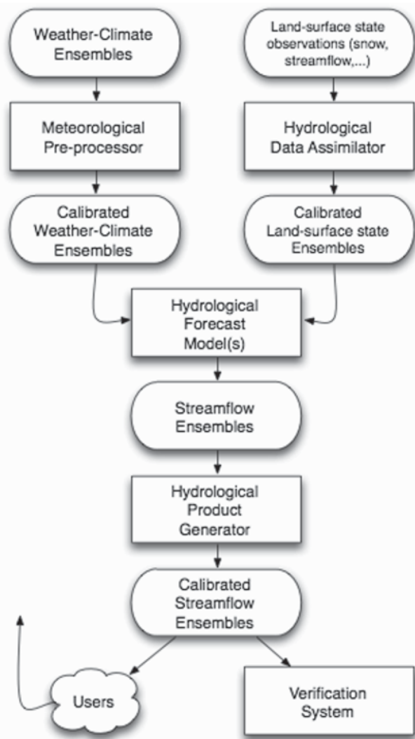
FIG. 1. Schematic of the components and information flow in an ensemble hydrological prediction system.
