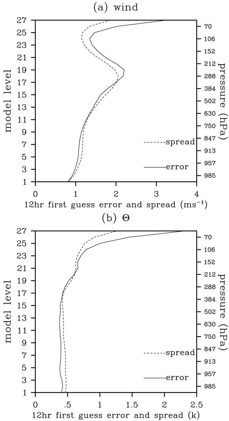
Figure 8. The ETKF ensemble spread (dotted) and the rms first guess error (solid) as a function of model levels for the hybrid with simulated observation up to 100 hPa, ensemble size 50, 1/\beta_1 = 0.2 , and S_e = 1414 \text{ km} . (a) wind, (b) potential temperature.
