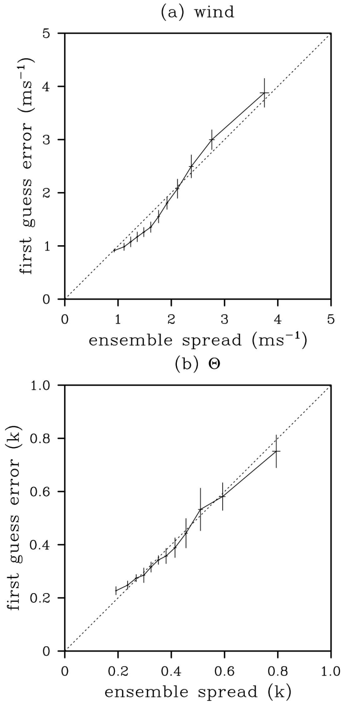
Figure 9. Second-order measure (see details in the text) of the skill of the ETKF ensemble spread for model level 17 of Fig. 8. (a) wind, (b) potential temperature.
