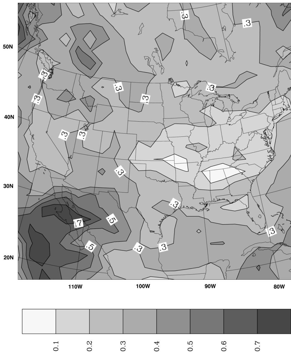
Figure 5. The difference of the root-mean-square vertically averaged wind analysis error between the hybrid (ensemble size 50, 1/\beta_1 = 0.2 , and S_e = 1414\text{km} ) and the 3DVAR for the verification domain. Positive values mean the hybrid analysis was more accurate than the 3DVAR.
