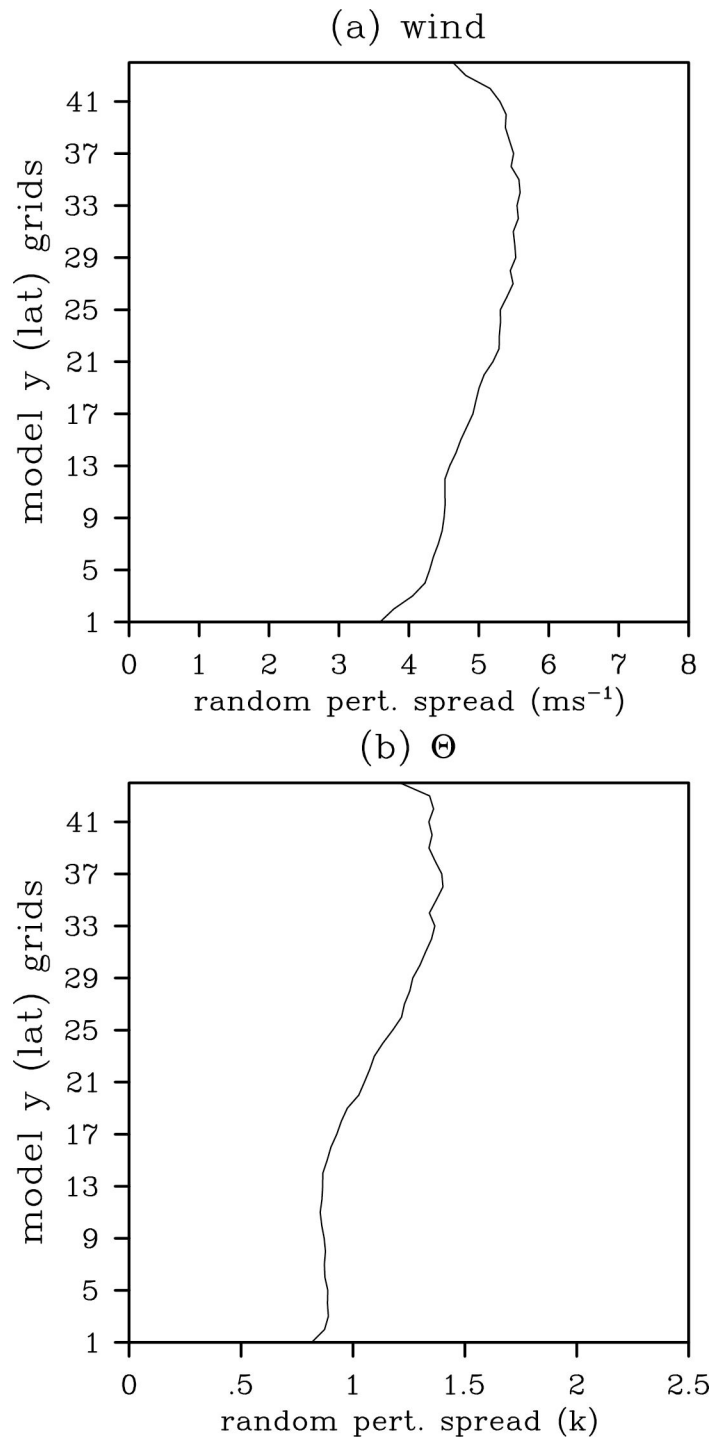
Figure 3. Zonally averaged spread of 50 random perturbations drawn from the WRF 3DVAR NCEP background error covariance for (a) wind ( \sqrt{U^2 + V^2} ) and (b) potential temperature.
