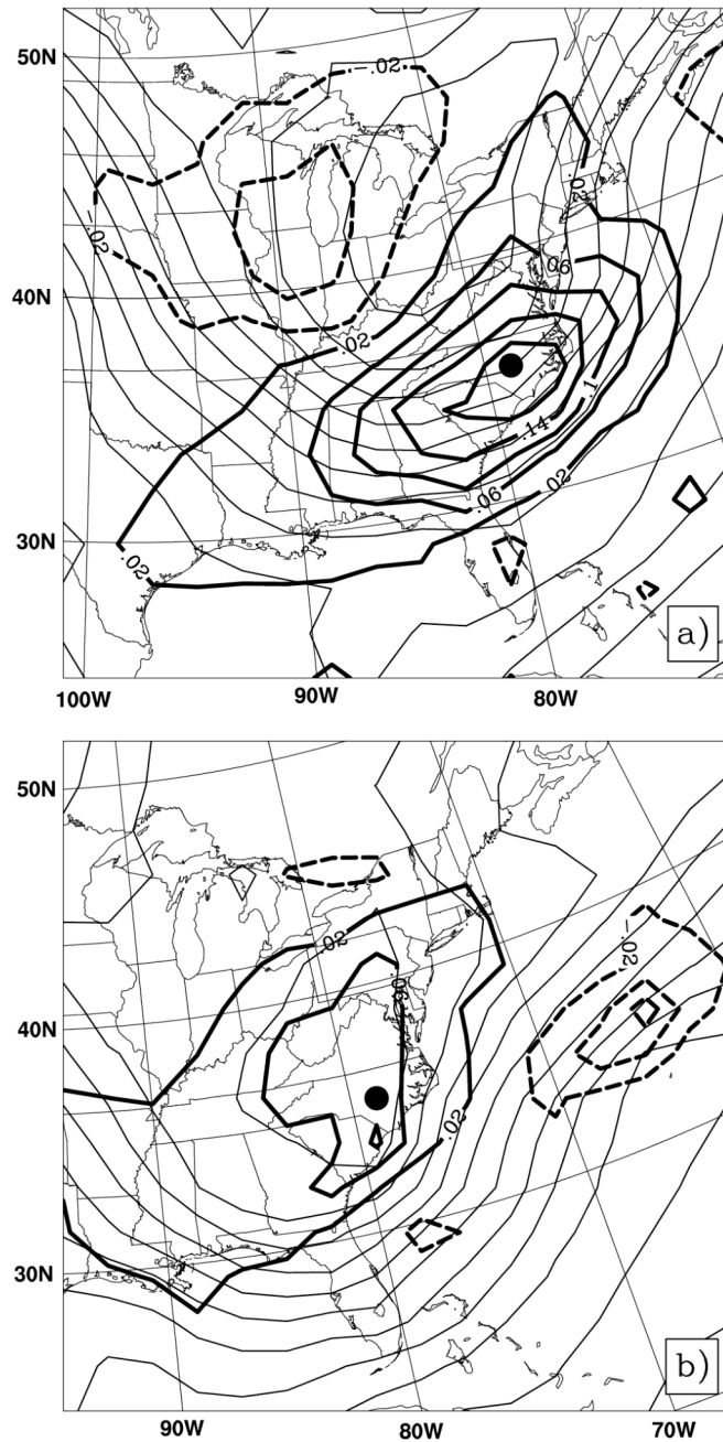
Figure 4. 850 hPa temperature increment by assimilating a single observation of 850 hPa temperature at the black dot using localized ETKF ensemble covariance only. The observation was 1 degree warmer than the background forecast. Thin black contours are 850 hPa temperature from -21 to 15 degrees with contour interval of 3 degrees. The thick black contours are the temperature increments with a 0.04 degrees contour interval. (a) a case at 0000 UTC 14 January 2003. (b) a case at 0000 UTC 24 January 2003.
