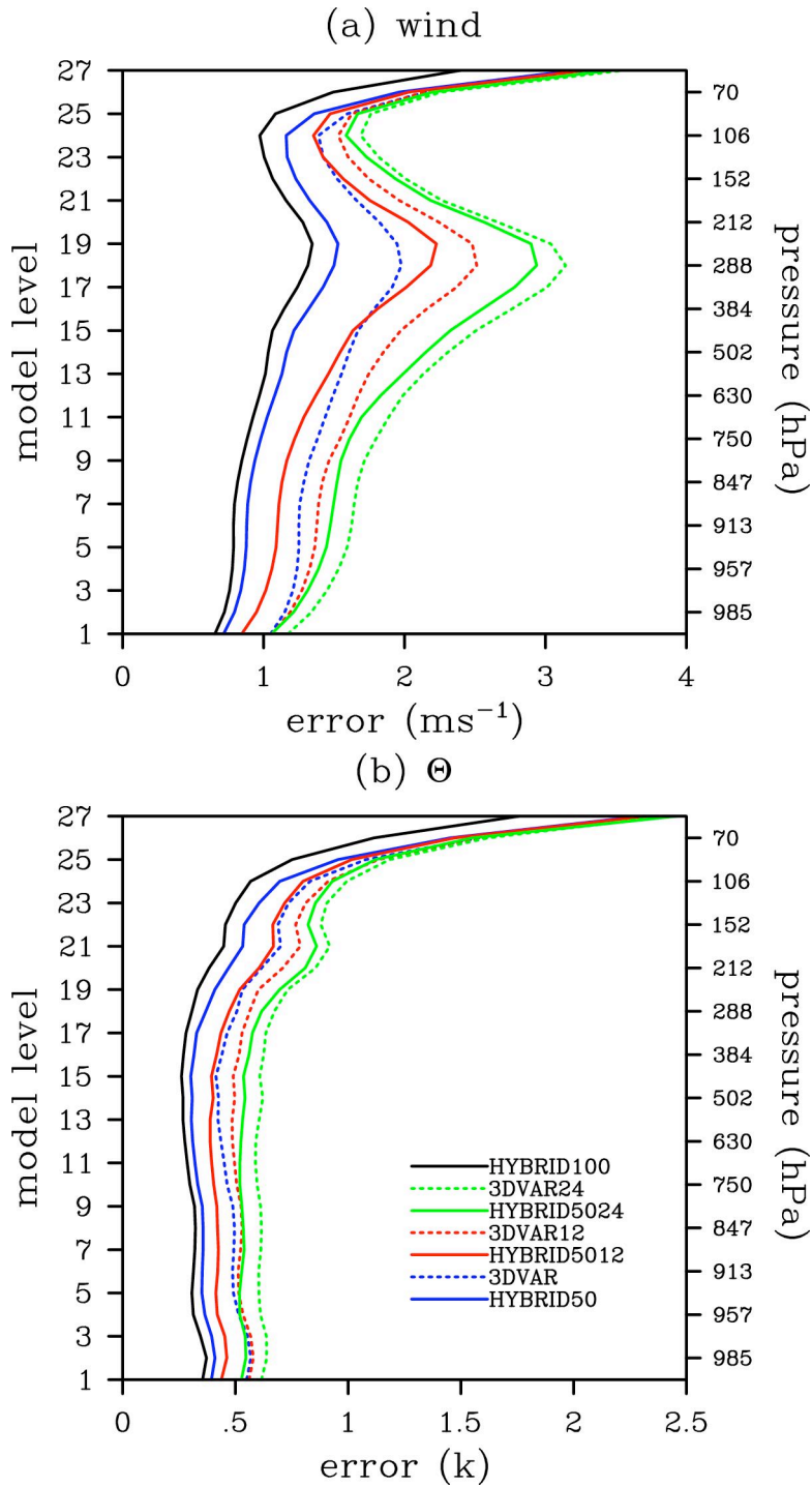
Figure 6. Vertical profiles (as a function of model eta levels) of the analysis errors (blue), 12-hour (red) and 24-hour (green) forecast errors for the 3DVAR (dotted) and the hybrid with ensemble size 50, 1/\beta_1 = 0.2 , and S_e = 1414\text{km} (solid). The analysis error for the hybrid with ensemble size 100, 1/\beta_1 = 0.2 , and S_e = 1414\text{km} is in black. (a) wind. (b) potential temperature. The pressure on the right axis was calculated from the eta values, model top pressure of 50 hPa and approximated surface pressure of 1000 hPa.
