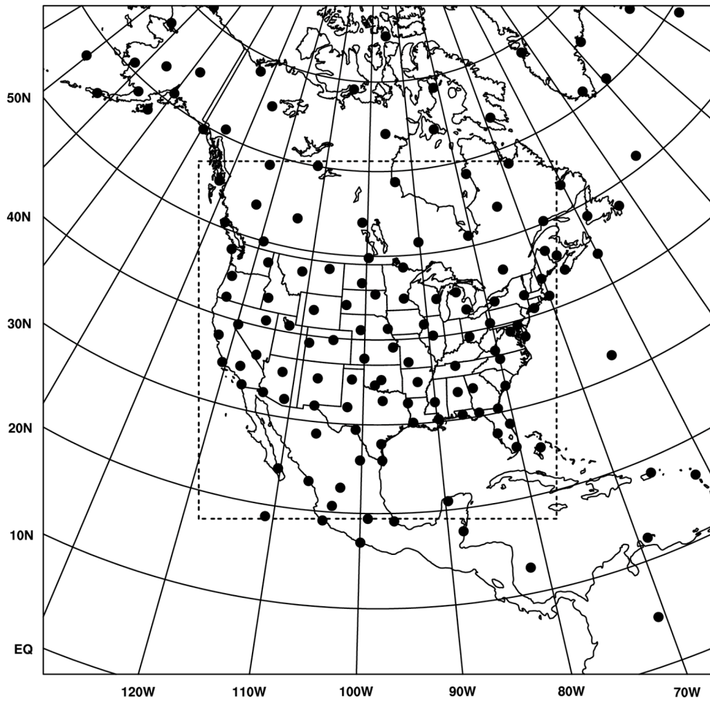
Figure 1. The WRF domain (full grid), the verification region (inner box), and a snapshot of radiosonde network at 1200 UTC 8 January 2003 (black dots).
