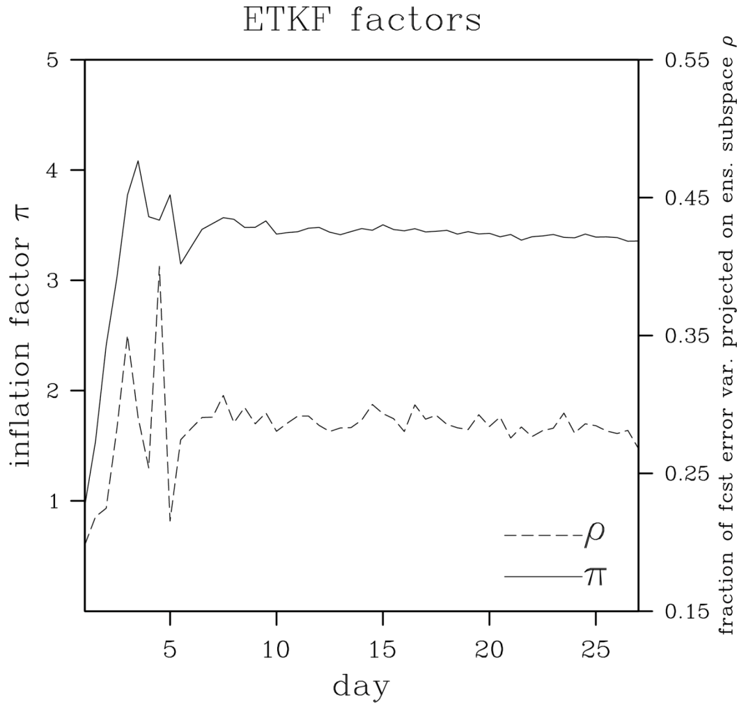
Figure 7. The inflation factor ( \Pi ) and the factor ( \rho ) of percentage projection of the first guess error variance onto the ensemble subspace for the ETKF in the hybrid experiment with 1/\beta_1=0.2 and S_e=1414km .
