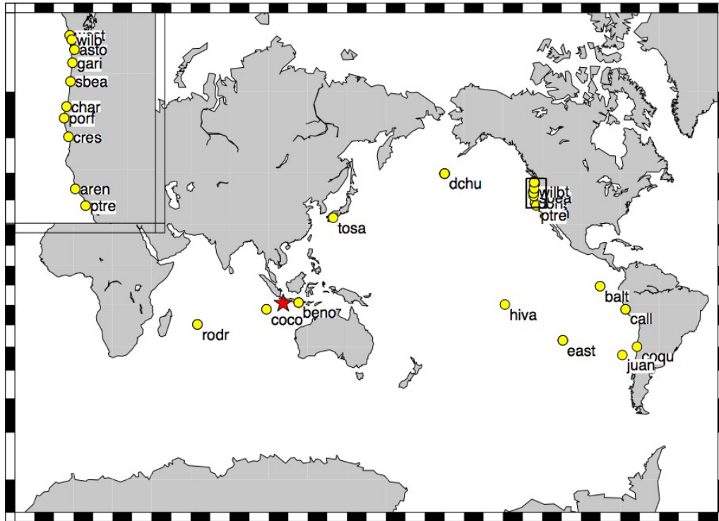
Figure 1 Stations recording sea level data (yellow dots) and epicenter of July 17, 2006 earthquake (red star). Enlarged view of northern US coast in top left corner.
