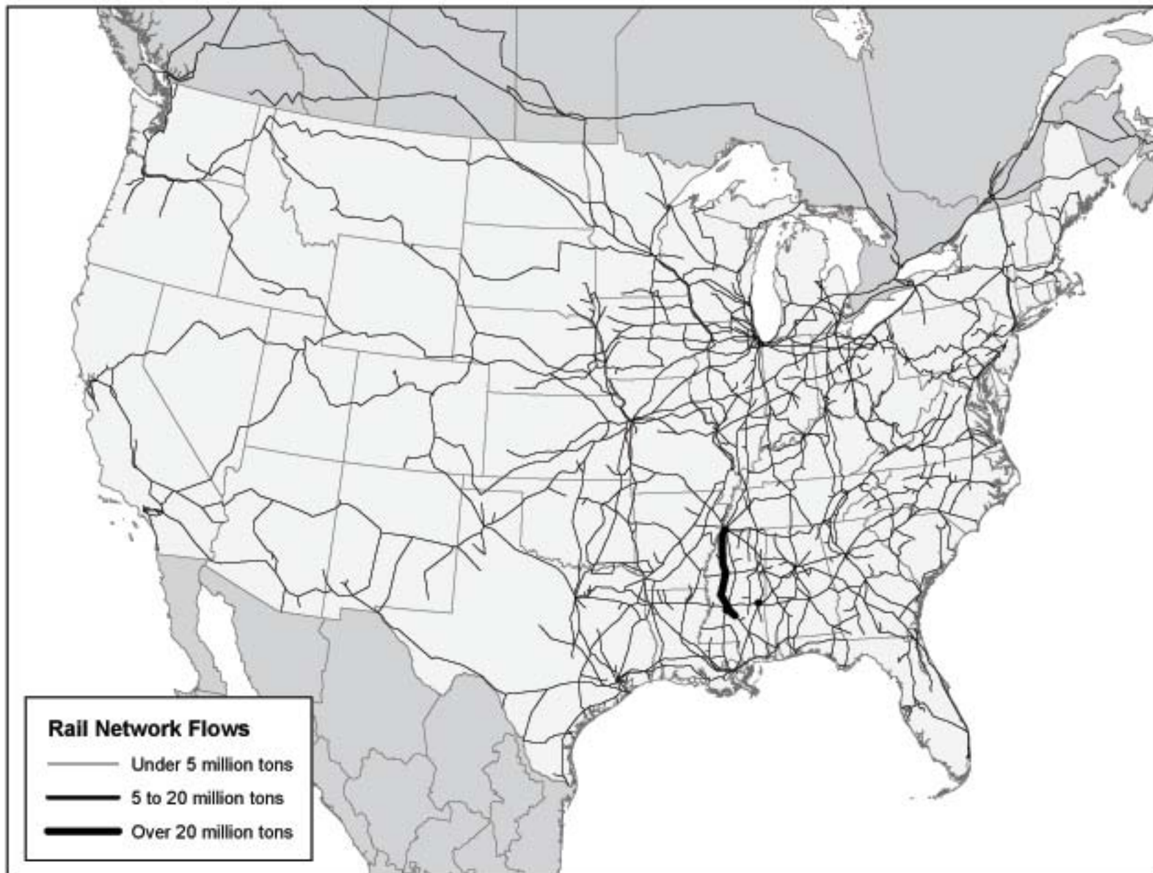
Map 3-2: Mississippi Total Rail Flows: 1999
