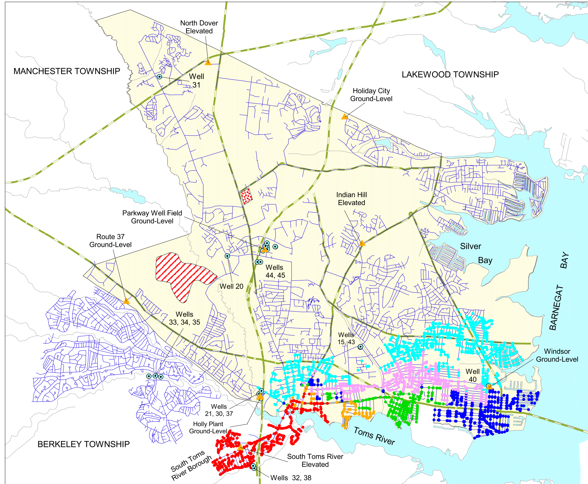
PLATE 14. AREAL DISTRIBUTION OF SIMULATED PROPORTIONATE CONTRIBUTION OF WATER FROM THE SOUTH TOMS RIVER WELL (32) TO LOCATIONS IN THE DOVER TOWNSHIP AREA, NEW JERSEY MARCH 1998 CONDITIONS By Morris L. Maslia, Jason B. Sautner, and Mustafa M. Aral
