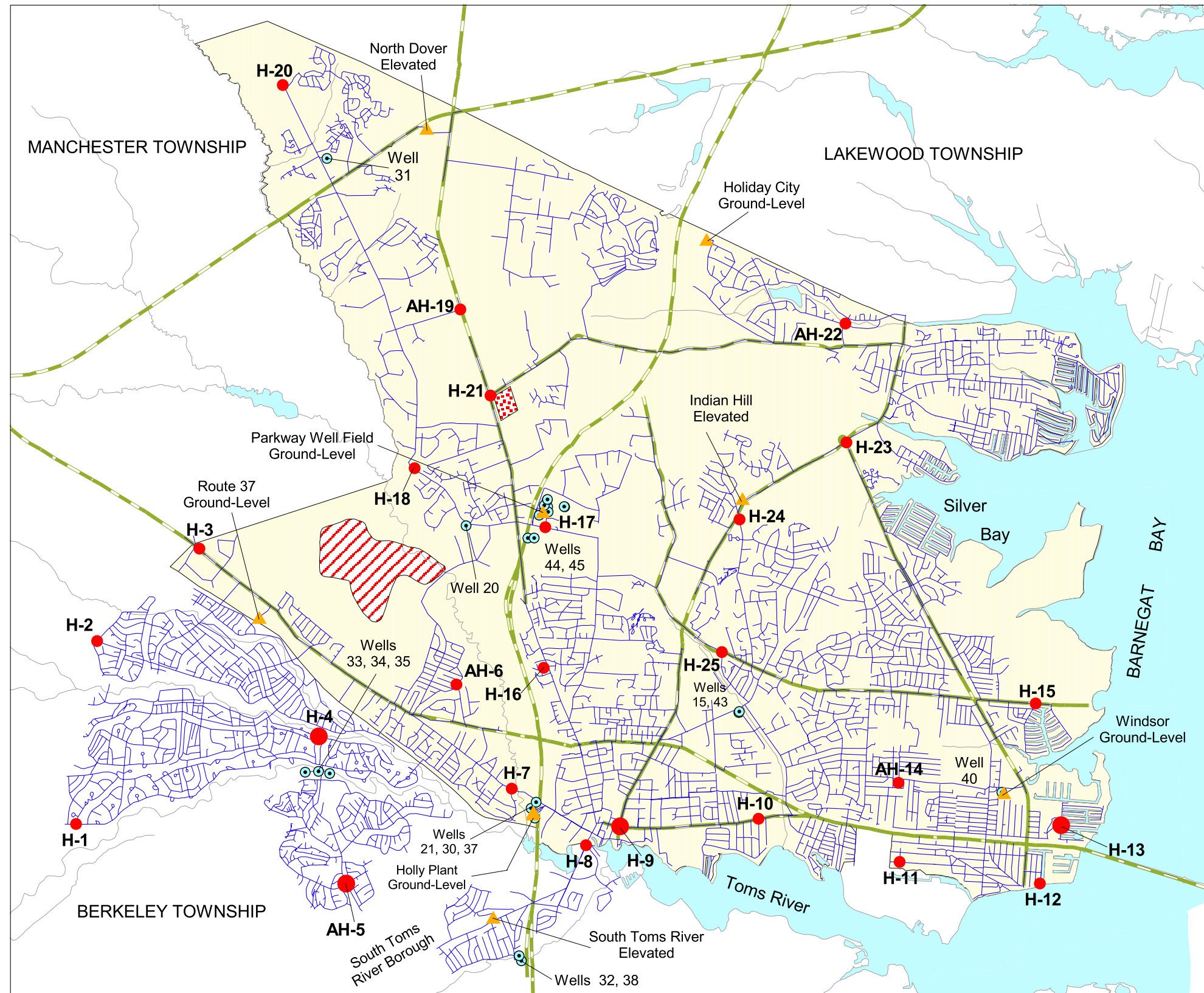
PLATE 11. AREAL DISTRIBUTION OF MEAN ABSOLUTE PRESSURE DIFFERENCE BETWEEN AUGUST 1998 TEST DATA AND SIMULATION, DOVER TOWNSHIP AREA, NEW JERSEY
