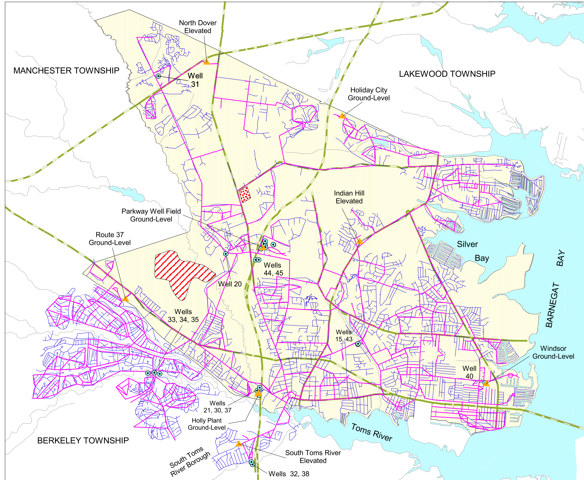
PLATE 3. EQUIVALENT HYDRAULIC NETWORK USED FOR INITIAL SIMULATION OF THE WATER-DISTRIBUTION SYSTEM SERVING THE DOVER TOWNSHIP AREA, NEW JERSEY
