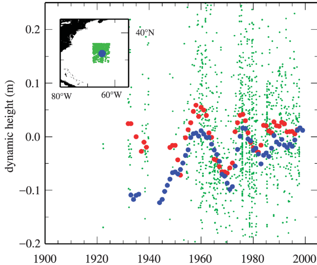
Figure 9. Comparison of GIA-corrected Bermuda tide-gauge time series (blue) and surface dynamic heights (green) computed from hydrographic data in 6 \times 6^\circ box centred on Bermuda. The red dots are dynamic heights smoothed with a 5 year running mean filter, as was the tide-gauge data.
