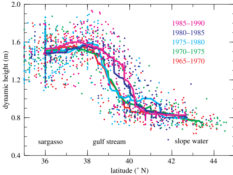
Figure 7. Surface dynamic height (0–1000 m) observations between 60 and 70 W plotted as a function of latitude, crossing the Gulf Stream just north of Bermuda (36N). Coloured dots and lines show actual measurements and the mean profile for each 5 year interval between 1965 and 1990.
