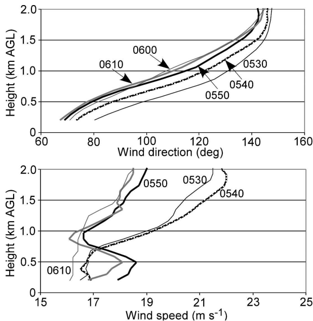
FIG. 13. Vertical profiles of (top) wind direction and (bottom) wind speed, based on 10-min averages from the 915-MHz profiler, for the stable offshore flow regime within the leading stratiform band from 0530 to 0610 UTC.
