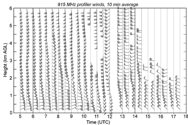
FIG. 5. Wind profiles derived from the 915-MHz profiler based on 10-min averages plotted every 30 min. A full wind barb represents 5 \text{ m s}^{-1} , and a flag represents 25 \text{ m s}^{-1} . The wind center passed over the MIPS site at about 1215 UTC.
