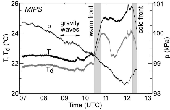
FIG. 11. MIPS surface parameters for the 0700–1300 UTC period. Frontal boundaries are depicted by the gray shading. Data frequency is 1 Hz.
