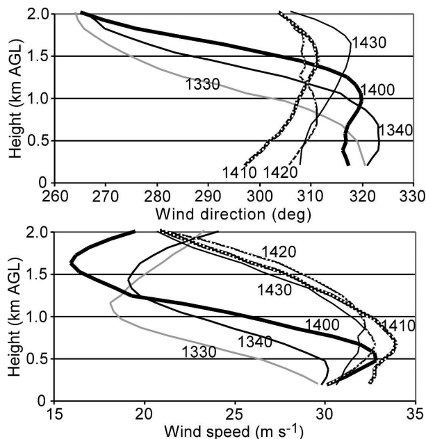
FIG. 15. As in Fig. 13, except for the unstable onshore flow regime along the west side of Gabrielle from 1330 to 1430 UTC.
