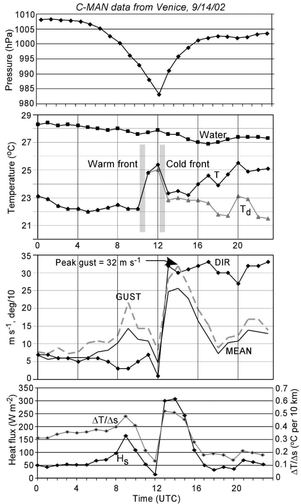
FIG. 8. Time series of recorded and estimated quantities of the Venice (VENF1) C-MAN station, located adjacent to the MIPS. The bottom panel includes surface heat flux ( H_s ), estimated from Eq. (1), and temperature gradient ( \Delta T/\Delta s ) off the west coast based on the value of heat flux and wind speed.
