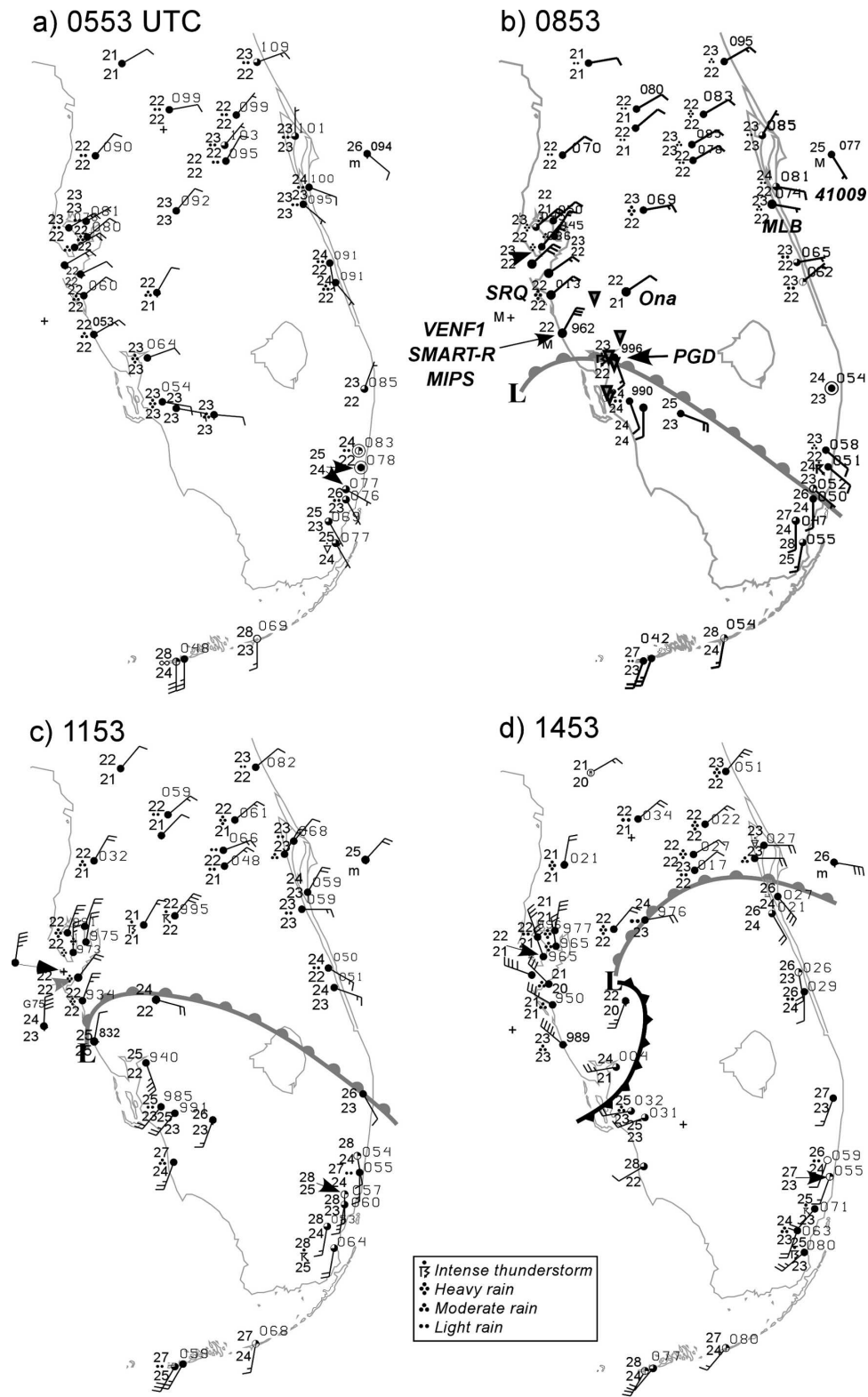
FIG. 6. Surface analyses at (a) 0553, (b) 0853, (c) 1153, and (d) 1453 UTC 14 Sep 2001. Temperature and dewpoint are plotted in ^{\circ}\text{C} ; full wind barbs represent 5\text{ m s}^{-1} . Pressure is coded in the upper right, in units of hPa according to standard convention (e.g., 082 = 1008.2 hPa, 940 = 994.0 hPa). Warm and cold frontal symbols represent boundaries that behave like warm and cold fronts. (b) Surface sites referred to in the text are identified. The MIPS and SMART-R locations are coincident with the Venice C-MAN station (VENF1).
