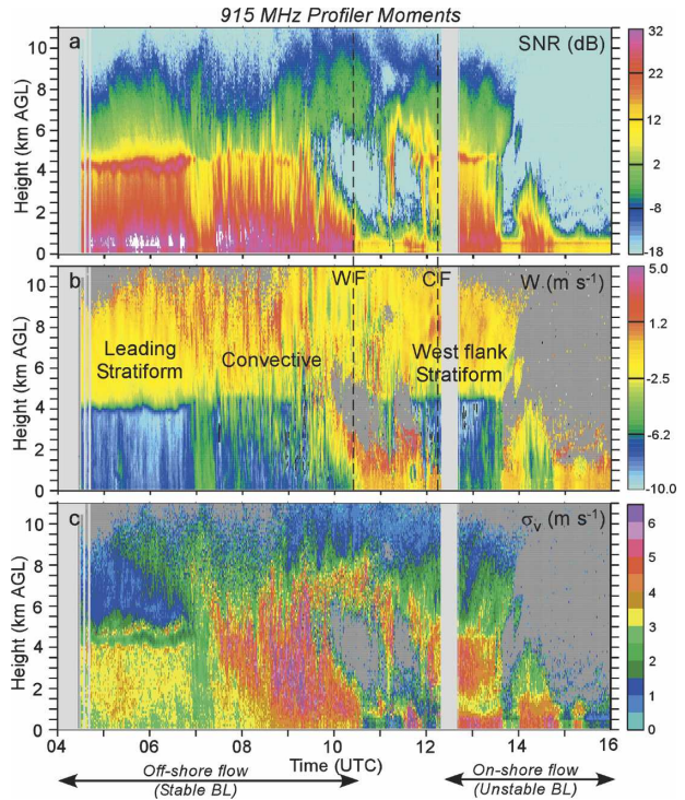
FIG. 4. Time vs height sections of 915 Doppler wind profiler parameters at vertical incidence: (a) signal-to-noise ratio (SNR, dB), (b) total vertical motion, W = w + V_T ( m s^{-1} ), and (c) spectrum width ( m s^{-1} ).
