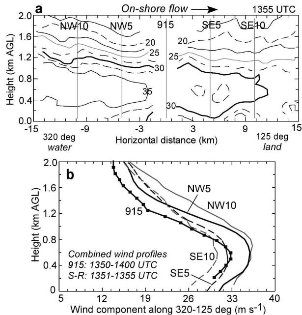
FIG. 16. As in Fig. 14, except for 1355 UTC. (a) The vertical plane is oriented along 320^\circ on the water side, and along 125^\circ on the land side, to follow the mean wind direction as it changes cyclonically from water to land.
