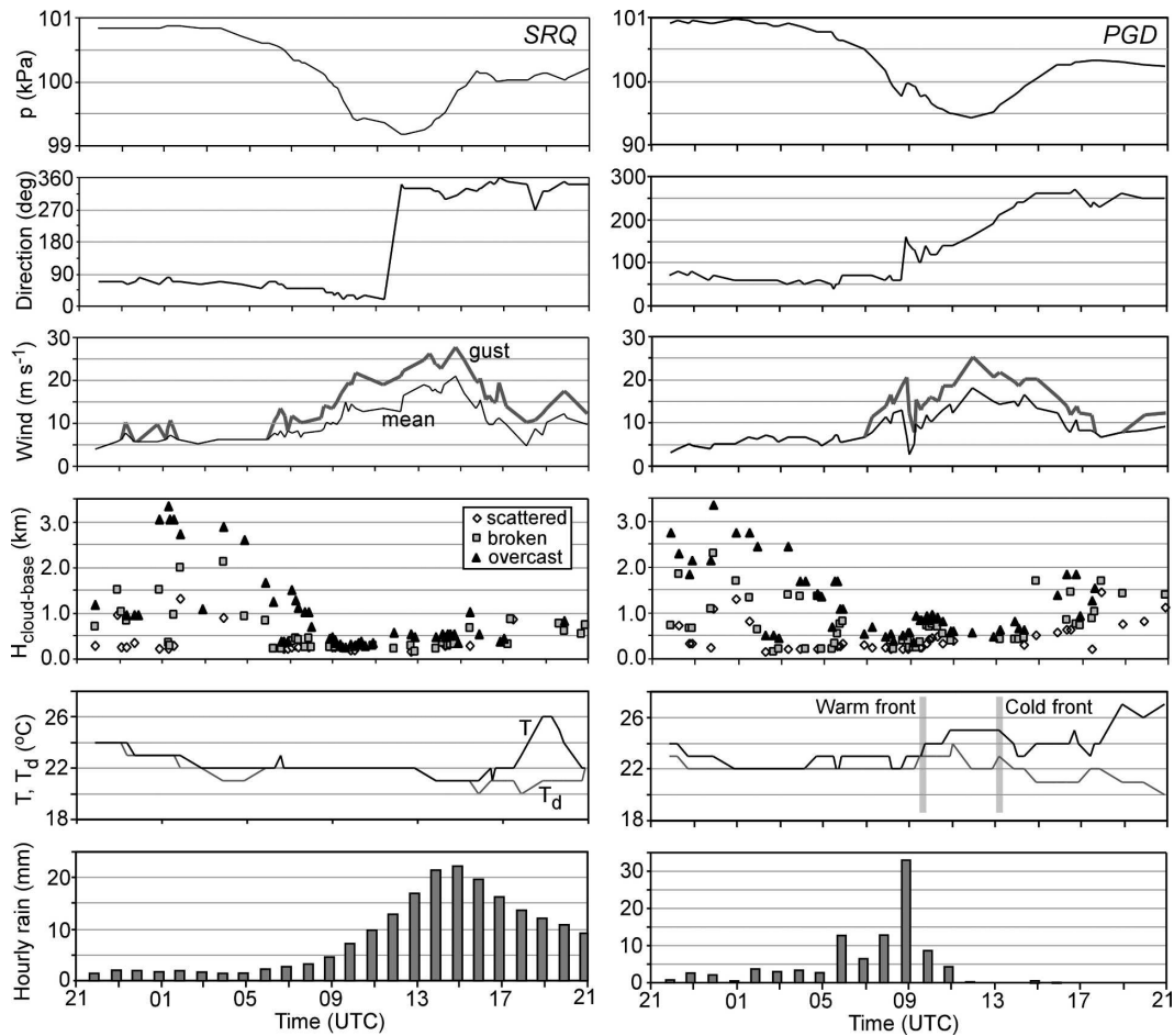
FIG. 10. Time series of surface parameters from ASOS sites located at Sarasota (SRQ) and Punta Gorda (PGD). Locations are shown in Fig. 6b. Rain rate is plotted as an hourly value. All other parameters are plotted for standard hourly plus supplemental observation times.
