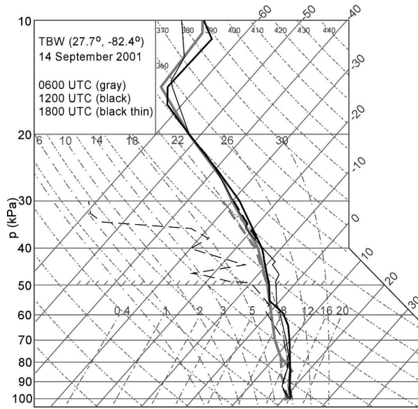
FIG. 3. Soundings from TBW at 0600, 1200, and 1800 UTC, plotted on a skew T -log p diagram. The TBW location is shown in Figs. 1 and 2.
