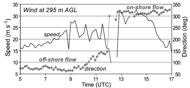
FIG. 12. The 915-MHz profiler wind speed and direction within the boundary layer at 295 m AGL. This time series is derived from contiguous 10-min averages.
