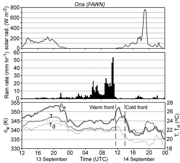
FIG. 7. Time series selected quantities from Ona, whose location is shown in Fig. 6b: (a) solar radiation, (b) rainfall rate, and (c) temperature, dewpoint, and equivalent potential temperature for the 36-h period 1200 UTC 13 Sep to 0000 UTC 15 Sep 2001. Temporal resolution is 15 min.
