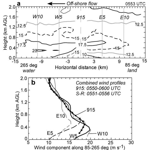
FIG. 14. (a) Isotach analysis of the horizontal velocity component within the vertical plane that passes over the SMART-R and MIPS along the direction 265^\circ\text{--}85^\circ , roughly parallel to the wind direction at 400 m AGL. Contours are labeled in \text{m s}^{-1} . (b) W10, W5, E5, and E10 represent locations of vertical profiles of this wind component. Here, 915 represents the location of the wind component within this plane derived from the MIPS 915-MHz profiler. (b) Vertical profiles of the wind component analyzed in (a). The 915-MHz wind profile represents a 10-min average. All profiles exhibit a jet structure. The jet height progressively increases from water (W, west) to land (E, east).
