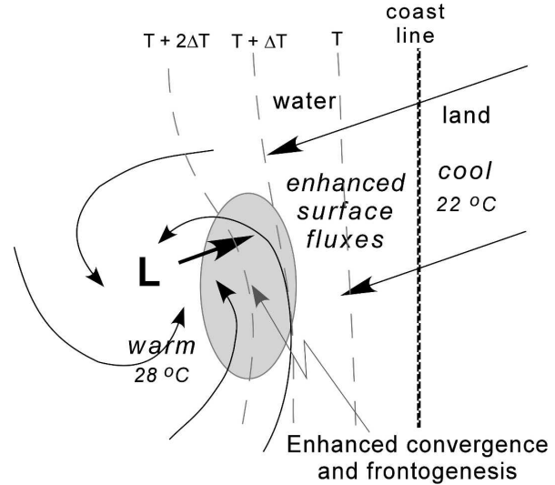
FIG. 9. Schematic showing the basic elements within the boundary layer that promote frontogenesis. These include the source of cool air from land, surface heat fluxes over the water producing a horizontal temperature gradient, and the convergent forward flank of Gabrielle, perhaps enhanced in this case by the east-northeasterly airflow that existed on a scale larger than that of Gabrielle's core cyclonic circulation. Dashed lines are isotherms near the surface.
