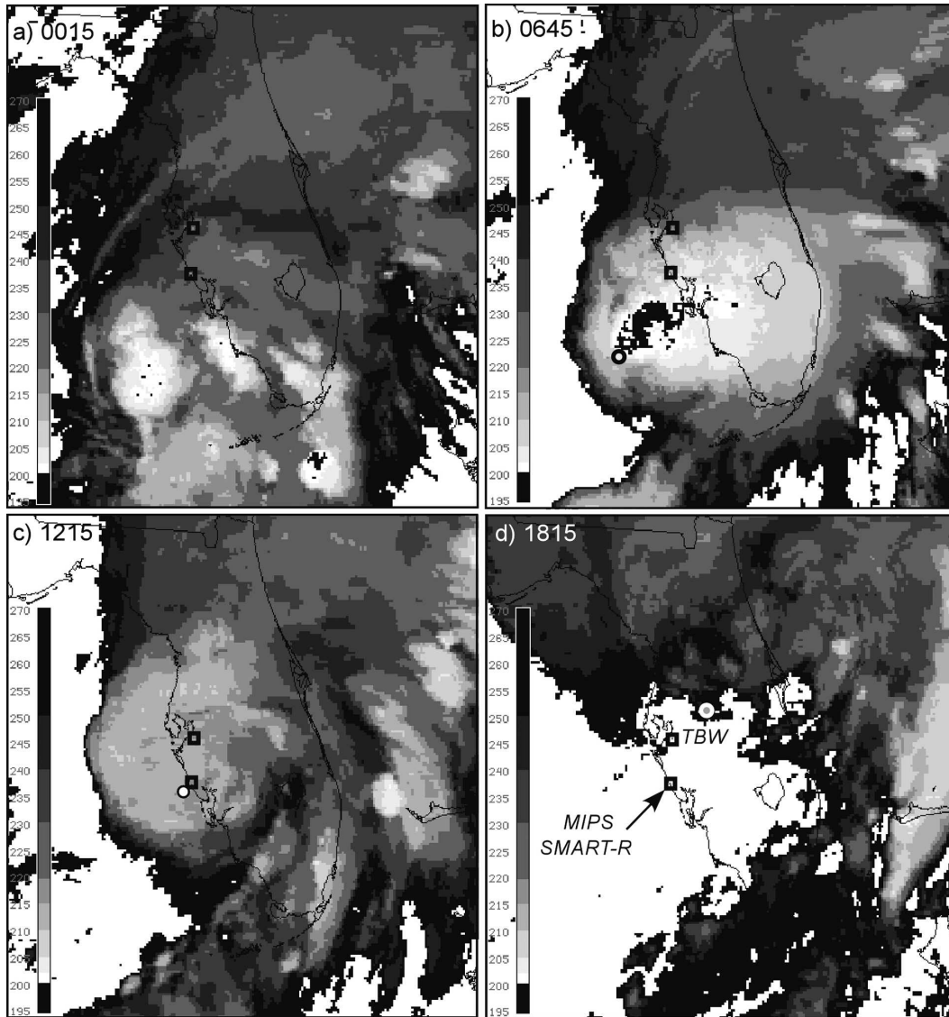
FIG. 1. GOES-enhanced IR imagery at (a) 0015, (b) 0645, (c) 1215, and (d) 1815 UTC 14 Sep 2001. (b)–(d) The approximate location of the wind center is denoted by a filled circle. The grayscale on the left defines brightness temperature (K). Instrument locations are identified in (d). The distance between the TBW WSR-88D and SMART-R radars is 70 km.
