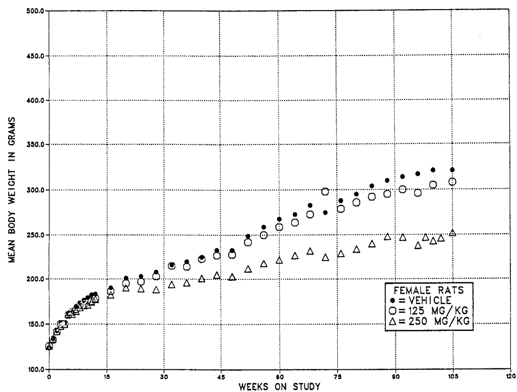
Figure 1. Growth Curves for Rats Administered 1,2-Dichloropropane by Gavage
