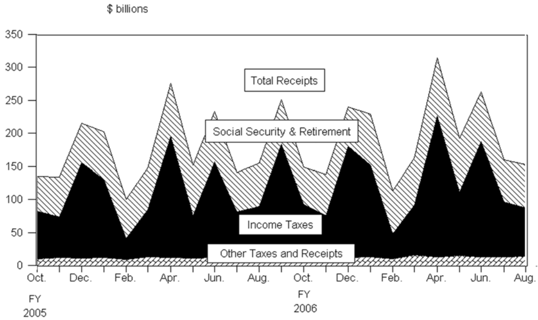
Figure 2. Monthly Receipts of the U.S. Government, by Source, Fiscal Years 2005 and 2006
